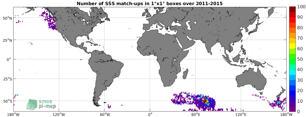
Figure 4: Number of SSS match-ups between Sea mammals SSS and the Aquarius-L2-JPL-V5 SSS product for the SMOS coastal zone (<800km) 60N-60S Pi-MEP region over 1^\circ \times 1^\circ boxes and for the full satellite product period.
