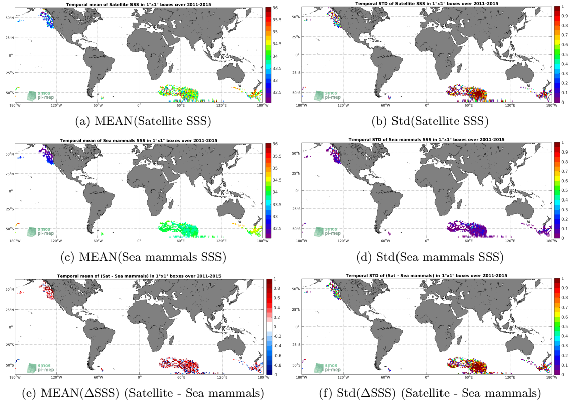
Figure 6: Temporal mean (left) and Std (right) of SSS from Aquarius-L2-JPL-V5 (top), Sea mammals (middle), and of \Delta SSS (Satellite - Sea mammals). Only match-up pairs are used to generate these maps.
