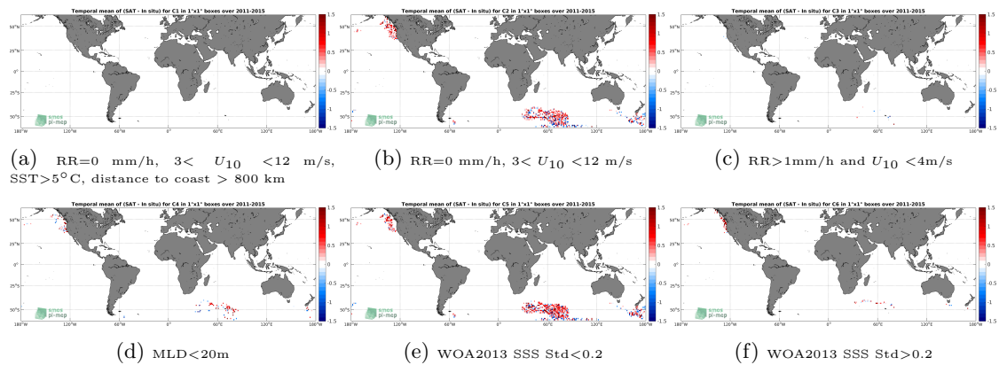
Figure 12: Temporal mean gridded over spatial boxes of size 1^\circ \times 1^\circ of \Delta SSS (Aquarius-L2-JPL-V5 - Sea mammals) for 6 different subdatasets corresponding to:RR=0 mm/h, 3 < U_{10} < 12 m/s, SST > 5^\circ\text{C} , distance to coast > 800 km (a), RR=0 mm/h, 3 < U_{10} < 12 m/s (b), RR > 1 mm/h and U_{10} < 4 m/s (c),MLD < 20 m (d),WOA2013 SSS Std < 0.2 (e),WOA2013 SSS Std > 0.2 (f).
