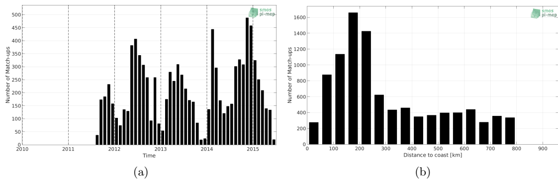
Figure 1: Number of match-ups between Sea mammals and Aquarius-L2-JPL-V5 SSS as a function of time (a) and as function of the distance to coast (b) over the SMOS coastal zone (<800km) 60N-60S Pi-MEP region and for the full satellite product period.
