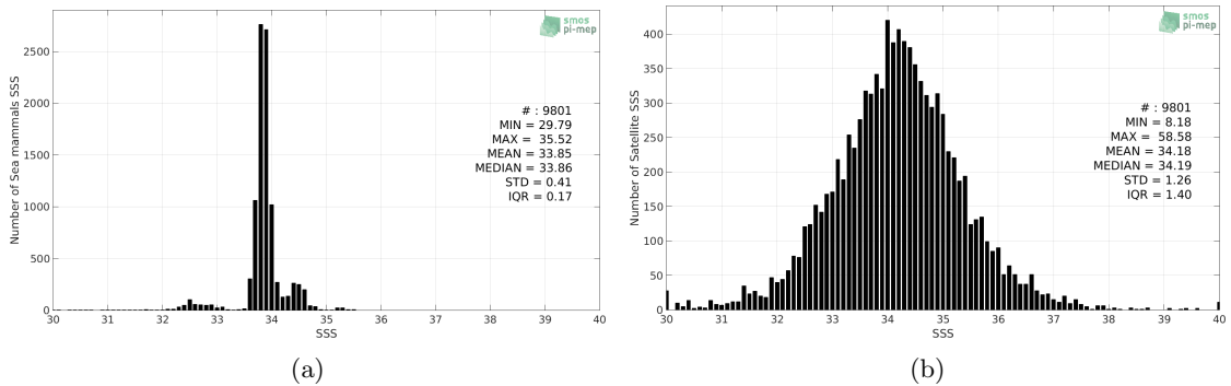
Figure 2: Histograms of SSS from Sea mammals (a) and Aquarius-L2-JPL-V5 (b) considering all match-up pairs per bins of 0.1 over the SMOS coastal zone (<800km) 60N-60S Pi-MEP region and for the full satellite product period.
