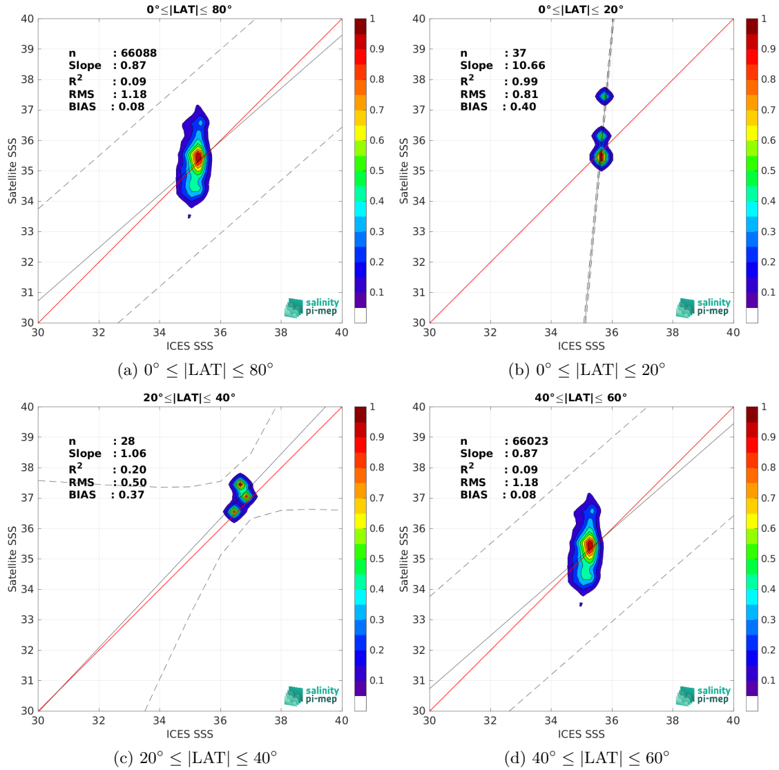
Figure 10: Contour maps of the concentration of Aquarius SSS L2 CAP v5 (JPL) SSS (y-axis) versus ICES SSS (x-axis) at match-up pairs for different latitude bands. For each plot, the red line shows x=y . The black thin and dashed lines indicate a linear fit through the data cloud and the \pm 95\% confidence levels, respectively. The number match-up pairs n , the slope and R^2 coefficient of the linear fit, the root mean square (RMS) and the mean bias between satellite and in situ data are indicated for each latitude band in each plots.
