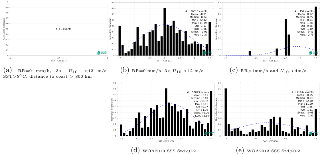
Figure 15: Normalized histogram of \Delta SSS (Aquarius SSS L2 CAP v5 (JPL) - ICES) for 5 different subdatasets corresponding to: RR=0 mm/h, 3 < U_{10} < 12 m/s, SST > 5°C, distance to coast > 800 km (a), RR=0 mm/h, 3 < U_{10} < 12 m/s (b), RR > 1mm/h and U_{10} < 4 m/s (c), WOA2013 SSS Std < 0.2 (d), WOA2013 SSS Std > 0.2 (e).
