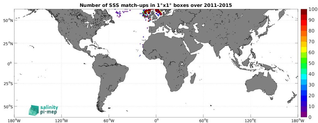
Figure 5: Number of SSS match-ups between ICES SSS and the Aquarius SSS L2 CAP v5 (JPL) SSS product for the SMOS coastal zone (<800km) 60N-60S Pi-MEP region over 1^\circ \times 1^\circ boxes and for the full satellite product period.
