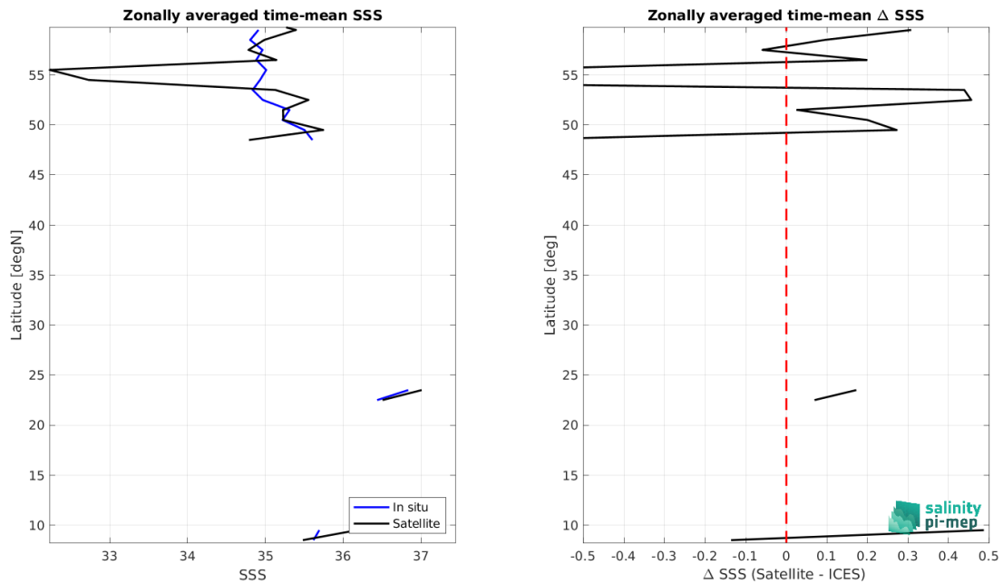
Figure 9: Left panel: Zonal mean SSS from Aquarius SSS L2 CAP v5 (JPL) satellite product (black) and from ICES (blue). Right panel: Zonal mean of \Delta SSS (Satellite - ICES) for all the collected Pi-MEP match-up pairs estimated over the full satellite product period.
