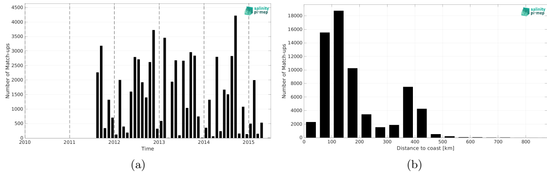
Figure 2: Number of match-ups between ICES and Aquarius SSS L2 CAP v5 (JPL) SSS as a function of time (a) and as function of the distance to coast (b) over the SMOS coastal zone (<800km) 60N-60S Pi-MEP region and for the full satellite product period.
