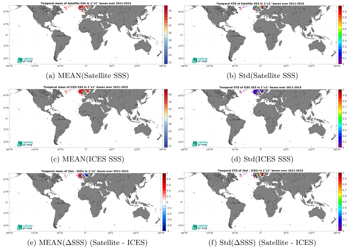
Figure 7: Temporal mean (left) and Std (right) of SSS from Aquarius SSS L2 CAP v5 (JPL) (top), ICES (middle), and of \Delta SSS (Satellite - ICES). Only match-up pairs are used to generate these maps.
