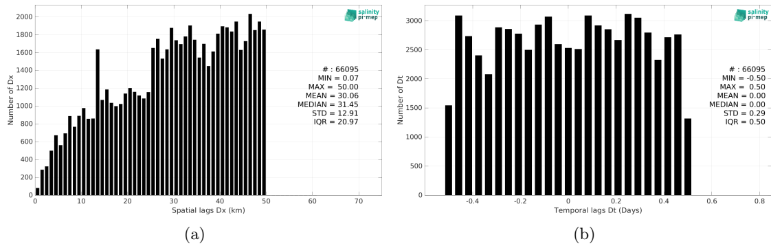
Figure 6: Histograms of the spatial (a) and temporal (b) lags between the location/time of the ICES measurement and the date of the corresponding Aquarius SSS L2 CAP v5 (JPL) SSS pixel.
