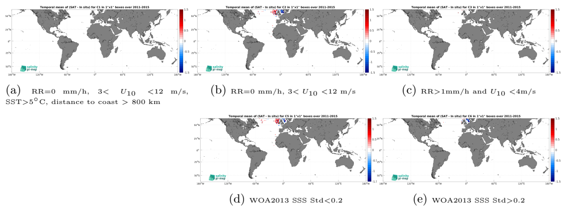
Figure 14: Temporal mean gridded over spatial boxes of size 1^\circ \times 1^\circ of \Delta SSS (Aquarius SSS L2 CAP v5 (JPL) - ICES) for 5 different subdatasets corresponding to:RR=0 mm/h, 3 < U_{10} < 12 m/s, SST >5^\circ C, distance to coast > 800 km (a), RR=0 mm/h, 3 < U_{10} < 12 m/s (b), RR >1 mm/h and U_{10} < 4 m/s (c), WOA2013 SSS Std <0.2 (d), WOA2013 SSS Std >0.2 (e).
