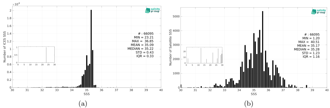
Figure 3: Histograms of SSS from ICES (a) and Aquarius SSS L2 CAP v5 (JPL) (b) considering all match-up pairs per bins of 0.1 over the SMOS coastal zone (<800km) 60N-60S Pi-MEP region and for the full satellite product period.
