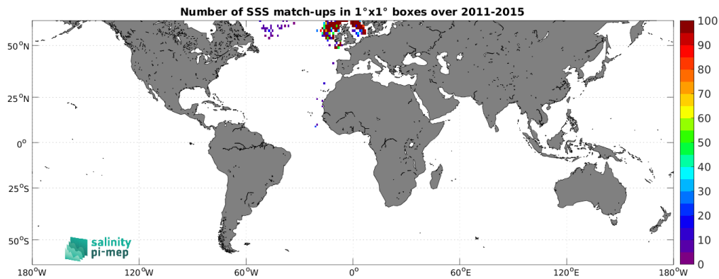
Figure 4: Number of SSS match-ups between ICES SSS and the Aquarius SSS L2 CAP v5 (JPL) SSS product for the SMOS coastal zone (<800km) 60N-60S Pi-MEP region over 1^\circ \times 1^\circ boxes and for the full satellite product period.
