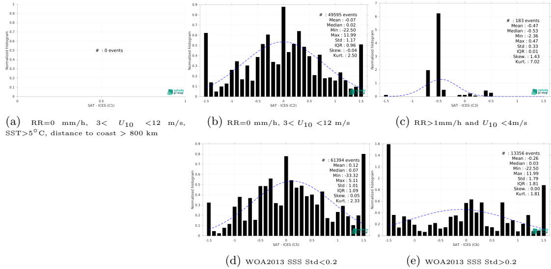
Figure 13: Normalized histogram of \Delta SSS (Aquarius SSS L2 CAP v5 (JPL) - ICES) for 5 different subdatasets corresponding to: RR=0 mm/h, 3 < U_{10} < 12 m/s, SST>5°C, distance to coast > 800 km (a), RR=0 mm/h, 3 < U_{10} < 12 m/s (b), RR>1mm/h and U_{10} < 4 m/s (c), WOA2013 SSS Std<0.2 (d), WOA2013 SSS Std>0.2 (e).
