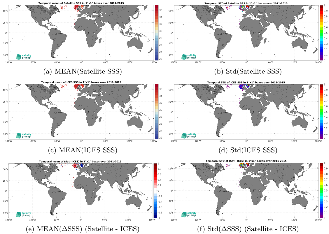
Figure 6: Temporal mean (left) and Std (right) of SSS from Aquarius SSS L2 CAP v5 (JPL) (top), ICES (middle), and of \Delta SSS (Satellite - ICES). Only match-up pairs are used to generate these maps.
