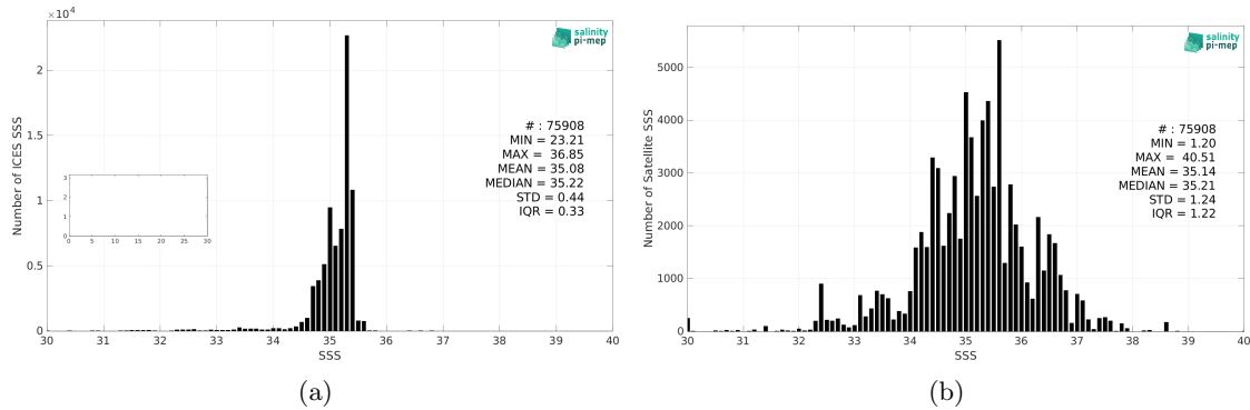
Figure 2: Histograms of SSS from ICES (a) and Aquarius SSS L2 CAP v5 (JPL) (b) considering all match-up pairs per bins of 0.1 over the SMOS coastal zone (<800km) 60N-60S Pi-MEP region and for the full satellite product period.
