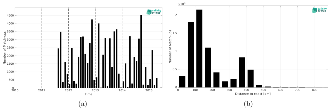
Figure 1: Number of match-ups between ICES and Aquarius SSS L2 CAP v5 (JPL) SSS as a function of time (a) and as function of the distance to coast (b) over the SMOS coastal zone (<800km) 60N-60S Pi-MEP region and for the full satellite product period.
