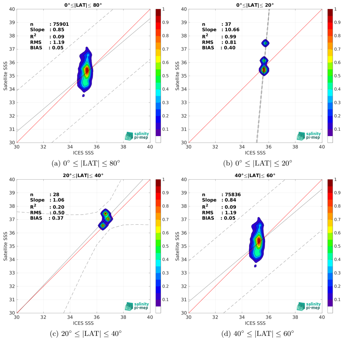
Figure 9: Contour maps of the concentration of Aquarius SSS L2 CAP v5 (JPL) SSS (y-axis) versus ICES SSS (x-axis) at match-up pairs for different latitude bands. For each plot, the red line shows x=y . The black thin and dashed lines indicate a linear fit through the data cloud and the \pm 95\% confidence levels, respectively. The number match-up pairs n , the slope and R^2 coefficient of the linear fit, the root mean square (RMS) and the mean bias between satellite and in situ data are indicated for each latitude band in each plots.
