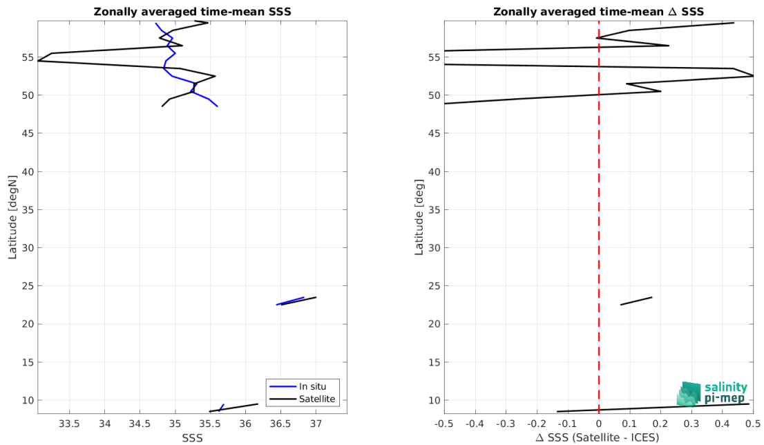
Figure 8: Left panel: Zonal mean SSS from Aquarius SSS L2 CAP v5 (JPL) satellite product (black) and from ICES (blue). Right panel: Zonal mean of \Delta SSS (Satellite - ICES) for all the collected Pi-MEP match-up pairs estimated over the full satellite product period.
