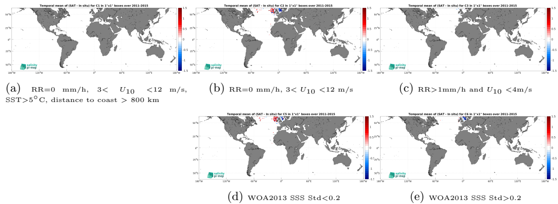
Figure 12: Temporal mean gridded over spatial boxes of size 1^\circ \times 1^\circ of \Delta SSS (Aquarius SSS L2 CAP v5 (JPL) - ICES) for 5 different subdatasets corresponding to:RR=0 mm/h, 3 < U_{10} < 12 m/s, SST >5^\circ\text{C} , distance to coast > 800 km (a), RR=0 mm/h, 3 < U_{10} < 12 m/s (b), RR >1 mm/h and U_{10} < 4 m/s (c), WOA2013 SSS Std <0.2 (d), WOA2013 SSS Std >0.2 (e).
