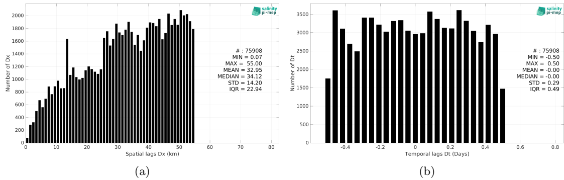
Figure 5: Histograms of the spatial (a) and temporal (b) lags between the location/time of the ICES measurement and the date of the corresponding Aquarius SSS L2 CAP v5 (JPL) SSS pixel.
