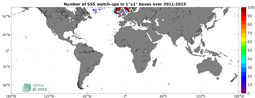
Figure 4: Number of SSS match-ups between ICES SSS and the Aquarius SSS L2 CAP v5 (JPL) SSS product for the SMOS coastal zone (<800km) 60N-60S Pi-MEP region over 1°×1° boxes and for the full satellite product period.
