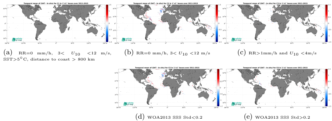
Figure 13: Temporal mean gridded over spatial boxes of size 1^\circ \times 1^\circ of \Delta SSS (Aquarius SSS L2 CAP v5 (JPL) - Surface drifters) for 5 different subdatasets corresponding to:RR=0 mm/h, 3 < U_{10} < 12 m/s, SST >5^\circ C, distance to coast > 800 km (a), RR=0 mm/h, 3 < U_{10} < 12 m/s (b), RR >1 mm/h and U_{10} < 4 m/s (c), WOA2013 SSS Std <0.2 (d), WOA2013 SSS Std >0.2 (e).
