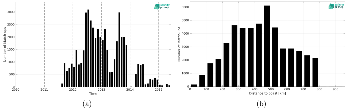
Figure 2: Number of match-ups between Surface drifters and Aquarius SSS L2 CAP v5 (JPL) SSS as a function of time (a) and as function of the distance to coast (b) over the SMOS coastal zone (<800km) 60N-60S Pi-MEP region and for the full satellite product period.
