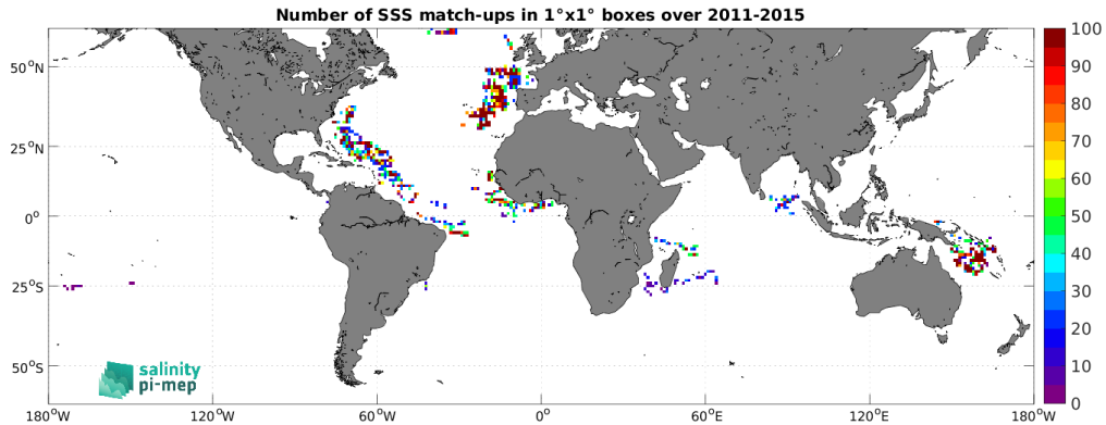
Figure 4: Number of SSS match-ups between Surface drifters SSS and the Aquarius SSS L2 CAP v5 (JPL) SSS product for the SMOS coastal zone (<800km) 60N-60S Pi-MEP region over 1^\circ \times 1^\circ boxes and for the full satellite product period.
