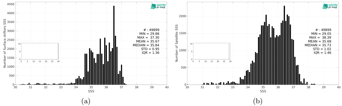
Figure 3: Histograms of SSS from Surface drifters (a) and Aquarius SSS L2 CAP v5 (JPL) (b) considering all match-up pairs per bins of 0.1 over the SMOS coastal zone (<800km) 60N-60S Pi-MEP region and for the full satellite product period.
