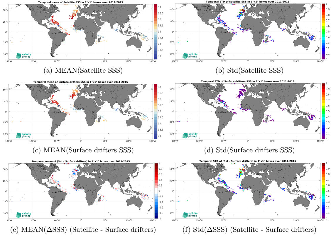
Figure 6: Temporal mean (left) and Std (right) of SSS from Aquarius SSS L2 CAP v5 (JPL) (top), Surface drifters (middle), and of \Delta SSS (Satellite - Surface drifters). Only match-up pairs are used to generate these maps.
