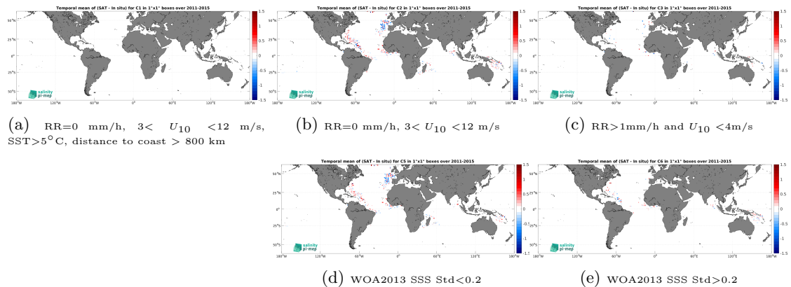
Figure 13: Temporal mean gridded over spatial boxes of size 1^\circ \times 1^\circ of \Delta\text{SSS} (Aquarius SSS L2 CAP v5 (JPL) - Surface drifters) for 5 different subdatasets corresponding to:RR=0 mm/h, 3 < U_{10} < 12 m/s, SST >5^\circ\text{C} , distance to coast > 800 km (a), RR=0 mm/h, 3 < U_{10} < 12 m/s (b), RR >1 mm/h and U_{10} < 4 m/s (c), WOA2013 SSS Std <0.2 (d), WOA2013 SSS Std >0.2 (e).
