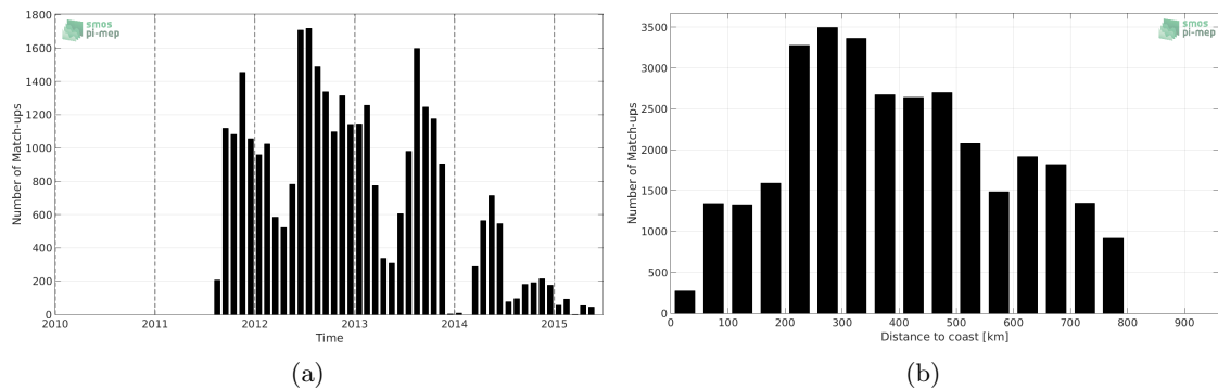
Figure 1: Number of match-ups between Surface drifters and Aquarius-L2-JPL-V5 SSS as a function of time (a) and as function of the distance to coast (b) over the SMOS coastal zone (¡800km) 60N-60S Pi-MEP region and for the full satellite product period.
