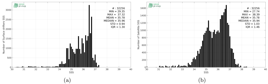
Figure 2: Histograms of SSS from Surface drifters (a) and Aquarius-L2-JPL-V5 (b) considering all match-up pairs per bins of 0.1 over the SMOS coastal zone ( \pm 800\text{km} ) 60N-60S Pi-MEP region and for the full satellite product period.
