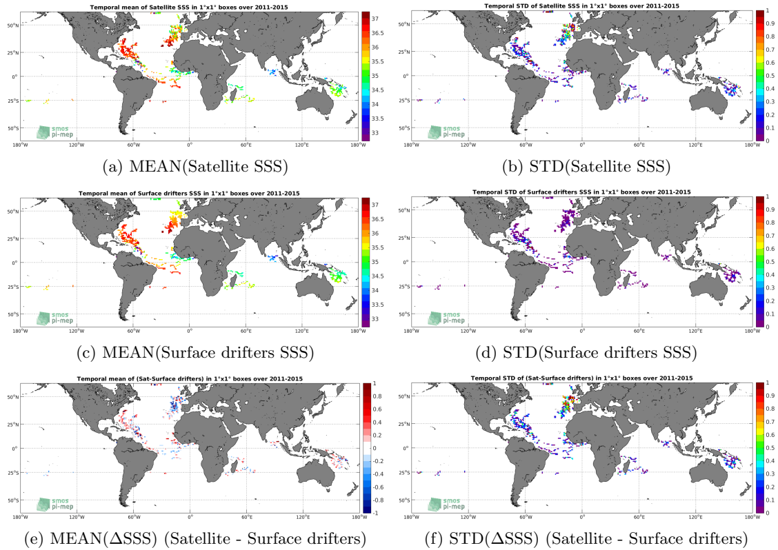
Figure 5: Temporal mean (left) and STD (right) of SSS from Aquarius-L2-JPL-V5 (top), Surface drifters (middle), and of \Delta SSS (Satellite - Surface drifters). Only match-up pairs are used to generate these maps.
