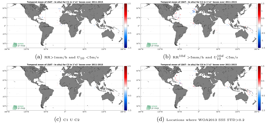
Figure 11: Temporal mean gridded over spatial boxes of size 1^\circ \times 1^\circ of \Delta SSS (Aquarius-L2-JPL-V5 - Surface drifters) for 4 different subdatasets corresponding to: RR > 1\text{mm/h} and U_{10} < 5\text{m/s} (a), RR^{10d} > 5\text{mm/h} and U_{10}^{10d} < 5\text{m/s} (b), C1 U C2 (c), Locations where WOA2013 SSS STD > 0.2 (d).
