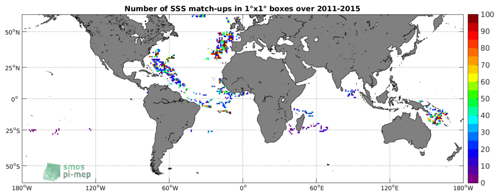
Figure 3: Number of SSS match-ups between Surface drifters SSS and the Aquarius-L2-JPL-V5 SSS product for the SMOS coastal zone ( \pm 800\text{km} ) 60N-60S Pi-MEP region over 1^\circ \times 1^\circ boxes and for the full satellite product period.
