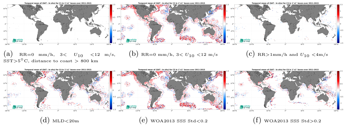
Figure 14: Temporal mean gridded over spatial boxes of size 1^\circ \times 1^\circ of \Delta\text{SSS} (Aquarius SSS L2 CAP v5 (JPL) - Argo) for 6 different subdatasets corresponding to: RR=0 mm/h, 3 < U_{10} < 12 m/s, SST > 5°C, distance to coast > 800 km (a), RR=0 mm/h, 3 < U_{10} < 12 m/s (b), RR > 1mm/h and U_{10} < 4 m/s (c), MLD < 20m (d), WOA2013 SSS Std < 0.2 (e), WOA2013 SSS Std > 0.2 (f).
