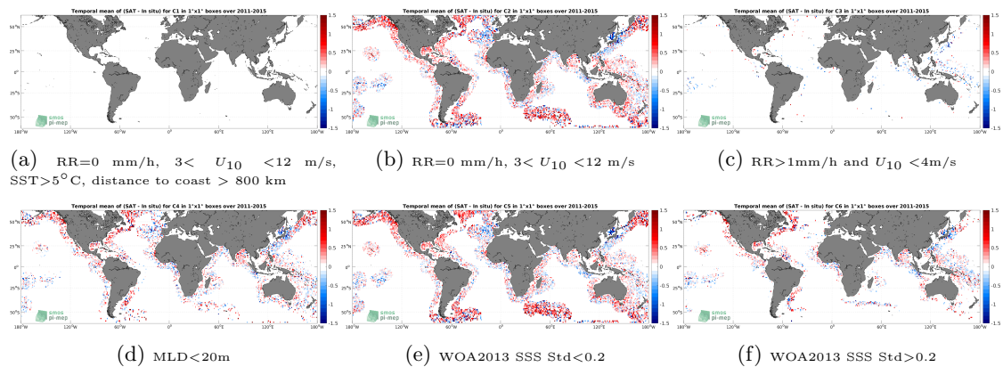
Figure 12: Temporal mean gridded over spatial boxes of size 1^\circ \times 1^\circ of \Delta SSS (Aquarius SSS L2 CAP v5 (JPL) - Argo) for 6 different subdatasets corresponding to:RR=0 mm/h, 3 < U_{10} < 12 m/s, SST >5^\circ C, distance to coast > 800 km (a), RR=0 mm/h, 3 < U_{10} < 12 m/s (b), RR >1 mm/h and U_{10} < 4 m/s (c),MLD <20 m (d),WOA2013 SSS Std <0.2 (e),WOA2013 SSS Std >0.2 (f).
