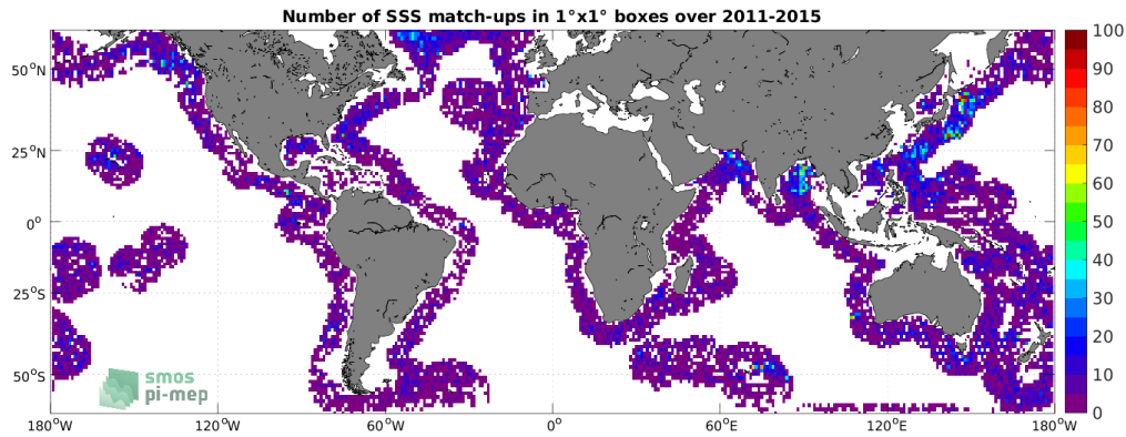
Figure 4: Number of SSS match-ups between Argo SSS and the Aquarius SSS L2 CAP v5 (JPL) SSS product for the SMOS coastal zone (<800km) 60N-60S Pi-MEP region over 1^\circ \times 1^\circ boxes and for the full satellite product period.
