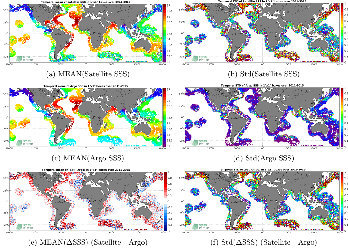
Figure 6: Temporal mean (left) and Std (right) of SSS from Aquarius SSS L2 CAP v5 (JPL) (top), Argo (middle), and of \Delta SSS (Satellite - Argo). Only match-up pairs are used to generate these maps.
