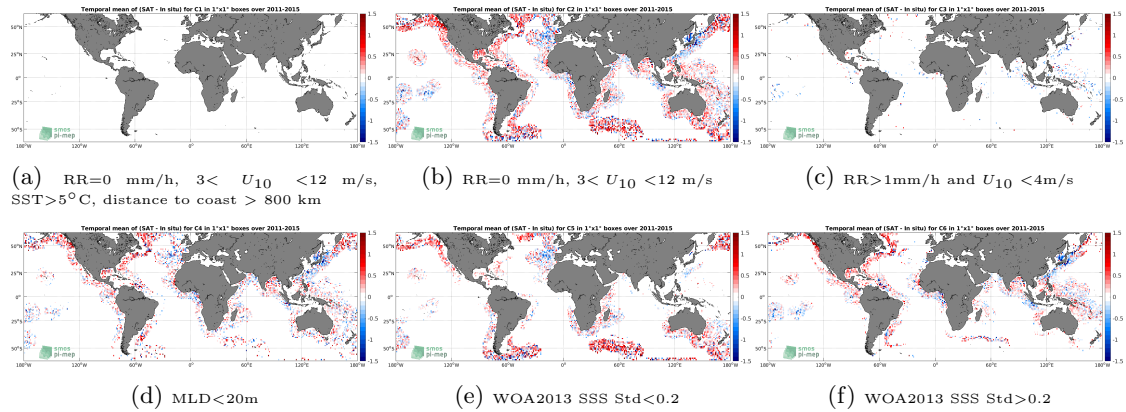
Figure 12: Temporal mean gridded over spatial boxes of size 1^\circ \times 1^\circ of \Delta SSS (Aquarius SSS L2 CAP v5 (JPL) - Argo) for 6 different subdatasets corresponding to: RR=0 mm/h, 3 < U_{10} < 12 m/s, SST > 5°C, distance to coast > 800 km (a), RR=0 mm/h, 3 < U_{10} < 12 m/s (b), RR > 1mm/h and U_{10} < 4 m/s (c), MLD < 20m (d), WOA2013 SSS Std < 0.2 (e), WOA2013 SSS Std > 0.2 (f).
