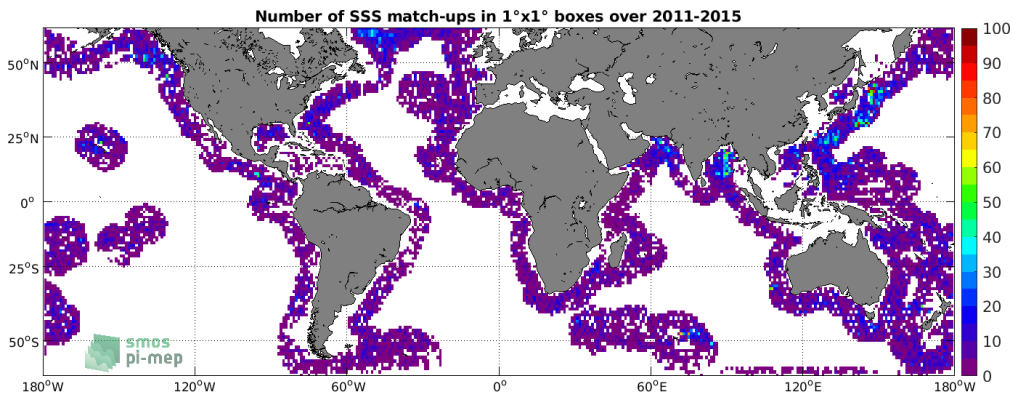
Figure 4: Number of SSS match-ups between Argo SSS and the Aquarius SSS L2 CAP v5 (JPL) SSS product for the SMOS coastal zone (<800km) 60N-60S Pi-MEP region over 1°×1° boxes and for the full satellite product period.
