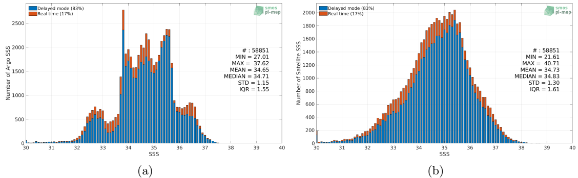
Figure 2: Histograms of SSS from Argo (a) and Aquarius SSS L2 CAP v5 (JPL) (b) considering all match-up pairs per bins of 0.1 over the SMOS coastal zone (<800km) 60N-60S Pi-MEP region and for the full satellite product period.
