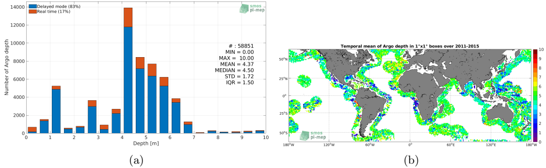
Figure 3: Histograms of the depth of the upper level SSS measurements from Argo in the Match-up DataBase for the SMOS coastal zone (<800km) 60N-60S Pi-MEP region (a) and temporal mean spatial distribution of pressure of the in situ SSS data over 1°×1° boxes and for the full satellite product period (b).
