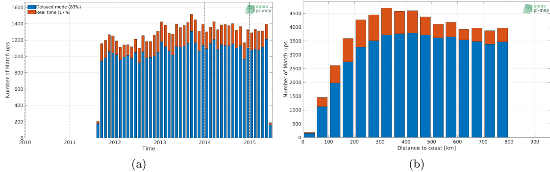
Figure 1: Number of match-ups between Argo and Aquarius SSS L2 CAP v5 (JPL) SSS as a function of time (a) and as function of the distance to coast (b) over the SMOS coastal zone (<800km) 60N-60S Pi-MEP region and for the full satellite product period.
