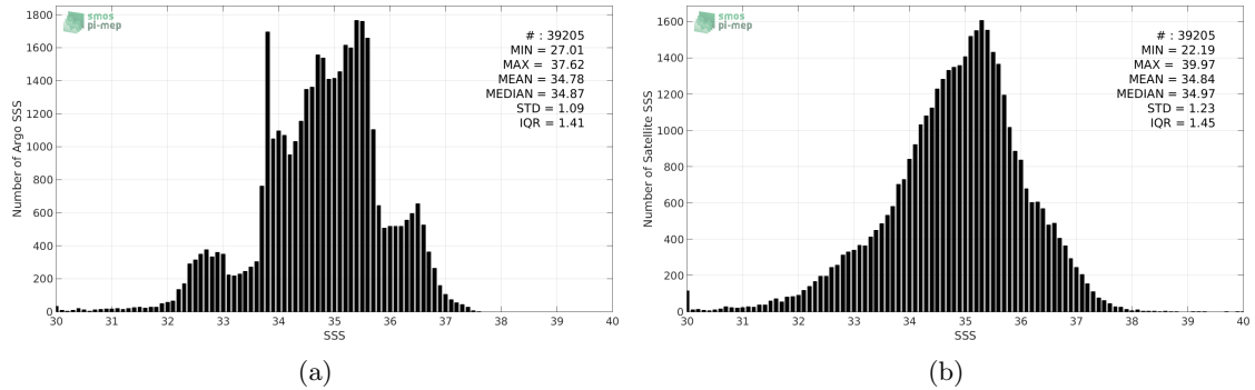
Figure 2: Histograms of SSS from Argo (a) and Aquarius-L2-JPL-V5 (b) considering all match-up pairs per bins of 0.1 over the SMOS coastal zone ( \approx 800\text{km} ) 60N-60S Pi-MEP region and for the full satellite product period.
