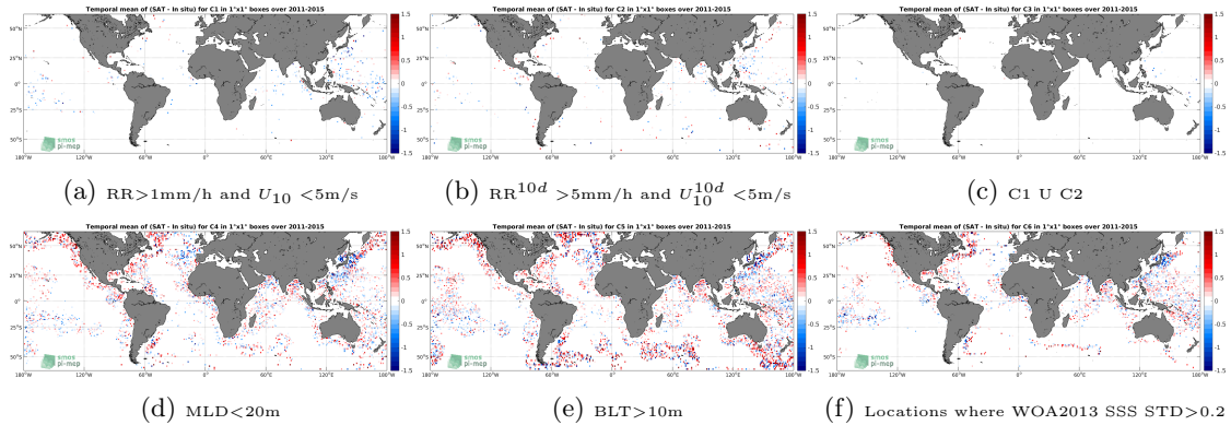
Figure 12: Temporal mean gridded over spatial boxes of size 1^\circ \times 1^\circ of \Delta\text{SSS} (Aquarius-L2-JPL-V5 - Argo) for 6 different subdatasets corresponding to: RR > 1\text{mm/h} and U_{10} < 5\text{m/s} (a), RR^{10d} > 5\text{mm/h} and U_{10}^{10d} < 5\text{m/s} (b), C1 U C2 (c), MLD < 20\text{m} (d), BLT > 10\text{m} (e), Locations where WOA2013 SSS STD > 0.2 (f).
