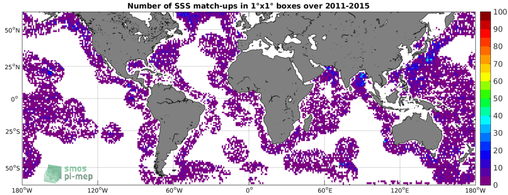
Figure 4: Number of SSS match-ups between Argo SSS and the Aquarius-L2-JPL-V5 SSS product for the SMOS coastal zone ( \geq 800\text{km} ) 60N-60S Pi-MEP region over 1^\circ \times 1^\circ boxes and for the full satellite product period.
