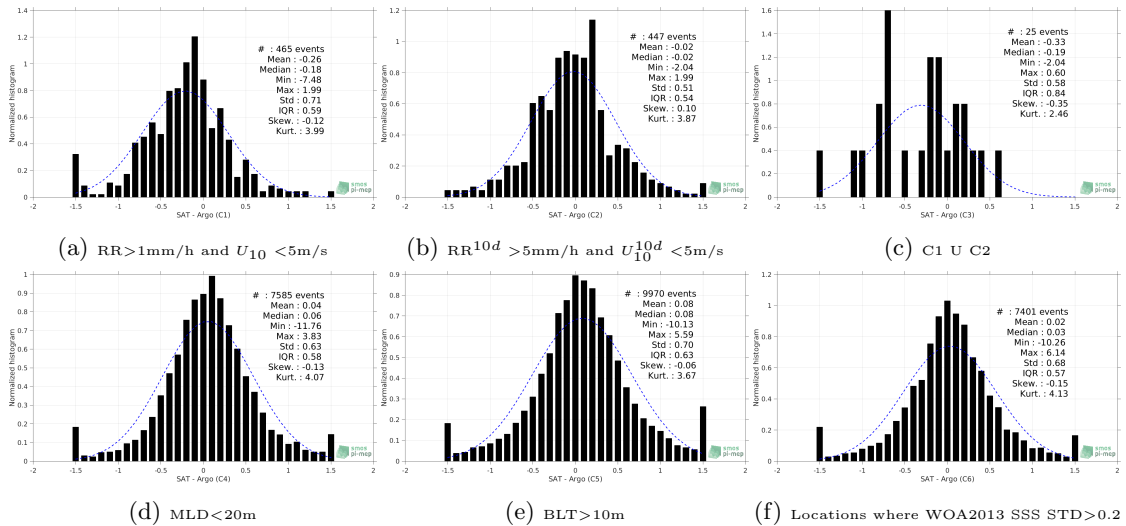
Figure 13: Normalized histogram of \Delta\text{SSS} (Aquarius-L2-JPL-V5 - Argo) for 6 different subdatasets corresponding to: RR > 1\text{mm/h} and U_{10} < 5\text{m/s} (a), RR^{10d} > 5\text{mm/h} and U_{10}^{10d} < 5\text{m/s} (b), C1 U C2 (c), MLD < 20\text{m} (d), BLT > 10\text{m} (e), Locations where WOA2013 SSS STD > 0.2 (f).
