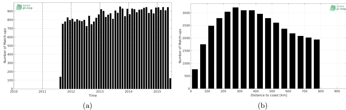
Figure 1: Number of match-ups between Argo and Aquarius-L2-JPL-V5 SSS as a function of time (a) and as function of the distance to coast (b) over the SMOS coastal zone ( \pm 800 km) 60N-60S Pi-MEP region and for the full satellite product period.
