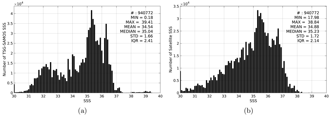
Figure 2: Histograms of SSS from TSG-SAMOS (a) and AQUARIUS-L2-JPL-V4 (b) considering all match-up pairs per bins of 0.1 over the SMOS coastal zone ( \pm 800\text{km} ) 60N-60S Pi-MEP region and for the full satellite product period.
