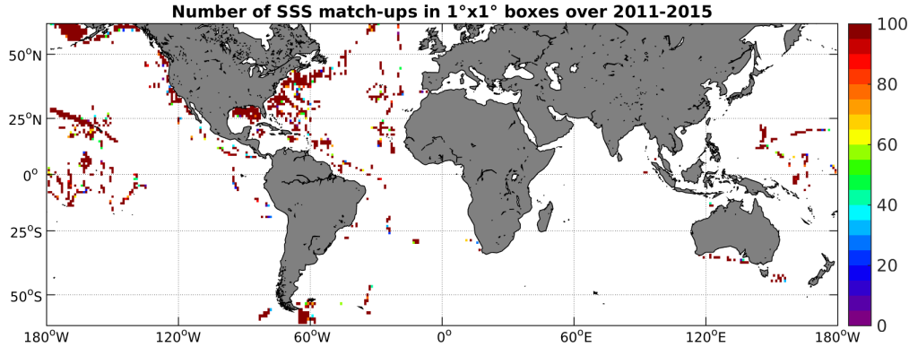
Figure 4: Number of SSS match-ups between TSG-SAMOS SSS and the AQUARIUS-L2-JPL-V4 SSS product for the SMOS coastal zone ( \leq 800\text{km} ) 60N-60S Pi-MEP region over 1^\circ \times 1^\circ boxes and for the full satellite product period.
