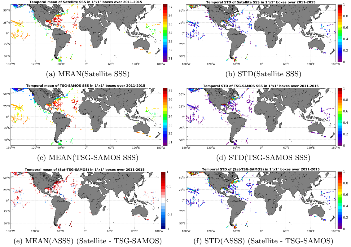
Figure 6: Temporal mean (left) and STD (right) of SSS from AQUARIUS-L2-JPL-V4 (top), TSG-SAMOS (middle), and of \Delta SSS (Satellite - TSG-SAMOS). Only match-up pairs are used to generate these maps.
