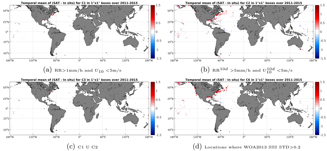
Figure 12: Temporal mean gridded over spatial boxes of size 1^\circ \times 1^\circ of \Delta SSS (AQUARIUS-L2-JPL-V4 - TSG-SAMOS) for 4 different subdatasets corresponding to: RR > 1\text{mm/h} and U_{10} < 5\text{m/s} (a), RR^{10d} > 5\text{mm/h} and U_{10}^{10d} < 5\text{m/s} (b), C1 U C2 (c), Locations where WOA2013 SSS STD > 0.2 (d).
