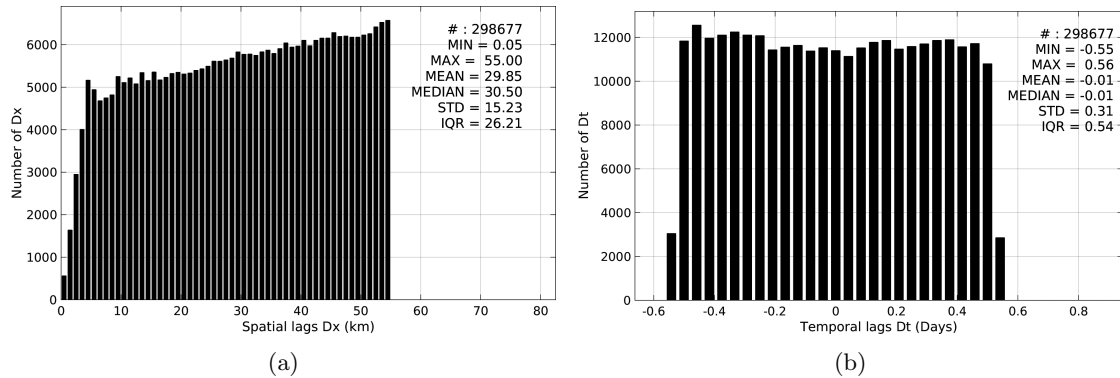
Figure 5: Histograms of the spatial (a) and temporal (b) lags between the time of the TSG-LEGOS-DM measurements and the date of the corresponding AQUARIUS-L2-JPL-V4 SSS product.
