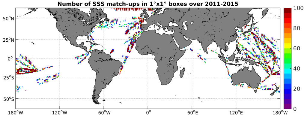
Figure 4: Number of SSS match-ups between TSG-LEGOS-DM SSS and the AQUARIUS-L2-JPL-V4 SSS product for the SMOS coastal zone ( \pm 800\text{km} ) 60N-60S Pi-MEP region over 1^\circ \times 1^\circ boxes and for the full satellite product period.
