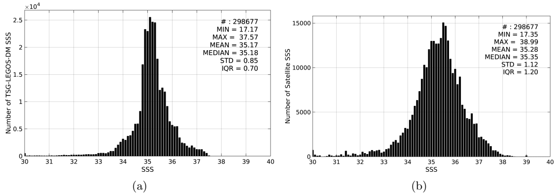
Figure 2: Histograms of SSS from TSG-LEGOS-DM (a) and AQUARIUS-L2-JPL-V4 (b) considering all match-up pairs per bins of 0.1 over the SMOS coastal zone ( \pm 800\text{km} ) 60N-60S Pi-MEP region and for the full satellite product period.
