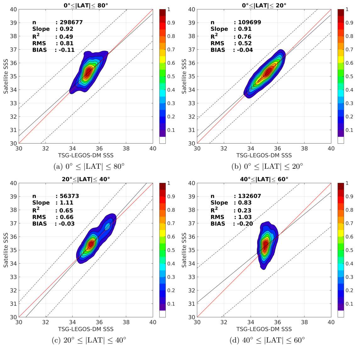
Figure 9: Contour maps of the concentration of AQUARIUS-L2-JPL-V4 SSS (y-axis) versus TSG-LEGOS-DM SSS (x-axis) at match-up pairs for different latitude bands. For each plot, the red line shows x=y . The black thin and dashed lines indicate a linear fit through the data cloud and the \pm 95\% confidence levels, respectively. The number match-up pairs n , the slope and R^2 coefficient of the linear fit, the root mean square (RMS) and the mean bias between satellite and in situ data are indicated for each latitude band in each plots.
