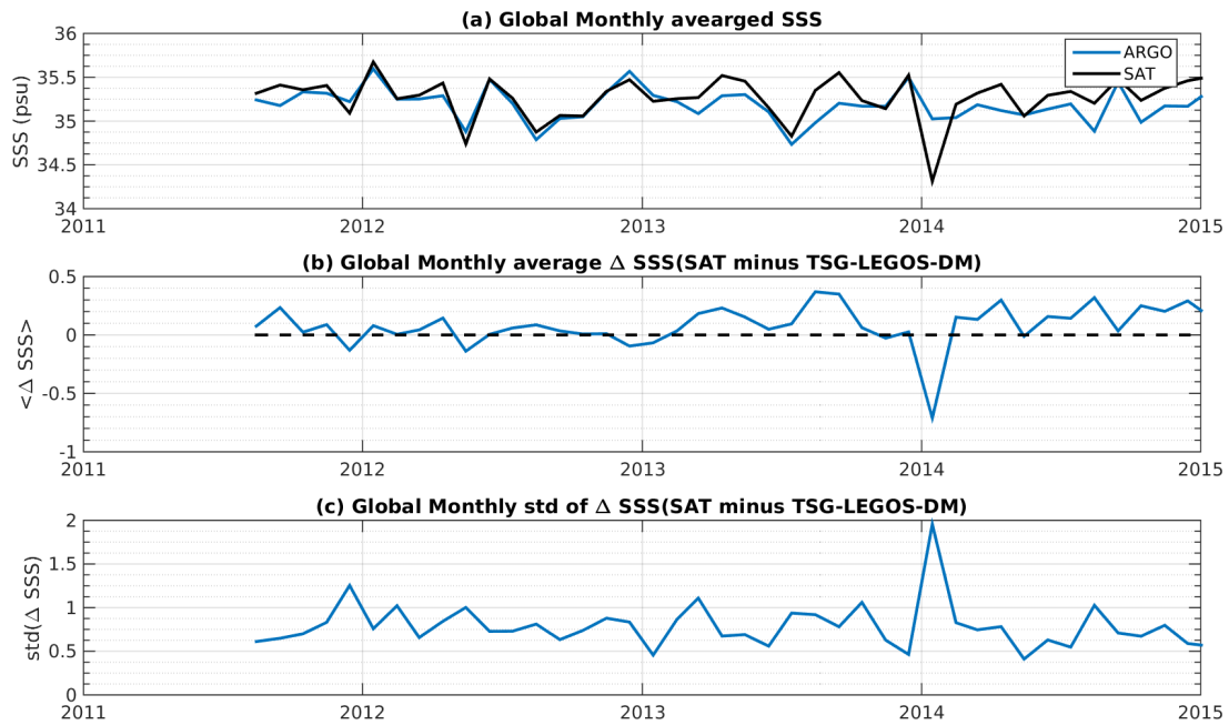
Figure 7: Time series of the monthly averaged mean SSS (top), mean \Delta SSS (Satellite - TSG-LEGOS-DM) and STD of \Delta SSS (Satellite - TSG-LEGOS-DM) over the SMOS coastal zone ( \approx 800 km) 60N-60S Pi-MEP region considering all match-ups collected by the Pi-MEP platform.
