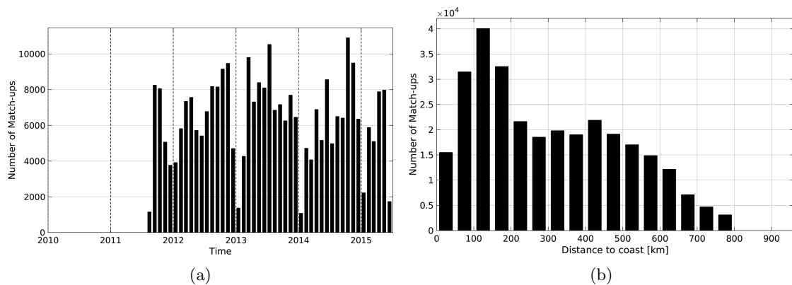
Figure 1: Number of match-ups between TSG-LEGOS-DM and AQUARIUS-L2-JPL-V4 SSS as a function of time (a) and as function of the distance to coast (b) over the SMOS coastal zone ( \pm 800 km) 60N-60S Pi-MEP region and for the full satellite product period.
