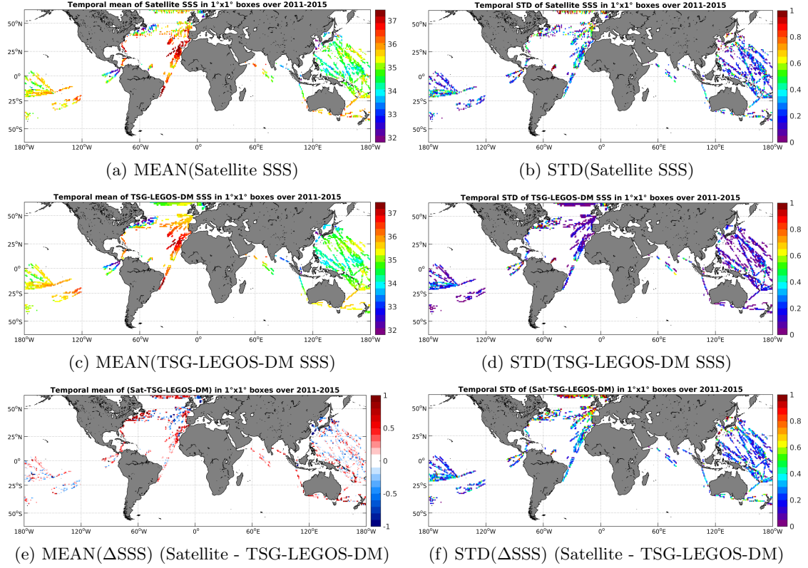
Figure 6: Temporal mean (left) and STD (right) of SSS from AQUARIUS-L2-JPL-V4 (top), TSG-LEGOS-DM (middle), and of \Delta SSS (Satellite - TSG-LEGOS-DM). Only match-up pairs are used to generate these maps.
