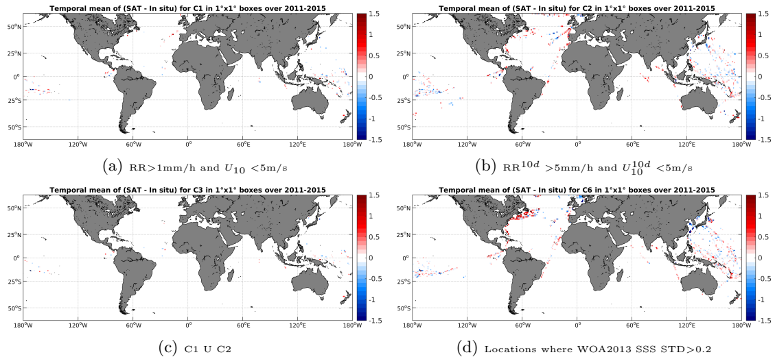
Figure 12: Temporal mean gridded over spatial boxes of size 1^\circ \times 1^\circ of \Delta SSS (AQUARIUS-L2-JPL-V4 - TSG-LEGOS-DM) for 4 different subdatasets corresponding to: RR > 1\text{mm/h} and U_{10} < 5\text{m/s} (a), RR^{10d} > 5\text{mm/h} and U_{10}^{10d} < 5\text{m/s} (b), C1 U C2 (c), Locations where WOA2013 SSS STD > 0.2 (d).
