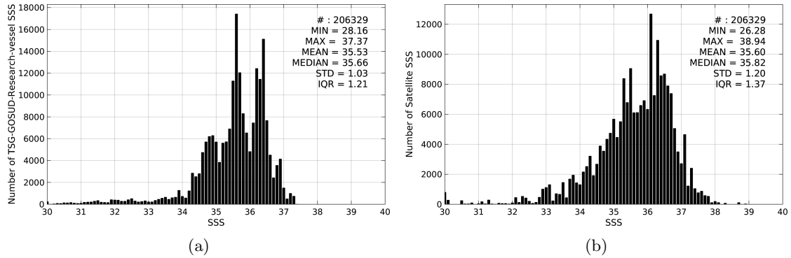
Figure 2: Histograms of SSS from TSG-GOSUD-Research-vessel (a) and AQUARIUS-L2-JPL-V4 (b) considering all match-up pairs per bins of 0.1 over the SMOS coastal zone ( \leq 800 km) 60N-60S Pi-MEP region and for the full satellite product period.
