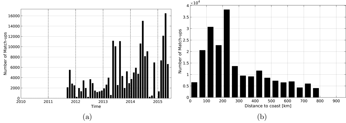
Figure 1: Number of match-ups between TSG-GOSUD-Research-vessel and AQUARIUS-L2-JPL-V4 SSS as a function of time (a) and as function of the distance to coast (b) over the SMOS coastal zone ( \leq 800 km) 60N-60S Pi-MEP region and for the full satellite product period.
