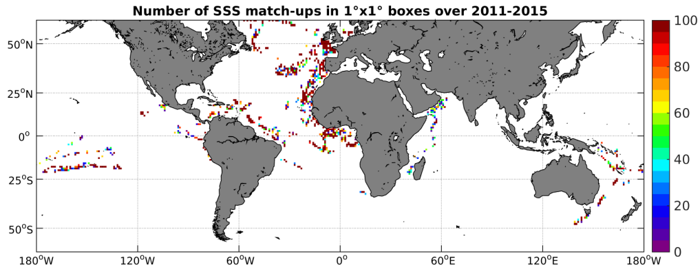
Figure 4: Number of SSS match-ups between TSG-GOSUD-Research-vessel SSS and the AQUARIUS-L2-JPL-V4 SSS product for the SMOS coastal zone ( \pm 800\text{km} ) 60^\circ\text{N} - 60^\circ\text{S} Pi-MEP region over 1^\circ \times 1^\circ boxes and for the full satellite product period.
