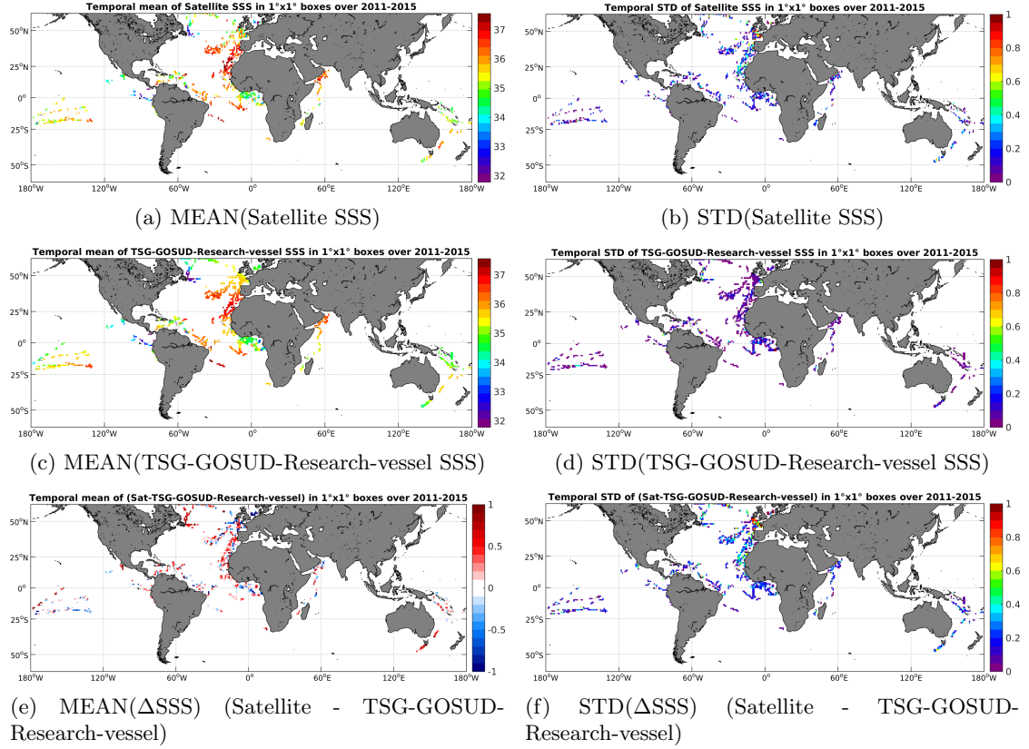
Figure 6: Temporal mean (left) and STD (right) of SSS from AQUARIUS-L2-JPL-V4 (top), TSG-GOSUD-Research-vessel (middle), and of \Delta SSS (Satellite - TSG-GOSUD-Research-vessel). Only match-up pairs are used to generate these maps.
