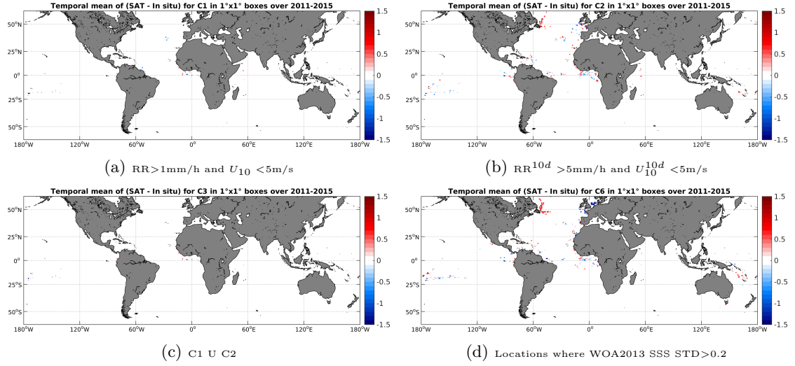
Figure 12: Temporal mean gridded over spatial boxes of size 1^\circ \times 1^\circ of \Delta SSS (AQUARIUS-L2-JPL-V4 - TSG-GOSUD-Research-vessel) for 4 different subdatasets corresponding to: RR > 1\text{mm/h} and U_{10} < 5\text{m/s} (a), RR^{10d} > 5\text{mm/h} and U_{10}^{10d} < 5\text{m/s} (b), C1 U C2 (c), Locations where WOA2013 SSS STD > 0.2 (d).
