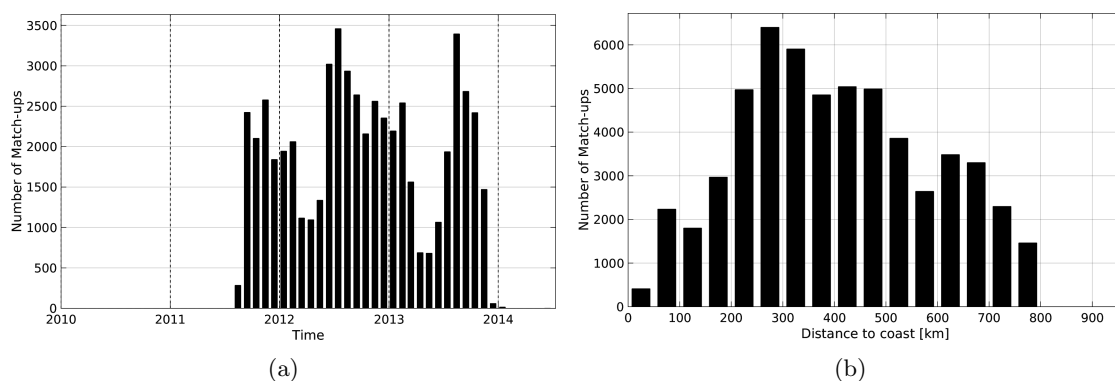
Figure 1: Number of match-ups between Surface drifters and AQUARIUS-L2-JPL-V4 SSS as a function of time (a) and as function of the distance to coast (b) over the SMOS coastal zone (<800km) 60N-60S Pi-MEP region and for the full satellite product period.
