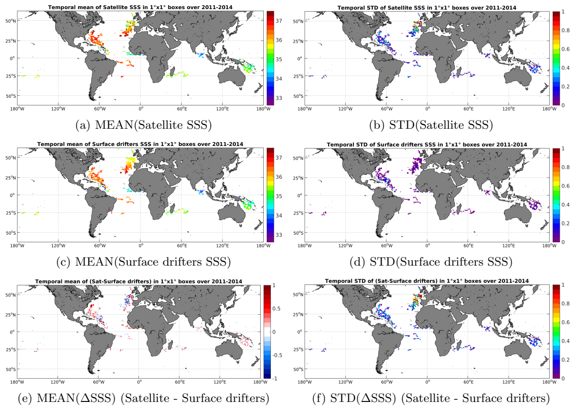
Figure 5: Temporal mean (left) and STD (right) of SSS from AQUARIUS-L2-JPL-V4 (top), Surface drifters (middle), and of \Delta SSS (Satellite - Surface drifters). Only match-up pairs are used to generate these maps.
