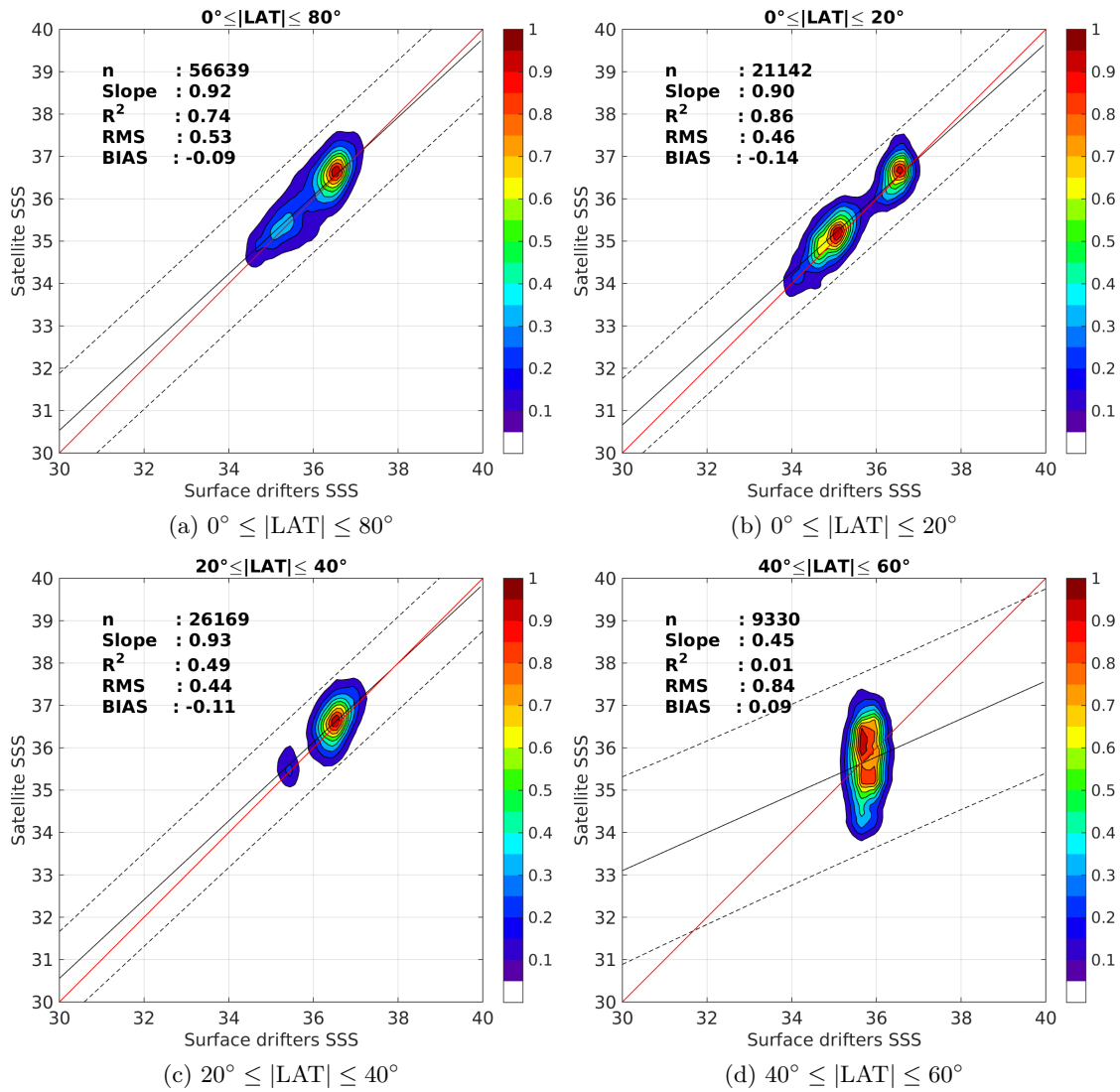
Figure 8: Contour maps of the concentration of AQUARIUS-L2-JPL-V4 SSS (y-axis) versus Surface drifters SSS (x-axis) at match-up pairs for different latitude bands. For each plot, the red line shows x=y . The black thin and dashed lines indicate a linear fit through the data cloud and the \pm 95\% confidence levels, respectively. The number match-up pairs n , the slope and R^2 coefficient of the linear fit, the root mean square (RMS) and the mean bias between satellite and in situ data are indicated for each latitude band in each plots.
