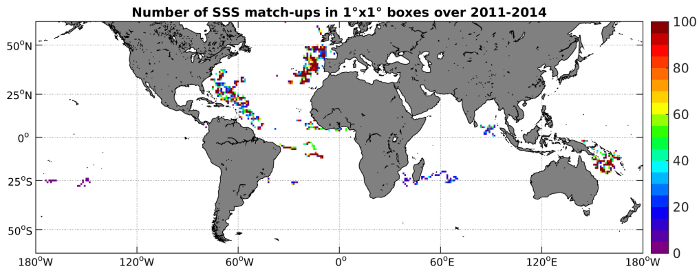
Figure 3: Number of SSS match-ups between Surface drifters SSS and the AQUARIUS-L2-JPL-V4 SSS product for the SMOS coastal zone ( \pm 800\text{km} ) 60N-60S Pi-MEP region over 1^\circ \times 1^\circ boxes and for the full satellite product period.
