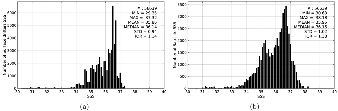
Figure 2: Histograms of SSS from Surface drifters (a) and AQUARIUS-L2-JPL-V4 (b) considering all match-up pairs per bins of 0.1 over the SMOS coastal zone ( \pm 800\text{km} ) 60N-60S Pi-MEP region and for the full satellite product period.
