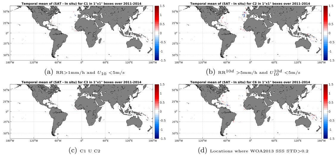
Figure 11: Temporal mean gridded over spatial boxes of size 1°x1° of \Delta SSS (AQUARIUS-L2-JPL-V4 - Surface drifters) for 4 different subdatasets corresponding to: RR > 1\text{mm/h} and U_{10} < 5\text{m/s} (a), RR^{10d} > 5\text{mm/h} and U_{10}^{10d} < 5\text{m/s} (b), C1 U C2 (c), Locations where WOA2013 SSS STD > 0.2 (d).
