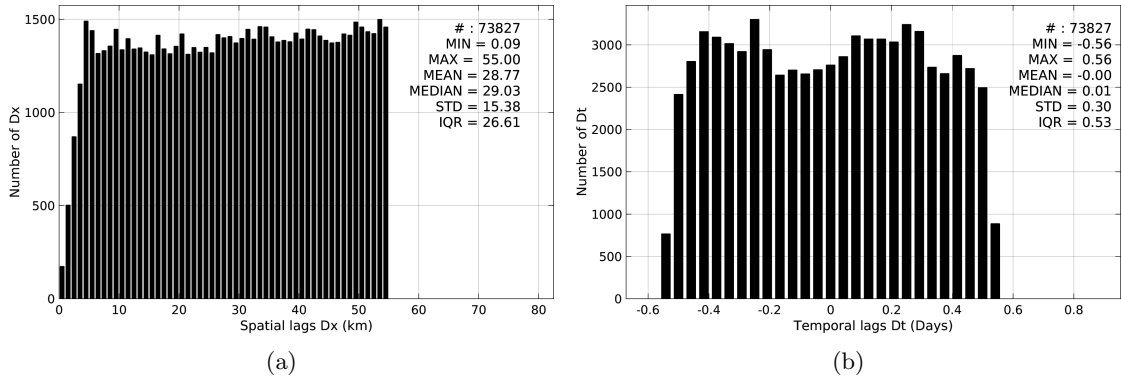
Figure 5: Histograms of the spatial (a) and temporal (b) lags between the time of the Argo measurements and the date of the corresponding AQUARIUS-L2-JPL-V4 SSS product.
