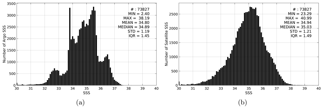
Figure 2: Histograms of SSS from Argo (a) and AQUARIUS-L2-JPL-V4 (b) considering all match-up pairs per bins of 0.1 over the SMOS coastal zone ( \approx 800\text{km} ) 60N-60S Pi-MEP region and for the full satellite product period.
