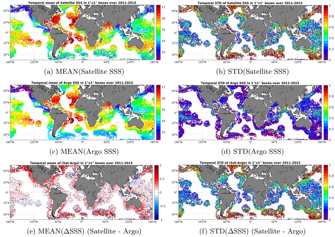
Figure 6: Temporal mean (left) and STD (right) of SSS from AQUARIUS-L2-JPL-V4 (top), Argo (middle), and of \Delta SSS (Satellite - Argo). Only match-up pairs are used to generate these maps.
