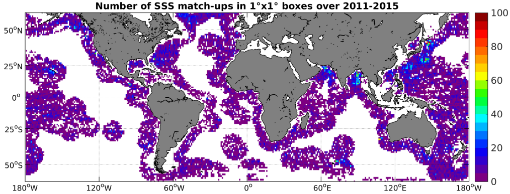
Figure 4: Number of SSS match-ups between Argo SSS and the AQUARIUS-L2-JPL-V4 SSS product for the SMOS coastal zone ( \geq 800\text{km} ) 60N-60S Pi-MEP region over 1^\circ \times 1^\circ boxes and for the full satellite product period.
