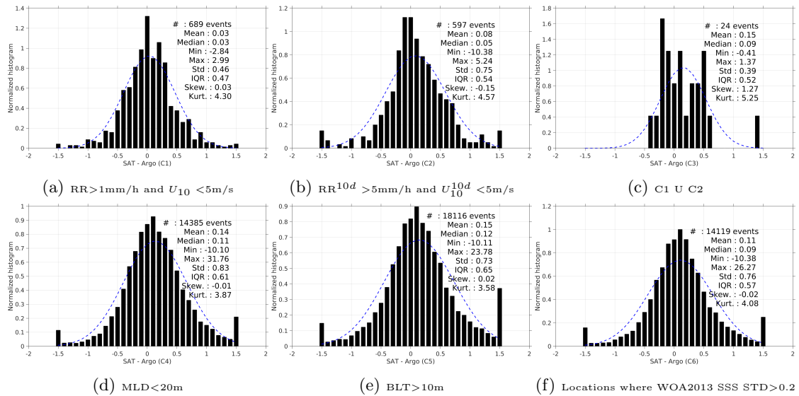
Figure 13: Normalized histogram of \Delta\text{SSS} (AQUARIUS-L2-JPL-V4 - Argo) for 6 different subdatasets corresponding to: \text{RR}>1\text{mm/h} and U_{10} <5\text{m/s} (a), \text{RR}^{10d} >5\text{mm/h} and U_{10}^{10d} <5\text{m/s} (b), C1 U C2 (c), \text{MLD}<20\text{m} (d), \text{BLT}>10\text{m} (e), Locations where WOA2013 SSS \text{STD}>0.2 (f).
