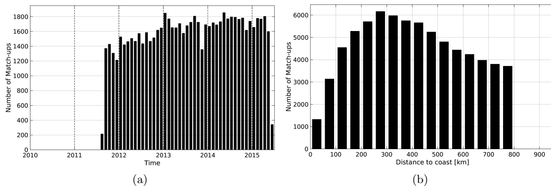
Figure 1: Number of match-ups between Argo and AQUARIUS-L2-JPL-V4 SSS as a function of time (a) and as function of the distance to coast (b) over the SMOS coastal zone ( \leq 800 km) 60N-60S Pi-MEP region and for the full satellite product period.
