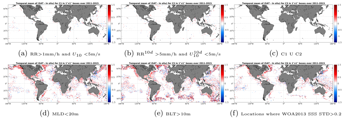
Figure 12: Temporal mean gridded over spatial boxes of size 1^\circ \times 1^\circ of \Delta\text{SSS} (AQUARIUS-L2-JPL-V4 - Argo) for 6 different subdatasets corresponding to: \text{RR}>1\text{mm/h} and U_{10} <5\text{m/s} (a), \text{RR}^{10d} >5\text{mm/h} and U_{10}^{10d} <5\text{m/s} (b), C1 U C2 (c), \text{MLD}<20\text{m} (d), \text{BLT}>10\text{m} (e), Locations where WOA2013 SSS \text{STD}>0.2 (f).
