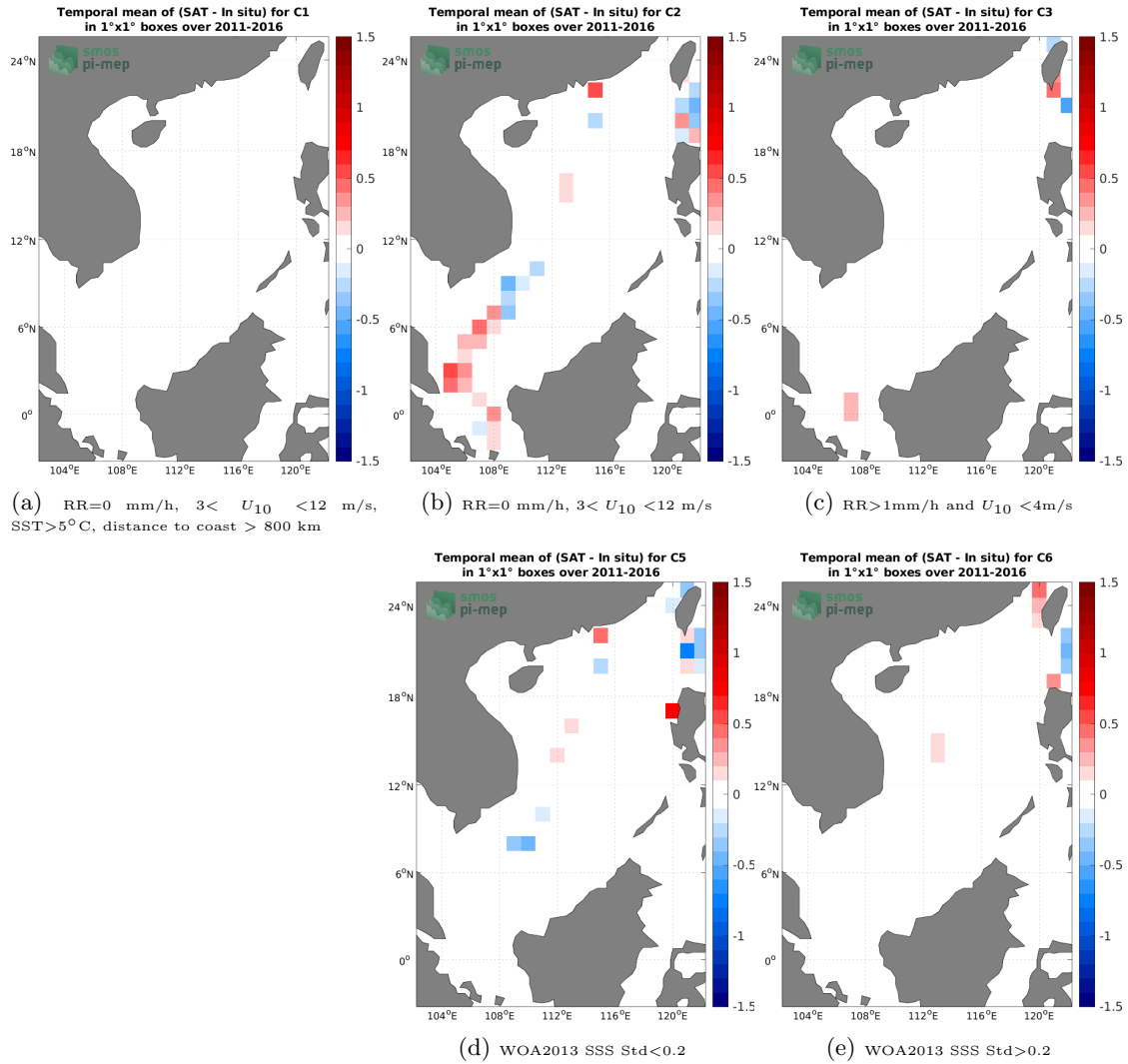
Figure 12: Temporal mean gridded over spatial boxes of size 1^\circ \times 1^\circ of \Delta SSS (SMOS and SMAP SSS L4 OI v1 - 7 Days (LOPS) - TSG (LEGOS-DM)) for 5 different subdatasets corresponding to: RR=0 mm/h, 3 < U_{10} < 12 m/s, SST>5°C, distance to coast > 800 km (a), RR=0 mm/h, 3 < U_{10} < 12 m/s (b), RR>1mm/h and U_{10} < 4 m/s (c), WOA2013 SSS Std<0.2 (d), WOA2013 SSS Std>0.2 (e).
