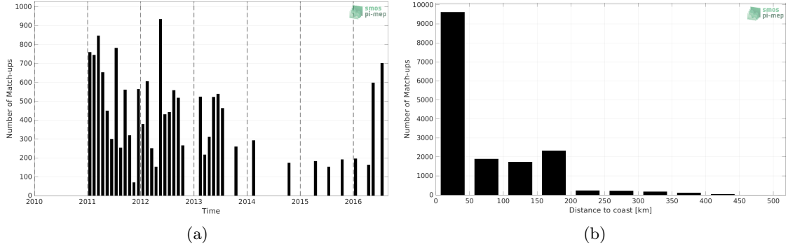
Figure 1: Number of match-ups between TSG (LEGOS-DM) and SMOS and SMAP SSS L4 OI v1 - 7 Days (LOPS) SSS as a function of time (a) and as function of the distance to coast (b) over the South China Sea Pi-MEP region and for the full satellite product period.
