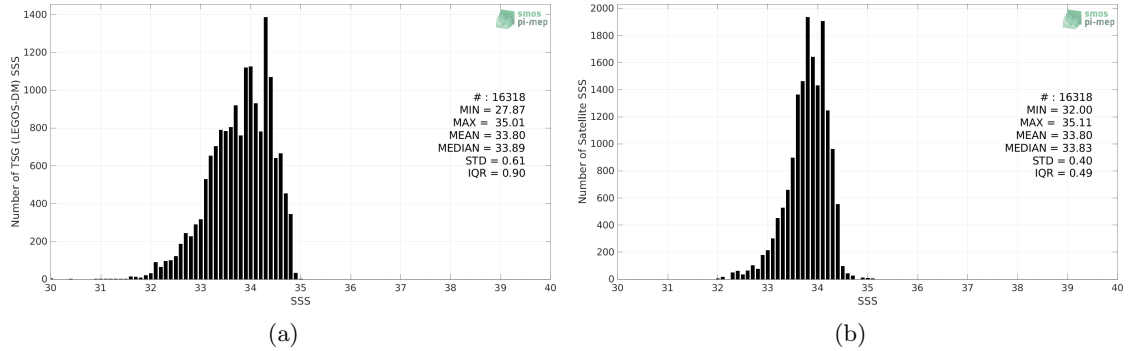
Figure 2: Histograms of SSS from TSG (LEGOS-DM) (a) and SMOS and SMAP SSS L4 OI v1 - 7 Days (LOPS) (b) considering all match-up pairs per bins of 0.1 over the South China Sea Pi-MEP region and for the full satellite product period.
