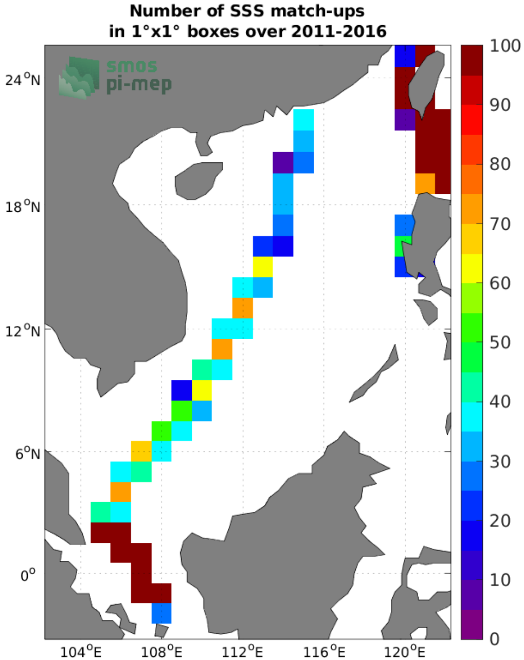
Figure 4: Number of SSS match-ups between TSG (LEGOS-DM) SSS and the SMOS and SMAP SSS L4 OI v1 - 7 Days (LOPS) SSS product for the South China Sea Pi-MEP region over 1°x1° boxes and for the full satellite product period.
