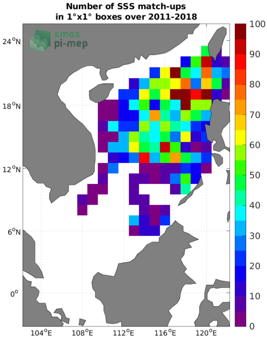
Figure 4: Number of SSS match-ups between Argo SSS and the SMOS and SMAP SSS L4 OI v1 - 7 Days (LOPS) SSS product for the South China Sea Pi-MEP region over 1°x1° boxes and for the full satellite product period.
