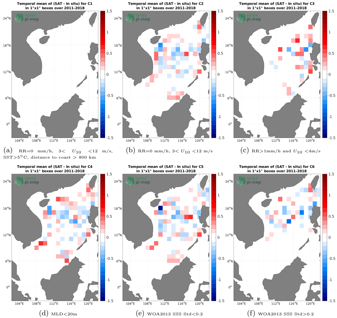
Figure 12: Temporal mean gridded over spatial boxes of size 1^\circ \times 1^\circ of \Delta SSS (SMOS and SMAP SSS L4 OI v1 - 7 Days (LOPS) - Argo) for 6 different subdatasets corresponding to:RR=0 mm/h, 3 < U_{10} < 12 m/s, SST>5°C, distance to coast > 800 km (a), RR=0 mm/h, 3 < U_{10} < 12 m/s (b), RR>1mm/h and U_{10} < 4 m/s (c),MLD<20m (d),WOA2013 SSS Std<0.2 (e),WOA2013 SSS Std>0.2 (f).
