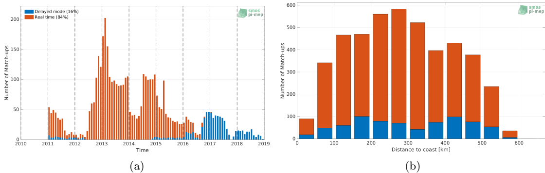
Figure 1: Number of match-ups between Argo and SMOS and SMAP SSS L4 OI v1 - 7 Days (LOPS) SSS as a function of time (a) and as function of the distance to coast (b) over the South China Sea Pi-MEP region and for the full satellite product period.
