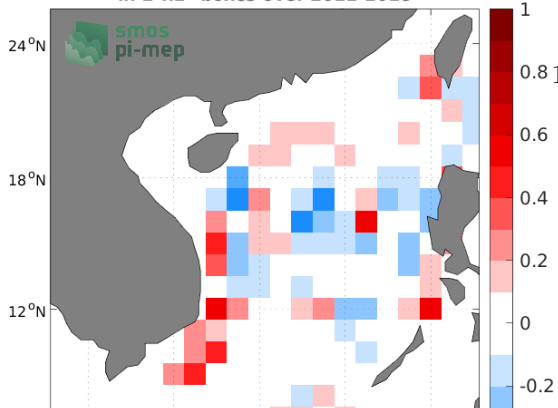
Temporal mean of (Sat - Argo) in 1°x1° boxes over 2011-2018
