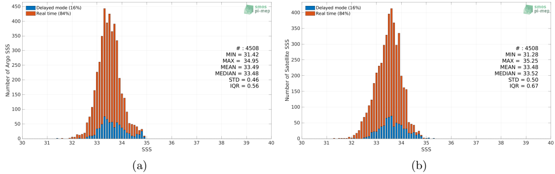
Figure 2: Histograms of SSS from Argo (a) and SMOS and SMAP SSS L4 OI v1 - 7 Days (LOPS) (b) considering all match-up pairs per bins of 0.1 over the South China Sea Pi-MEP region and for the full satellite product period.
