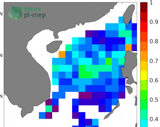
Temporal STD of (Sat - Argo) in 1°x1° boxes over 2011-2018
