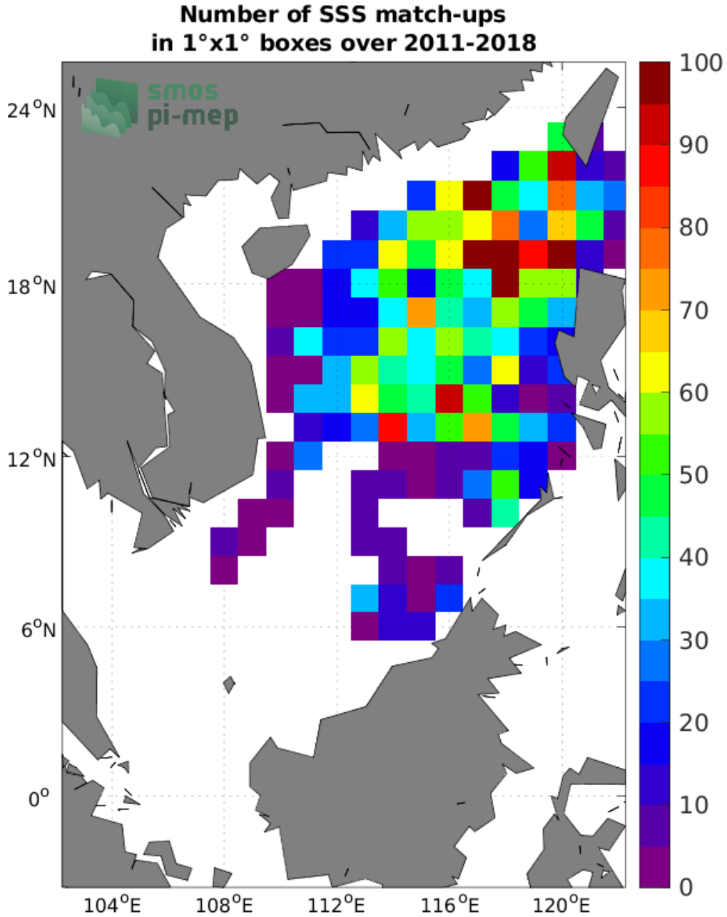
Figure 4: Number of SSS match-ups between Argo SSS and the SMOS and SMAP SSS L4 OI v1 - 7 Days (LOPS) SSS product for the South China Sea Pi-MEP region over 1^\circ \times 1^\circ boxes and for the full satellite product period.
