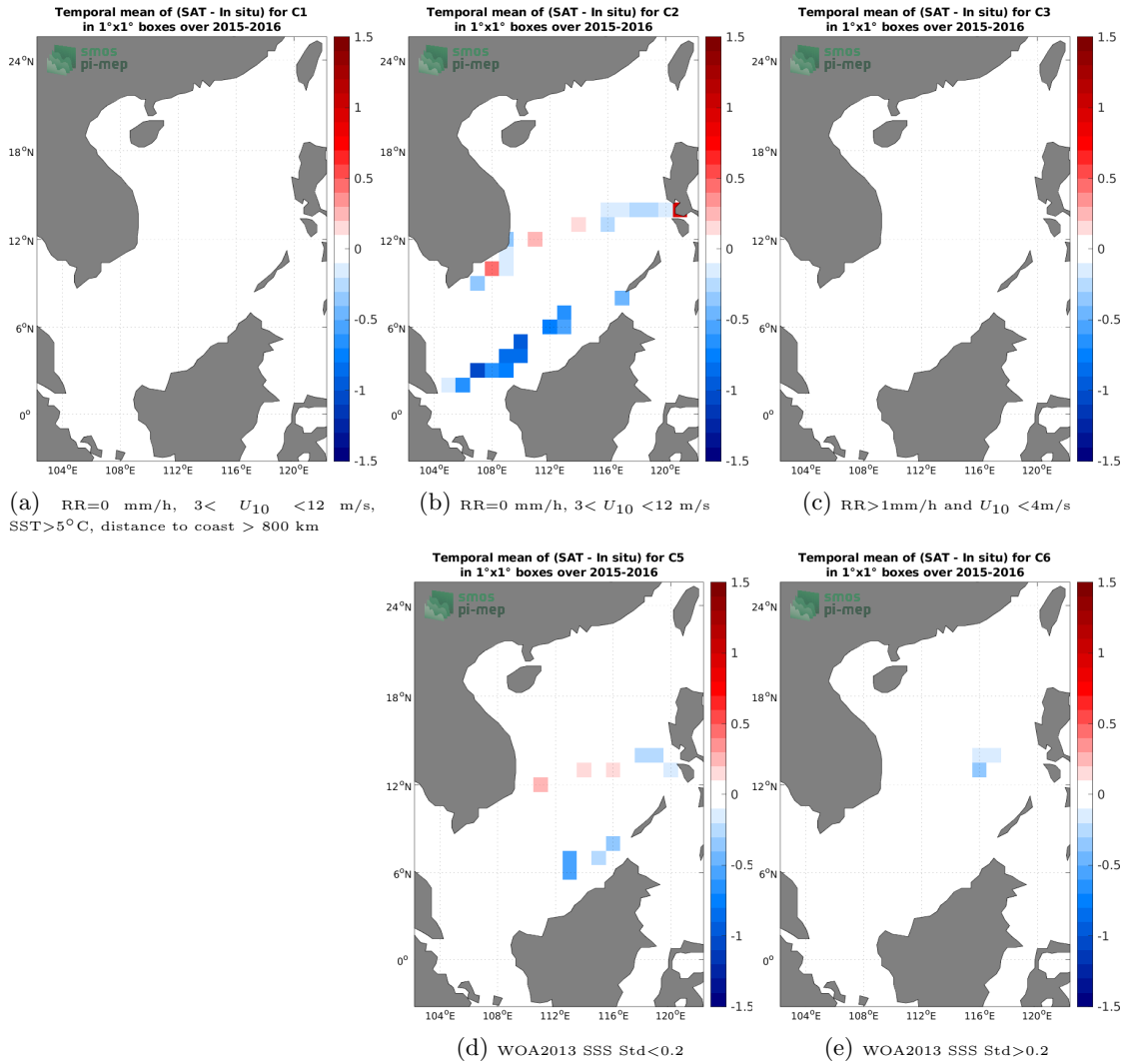
Figure 12: Temporal mean gridded over spatial boxes of size 1^\circ \times 1^\circ of \Delta SSS (SMOS SSS L4 v1 - Weekly (CMEMS-CNR) - TSG (SAMOS)) for 5 different subdatasets corresponding to: RR=0 mm/h, 3 < U_{10} < 12 m/s, SST > 5°C, distance to coast > 800 km (a), RR=0 mm/h, 3 < U_{10} < 12 m/s (b), RR > 1mm/h and U_{10} < 4 m/s (c), WOA2013 SSS Std < 0.2 (d), WOA2013 SSS Std > 0.2 (e).
