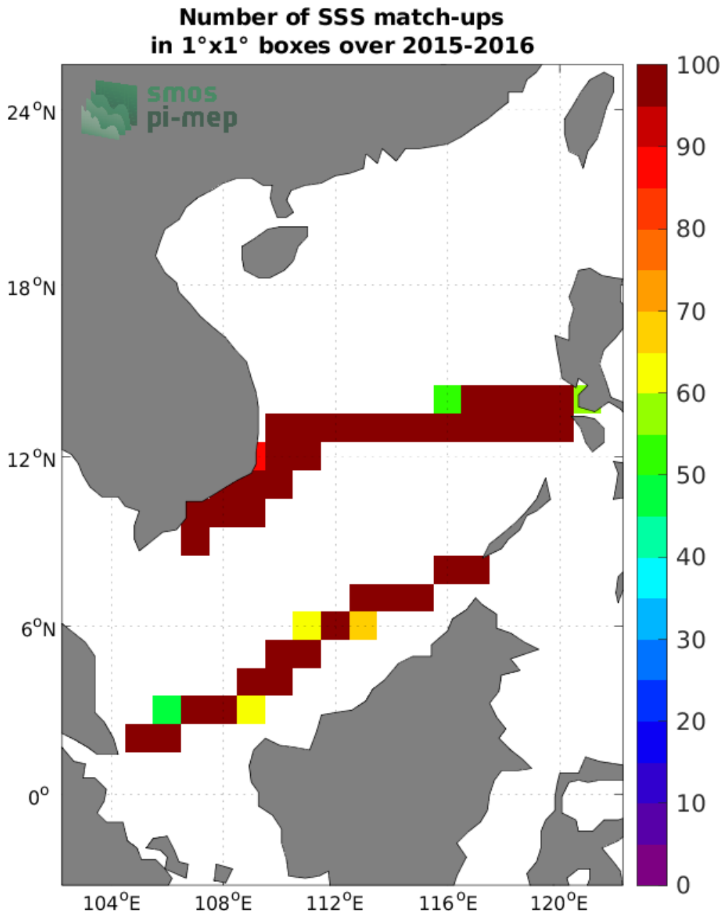
Figure 4: Number of SSS match-ups between TSG (SAMOS) SSS and the SMOS SSS L4 v1 - Weekly (CMEMS-CNR) SSS product for the South China Sea Pi-MEP region over 1^\circ \times 1^\circ boxes and for the full satellite product period.
