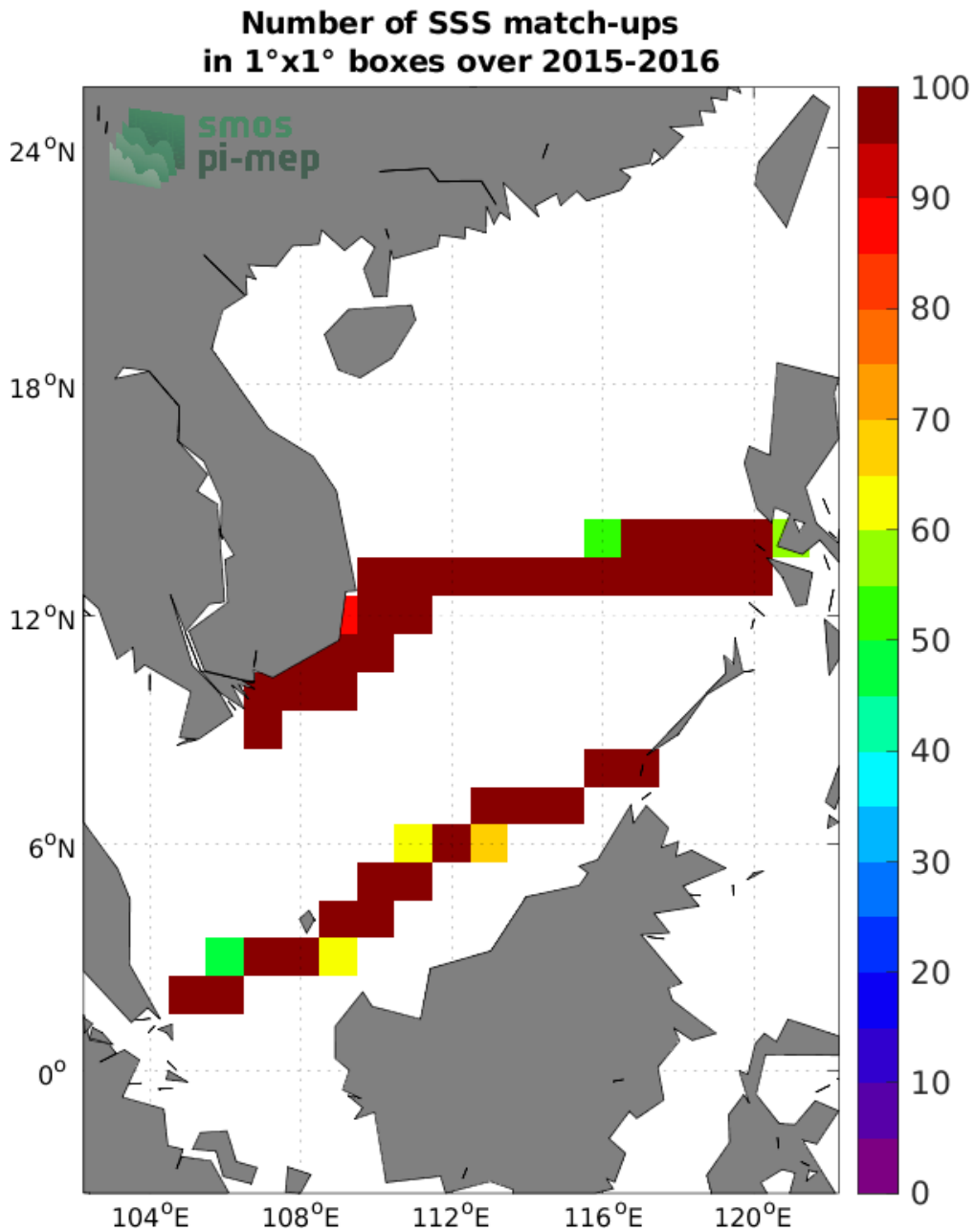
Figure 4: Number of SSS match-ups between TSG (SAMOS) SSS and the SMOS SSS L4 v1 - Weekly (CMEMS-CNR) SSS product for the South China Sea Pi-MEP region over 1°×1° boxes and for the full satellite product period.
