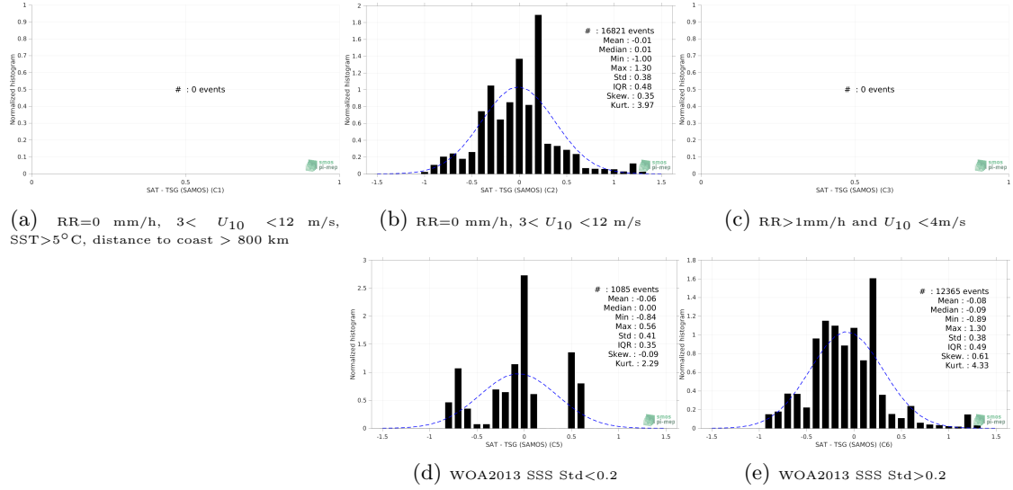
Figure 13: Normalized histogram of \Delta SSS (SMOS SSS L4 v1 - Weekly (CMEMS-CNR) - TSG (SAMOS)) for 5 different subdatasets corresponding to: RR=0 mm/h, 3 < U_{10} < 12 m/s, SST >5^{\circ} C, distance to coast > 800 km (a), RR=0 mm/h, 3 < U_{10} < 12 m/s (b), RR >1 mm/h and U_{10} < 4 m/s (c), WOA2013 SSS Std <0.2 (d), WOA2013 SSS Std >0.2 (e).
