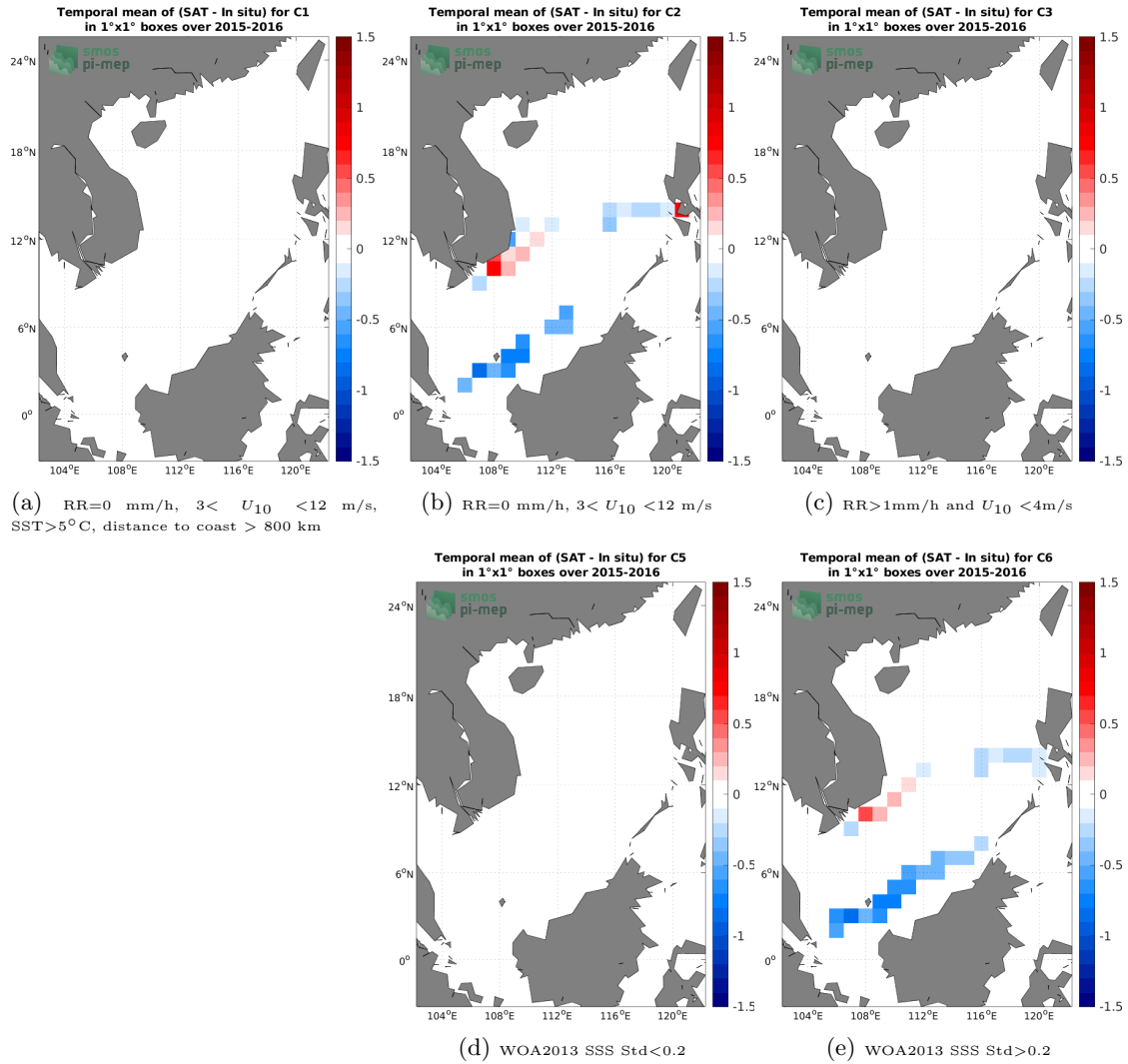
Figure 12: Temporal mean gridded over spatial boxes of size 1^\circ \times 1^\circ of \Delta SSS (SMOS SSS L4 v1 - Weekly (CMEMS-CNR) - TSG (SAMOS)) for 5 different subdatasets corresponding to:RR=0 mm/h, 3 < U_{10} < 12 m/s, SST>5°C, distance to coast > 800 km (a), RR=0 mm/h, 3 < U_{10} < 12 m/s (b), RR>1mm/h and U_{10} < 4 m/s (c), WOA2013 SSS Std<0.2 (d), WOA2013 SSS Std>0.2 (e).
