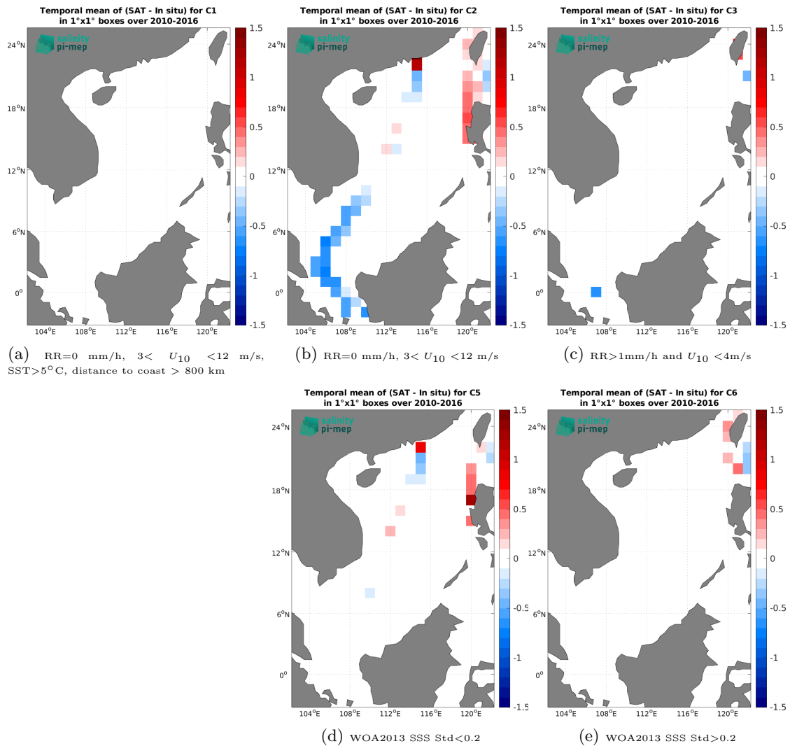
Figure 12: Temporal mean gridded over spatial boxes of size 1^\circ \times 1^\circ of \Delta\text{SSS} (SMOS SSS L4 v1 - Weekly (CMEMS-CNR) - TSG (LEGOS-DM)) for 5 different subdatasets corresponding to: RR=0 mm/h, 3 < U_{10} < 12 m/s, SST > 5^\circ\text{C} , distance to coast > 800 km (a), RR=0 mm/h, 3 < U_{10} < 12 m/s (b), RR > 1 mm/h and U_{10} < 4 m/s (c), WOA2013 SSS Std < 0.2 (d), WOA2013 SSS Std > 0.2 (e).
