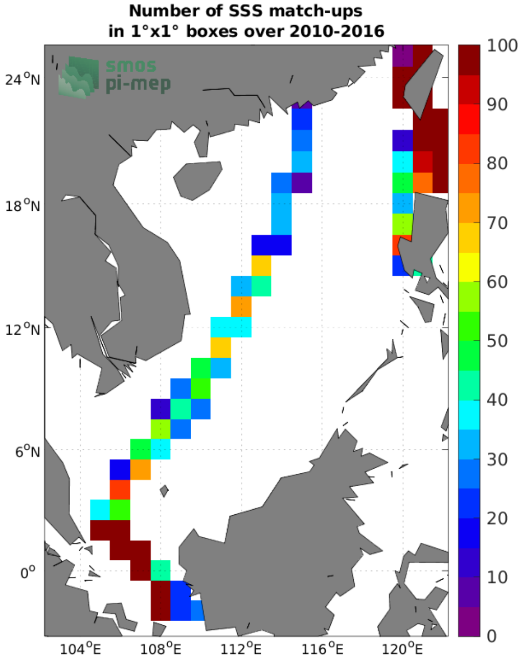
Figure 4: Number of SSS match-ups between TSG (LEGOS-DM) SSS and the SMOS SSS L4 v1 - Weekly (CMEMS-CNR) SSS product for the South China Sea Pi-MEP region over 1°x1° boxes and for the full satellite product period.
