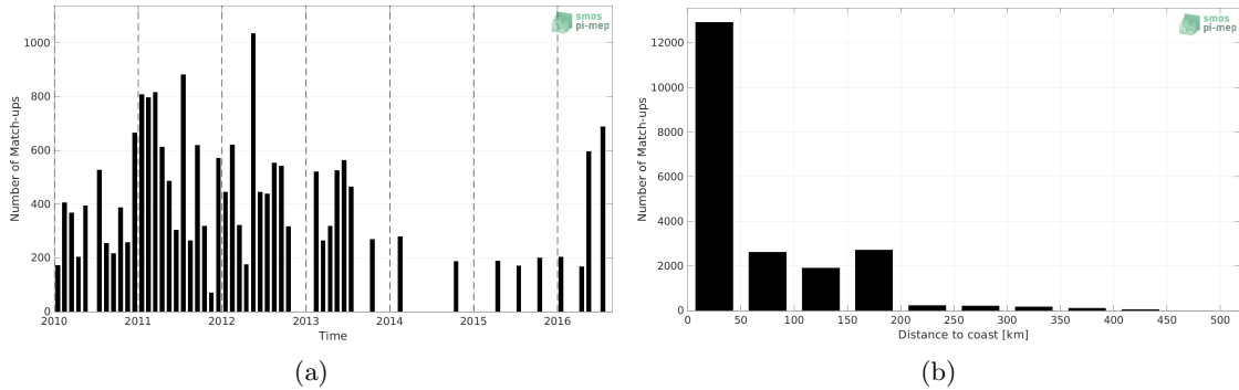
Figure 1: Number of match-ups between TSG (LEGOS-DM) and SMOS SSS L4 v1 - Weekly (CMEMS-CNR) SSS as a function of time (a) and as function of the distance to coast (b) over the South China Sea Pi-MEP region and for the full satellite product period.
