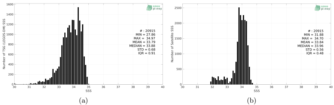
Figure 2: Histograms of SSS from TSG (LEGOS-DM) (a) and SMOS SSS L4 v1 - Weekly (CMEMS-CNR) (b) considering all match-up pairs per bins of 0.1 over the South China Sea Pi-MEP region and for the full satellite product period.
