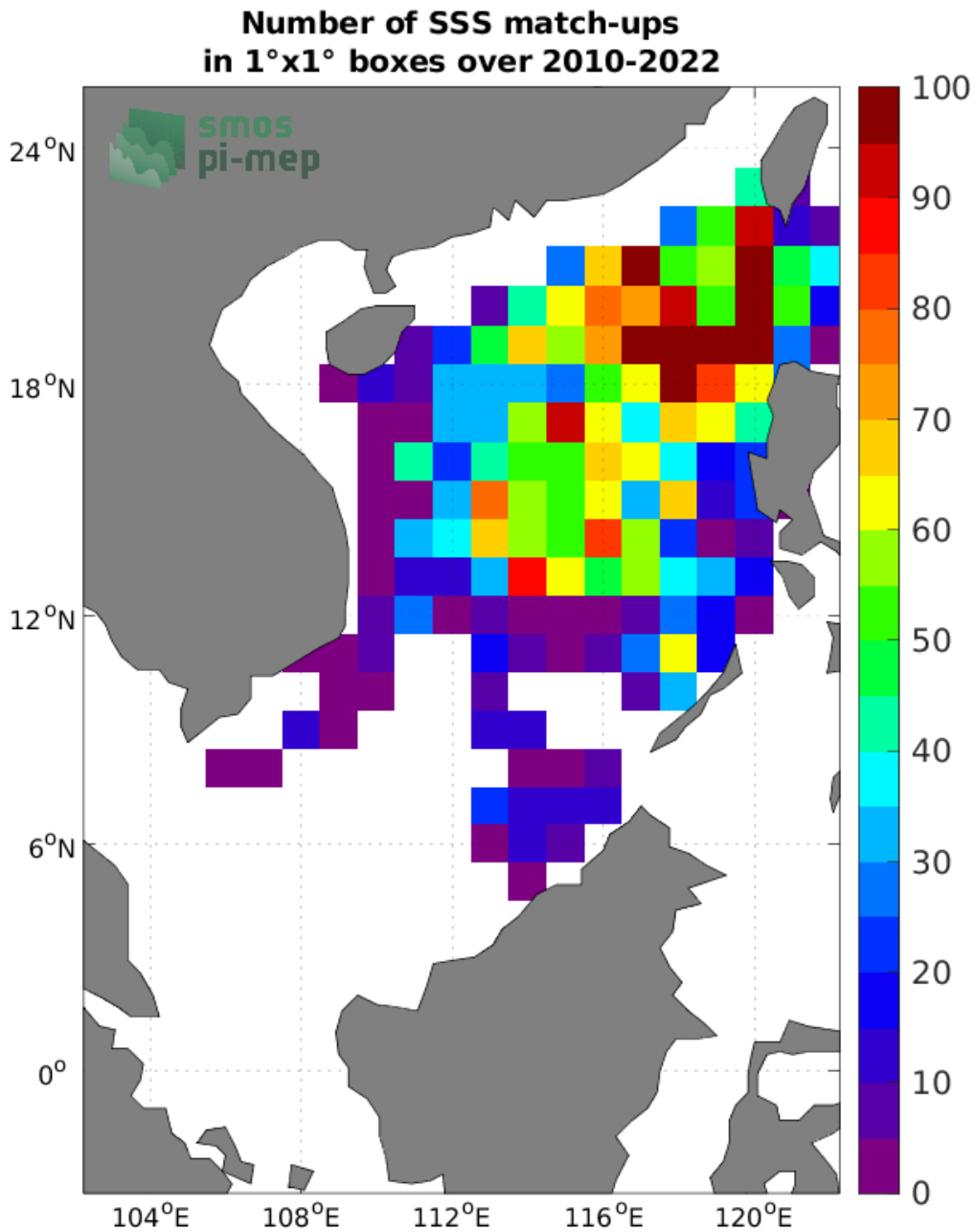
Figure 4: Number of SSS match-ups between Argo SSS and the SMOS SSS L4 v1 - Weekly (CMEMS-CNR) SSS product for the South China Sea Pi-MEP region over 1°x1° boxes and for the full satellite product period.
