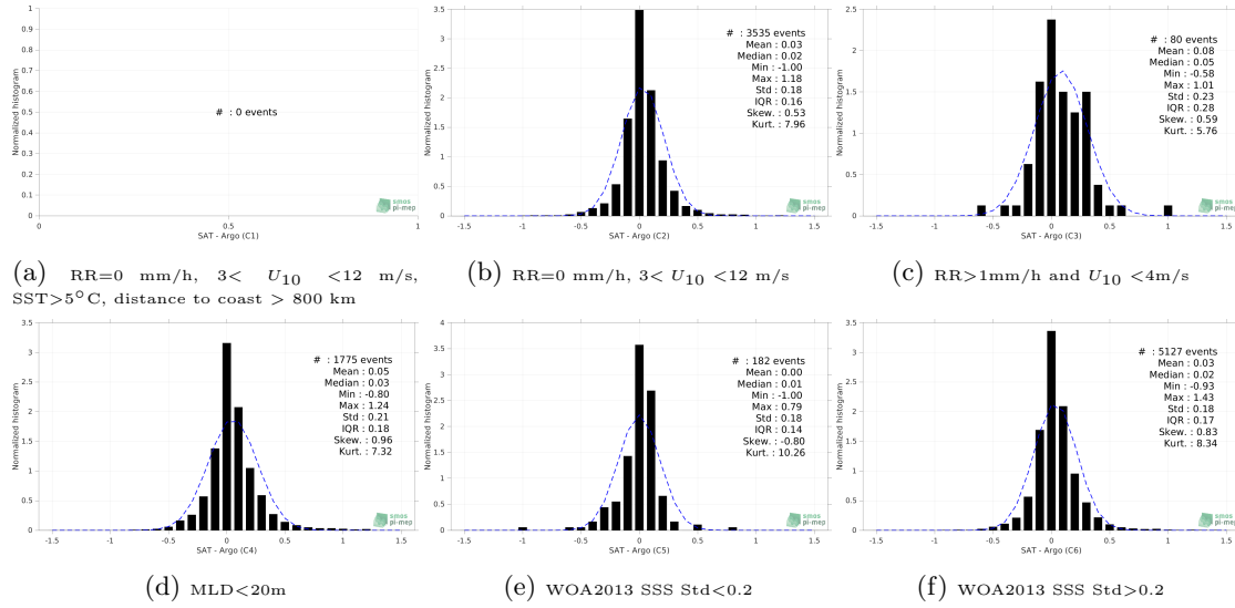
Figure 13: Normalized histogram of \Delta\text{SSS} (SMOS SSS L4 v1 - Weekly (CMEMS-CNR) - Argo) for 6 different subdatasets corresponding to: RR=0 mm/h, 3 < U_{10} < 12 m/s, SST>5°C, distance to coast > 800 km (a), RR=0 mm/h, 3 < U_{10} < 12 m/s (b), RR>1mm/h and U_{10} < 4 m/s (c), MLD<20m (d), WOA2013 SSS Std<0.2 (e), WOA2013 SSS Std>0.2 (f).
