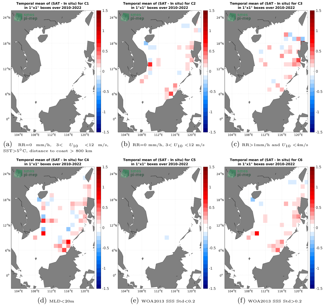
Figure 12: Temporal mean gridded over spatial boxes of size 1^\circ \times 1^\circ of \Delta SSS (SMOS SSS L4 v1 - Weekly (CMEMS-CNR) - Argo) for 6 different subdatasets corresponding to: RR=0 mm/h, 3 < U_{10} < 12 m/s, SST > 5^\circ C , distance to coast > 800 km (a), RR=0 mm/h, 3 < U_{10} < 12 m/s (b), RR > 1 mm/h and U_{10} < 4 m/s (c), MLD < 20 m (d), WOA2013 SSS Std < 0.2 (e), WOA2013 SSS Std > 0.2 (f).
