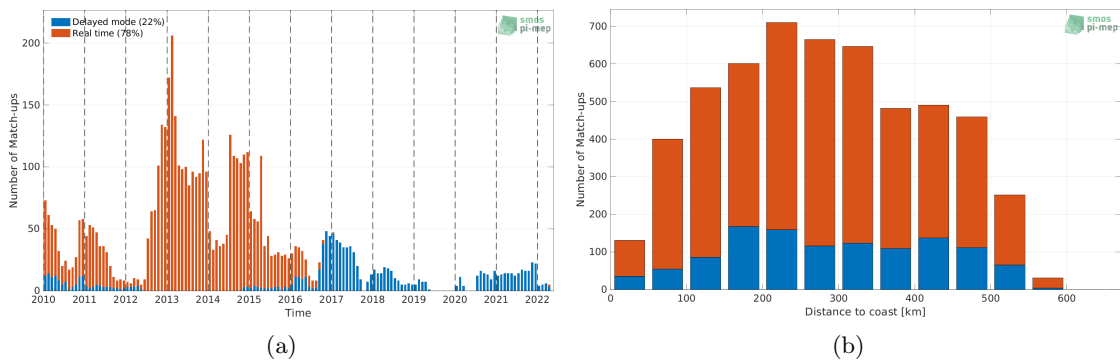
Figure 1: Number of match-ups between Argo and SMOS SSS L4 v1 - Weekly (CMEMS-CNR) SSS as a function of time (a) and as function of the distance to coast (b) over the South China Sea Pi-MEP region and for the full satellite product period.
