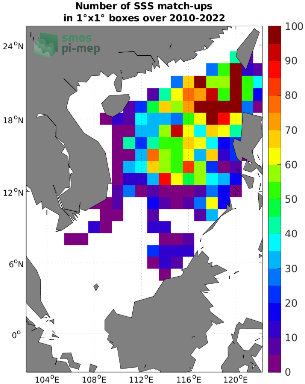
Figure 4: Number of SSS match-ups between Argo SSS and the SMOS SSS L4 v1 - Weekly (CMEMS-CNR) SSS product for the South China Sea Pi-MEP region over 1^\circ \times 1^\circ boxes and for the full satellite product period.
