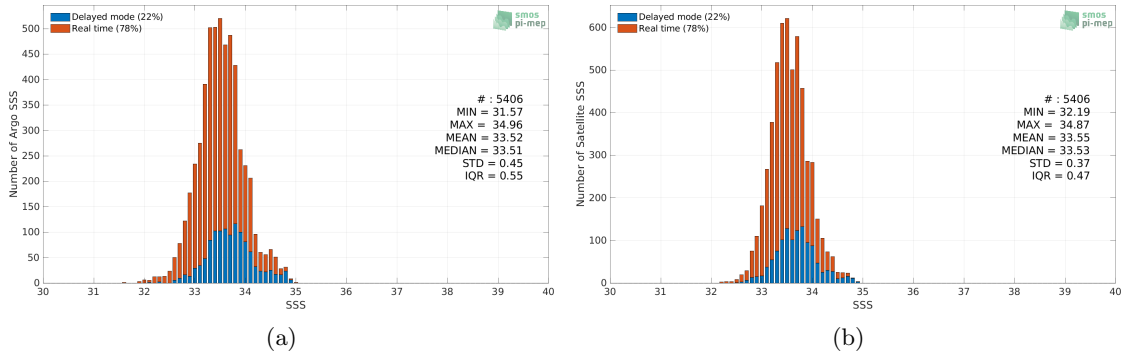
Figure 2: Histograms of SSS from Argo (a) and SMOS SSS L4 v1 - Weekly (CMEMS-CNR) (b) considering all match-up pairs per bins of 0.1 over the South China Sea Pi-MEP region and for the full satellite product period.
