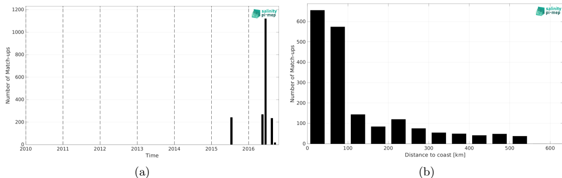
Figure 2: Number of match-ups between TSG (SAMOS) and SMOS SSS L4 v1 - Monthly (CMEMS-CNR) SSS as a function of time (a) and as function of the distance to coast (b) over the South China Sea Pi-MEP region and for the full satellite product period.
