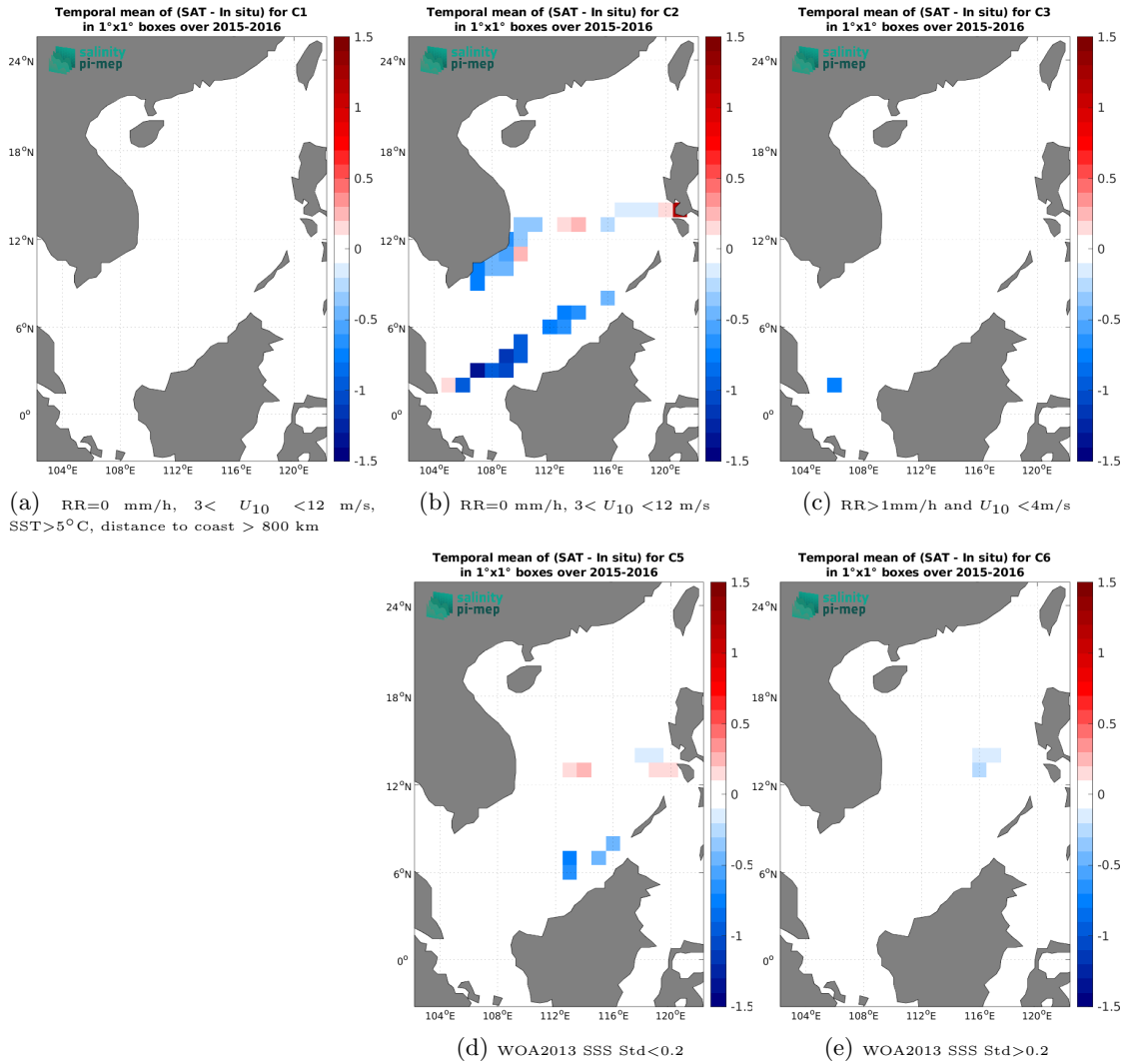
Figure 14: Temporal mean gridded over spatial boxes of size 1^\circ \times 1^\circ of \Delta\text{SSS} (SMOS SSS L4 v1 - Monthly (CMEMS-CNR) - TSG (SAMOS)) for 5 different subdatasets corresponding to: RR=0 mm/h, 3 < U_{10} < 12 m/s, SST > 5^\circ\text{C} , distance to coast > 800 km (a), RR=0 mm/h, 3 < U_{10} < 12 m/s (b), RR > 1 mm/h and U_{10} < 4 m/s (c), WOA2013 SSS Std < 0.2 (d), WOA2013 SSS Std > 0.2 (e).
