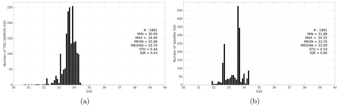
Figure 3: Histograms of SSS from TSG (SAMOS) (a) and SMOS SSS L4 v1 - Monthly (CMEMS-CNR) (b) considering all match-up pairs per bins of 0.1 over the South China Sea Pi-MEP region and for the full satellite product period.
