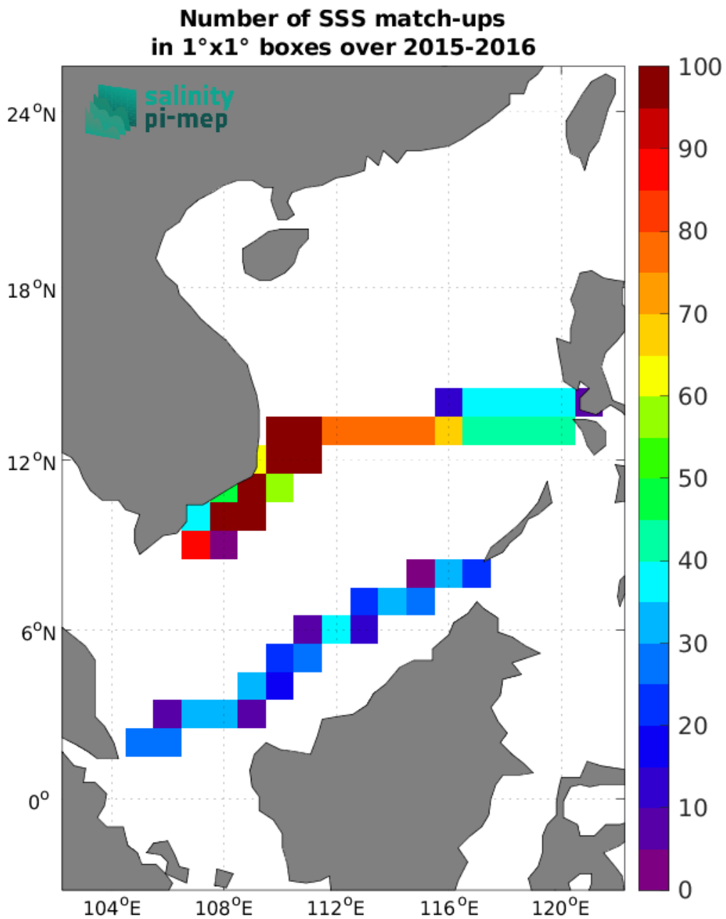
Figure 4: Number of SSS match-ups between TSG (SAMOS) SSS and the SMOS SSS L4 v1 - Monthly (CMEMS-CNR) SSS product for the South China Sea Pi-MEP region over 1^{\circ} \times 1^{\circ} boxes and for the full satellite product period.
