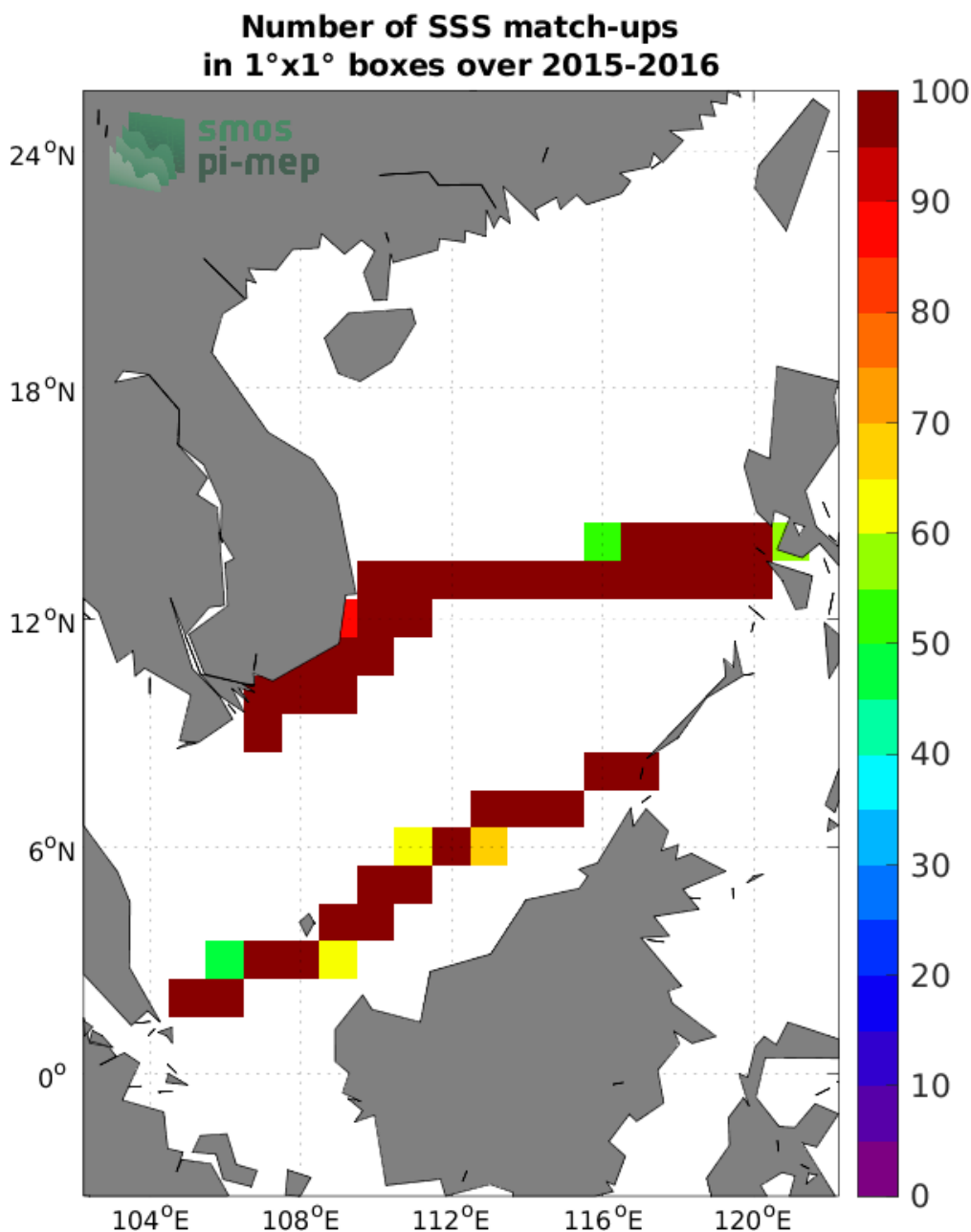
Figure 4: Number of SSS match-ups between TSG (SAMOS) SSS and the SMOS SSS L4 v1 - Monthly (CMEMS-CNR) SSS product for the South China Sea Pi-MEP region over 1°×1° boxes and for the full satellite product period.
