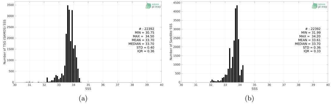
Figure 2: Histograms of SSS from TSG (SAMOS) (a) and SMOS SSS L4 v1 - Monthly (CMEMS-CNR) (b) considering all match-up pairs per bins of 0.1 over the South China Sea Pi-MEP region and for the full satellite product period.
