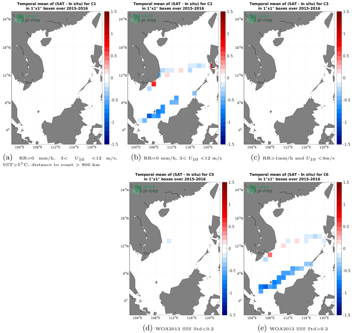
Figure 12: Temporal mean gridded over spatial boxes of size 1^\circ \times 1^\circ of \Delta\text{SSS} (SMOS SSS L4 v1 - Monthly (CMEMS-CNR) - TSG (SAMOS)) for 5 different subdatasets corresponding to: RR=0 mm/h, 3 < U_{10} < 12 m/s, SST > 5^\circ\text{C} , distance to coast > 800 km (a), RR=0 mm/h, 3 < U_{10} < 12 m/s (b), RR > 1 mm/h and U_{10} < 4 m/s (c), WOA2013 SSS Std < 0.2 (d), WOA2013 SSS Std > 0.2 (e).
