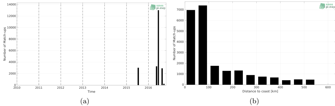
Figure 1: Number of match-ups between TSG (SAMOS) and SMOS SSS L4 v1 - Monthly (CMEMS-CNR) SSS as a function of time (a) and as function of the distance to coast (b) over the South China Sea Pi-MEP region and for the full satellite product period.
