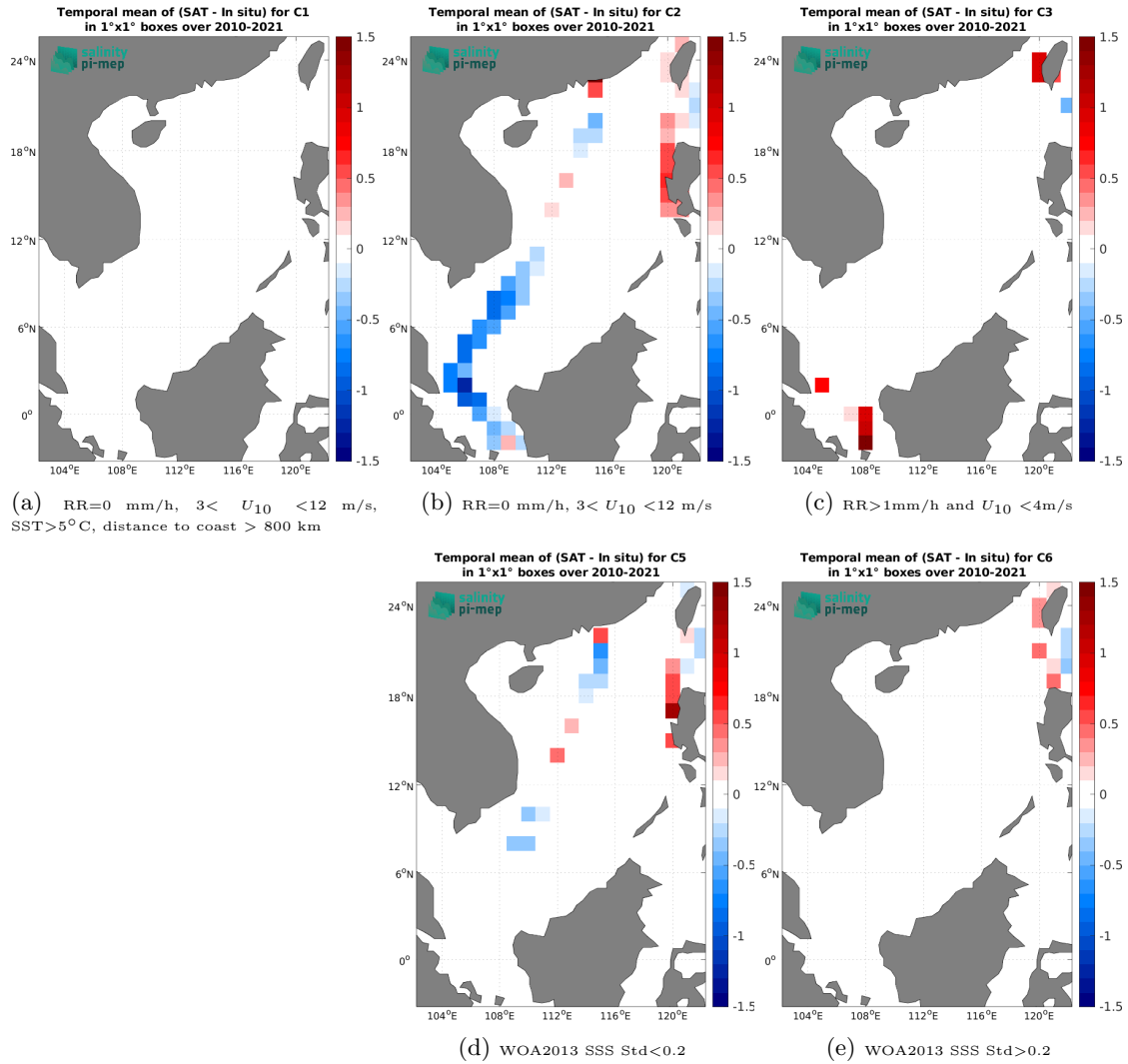
Figure 14: Temporal mean gridded over spatial boxes of size 1^\circ \times 1^\circ of \Delta\text{SSS} (SMOS SSS L4 v1 - Monthly (CMEMS-CNR) - TSG (LEGOS-DM)) for 5 different subdatasets corresponding to: RR=0 mm/h, 3 < U_{10} < 12 m/s, SST > 5^\circ\text{C} , distance to coast > 800 km (a), RR=0 mm/h, 3 < U_{10} < 12 m/s (b), RR > 1 mm/h and U_{10} < 4 m/s (c), WOA2013 SSS Std < 0.2 (d), WOA2013 SSS Std > 0.2 (e).
