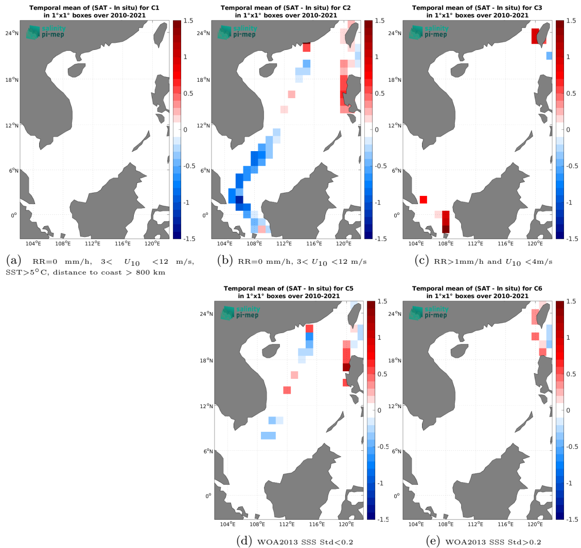
Figure 14: Temporal mean gridded over spatial boxes of size 1^{\circ} \times 1^{\circ} of \Delta SSS (SMOS SSS L4 v1 - Monthly (CMEMS-CNR) - TSG (LEGOS-DM)) for 5 different subdatasets corresponding to: RR=0 mm/h, 3 < U_{10} < 12 m/s, SST > 5^{\circ}C , distance to coast > 800 km (a), RR=0 mm/h, 3 < U_{10} < 12 m/s (b), RR > 1 mm/h and U_{10} < 4 m/s (c), WOA2013 SSS Std < 0.2 (d), WOA2013 SSS Std > 0.2 (e).
