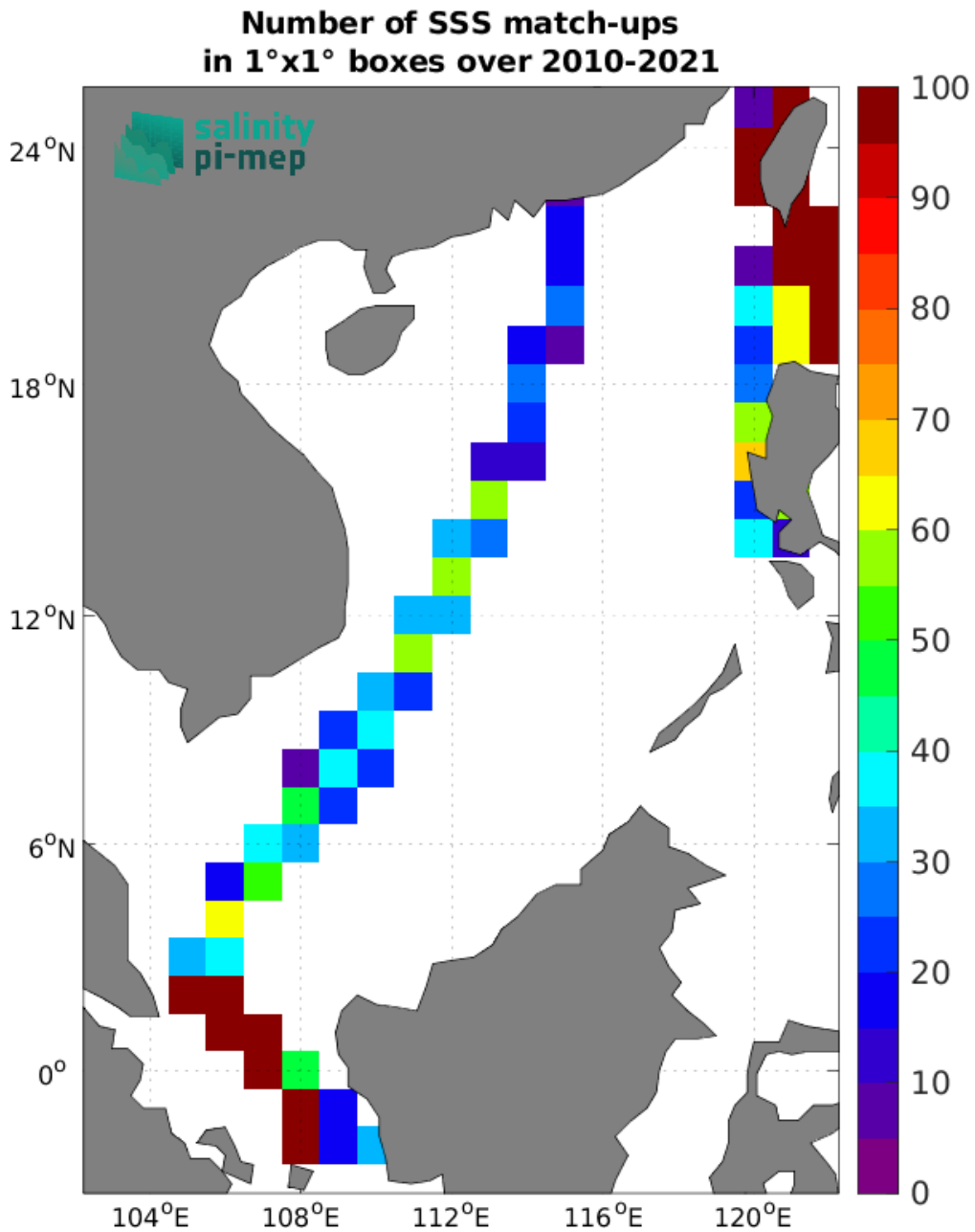
Figure 5: Number of SSS match-ups between TSG (LEGOS-DM) SSS and the SMOS SSS L4 v1 - Monthly (CMEMS-CNR) SSS product for the South China Sea Pi-MEP region over 1°x1° boxes and for the full satellite product period.
