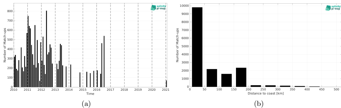
Figure 2: Number of match-ups between TSG (LEGOS-DM) and SMOS SSS L4 v1 - Monthly (CMEMS-CNR) SSS as a function of time (a) and as function of the distance to coast (b) over the South China Sea Pi-MEP region and for the full satellite product period.
