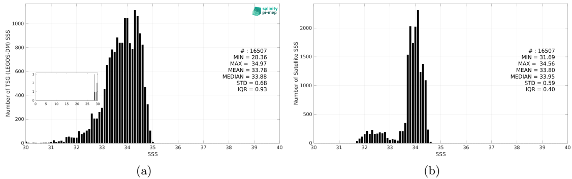
Figure 3: Histograms of SSS from TSG (LEGOS-DM) (a) and SMOS SSS L4 v1 - Monthly (CMEMS-CNR) (b) considering all match-up pairs per bins of 0.1 over the South China Sea Pi-MEP region and for the full satellite product period.
