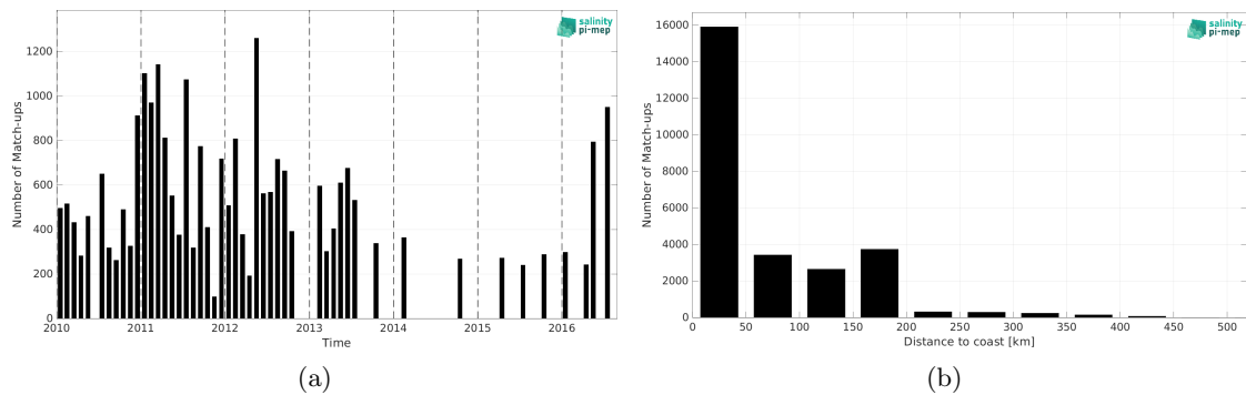
Figure 1: Number of match-ups between TSG (LEGOS-DM) and SMOS SSS L4 v1 - Monthly (CMEMS-CNR) SSS as a function of time (a) and as function of the distance to coast (b) over the South China Sea Pi-MEP region and for the full satellite product period.
