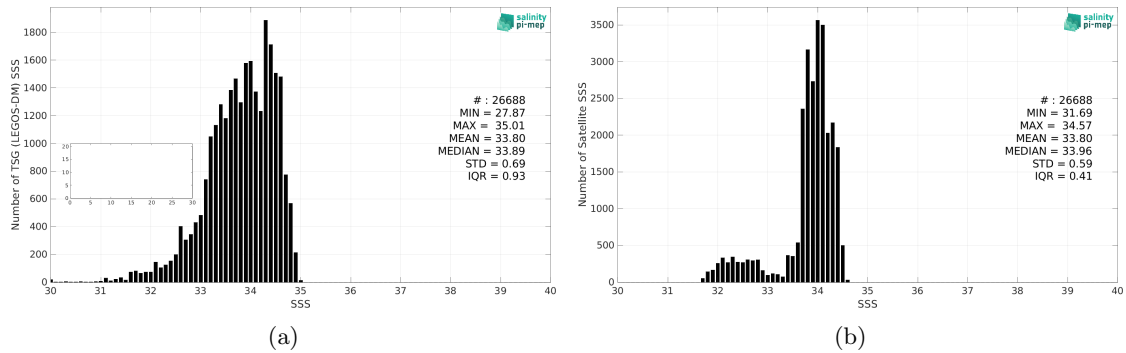
Figure 2: Histograms of SSS from TSG (LEGOS-DM) (a) and SMOS SSS L4 v1 - Monthly (CMEMS-CNR) (b) considering all match-up pairs per bins of 0.1 over the South China Sea Pi-MEP region and for the full satellite product period.
