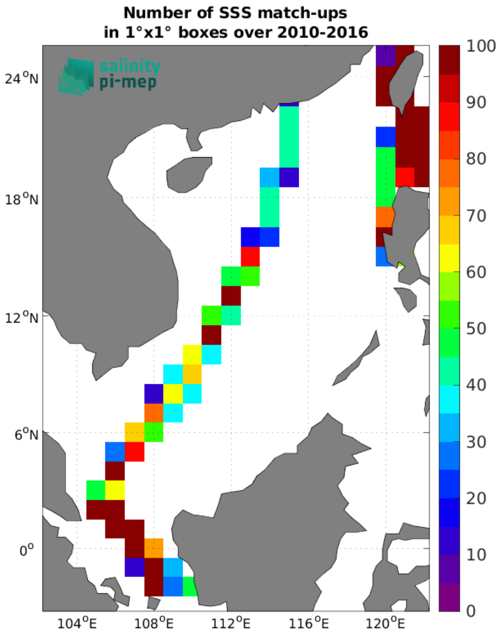
Figure 4: Number of SSS match-ups between TSG (LEGOS-DM) SSS and the SMOS SSS L4 v1 - Monthly (CMEMS-CNR) SSS product for the South China Sea Pi-MEP region over 1°x1° boxes and for the full satellite product period.
