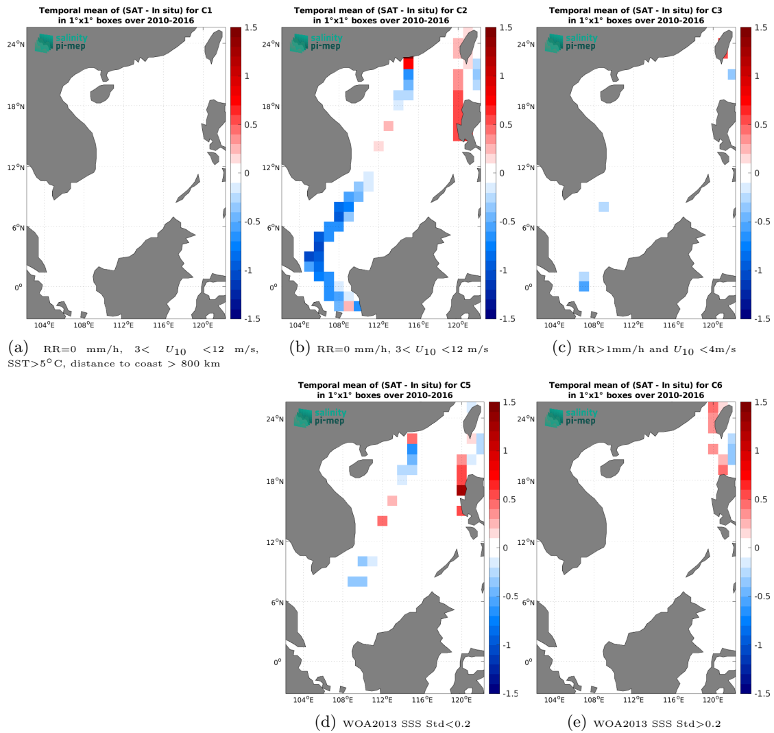
Figure 12: Temporal mean gridded over spatial boxes of size 1^\circ \times 1^\circ of \Delta\text{SSS} (SMOS SSS L4 v1 - Monthly (CMEMS-CNR) - TSG (LEGOS-DM)) for 5 different subdatasets corresponding to: RR=0 mm/h, 3 < U_{10} < 12 m/s, SST > 5^\circ\text{C} , distance to coast > 800 km (a), RR=0 mm/h, 3 < U_{10} < 12 m/s (b), RR > 1 mm/h and U_{10} < 4 m/s (c), WOA2013 SSS Std < 0.2 (d), WOA2013 SSS Std > 0.2 (e).
