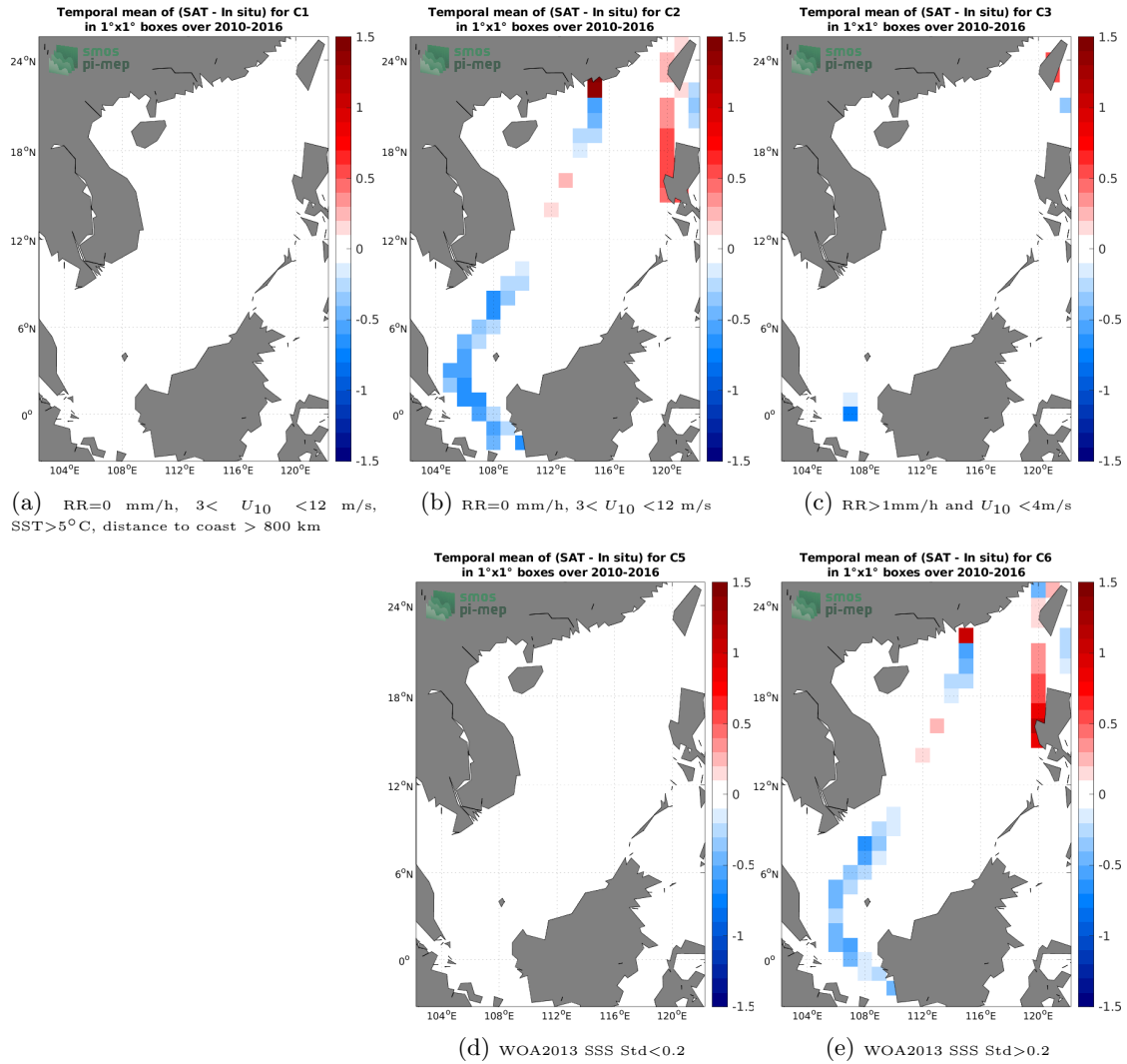
Figure 12: Temporal mean gridded over spatial boxes of size 1^\circ \times 1^\circ of \Delta SSS (SMOS SSS L4 v1 - Monthly (CMEMS-CNR) - TSG (LEGOS-DM)) for 5 different subdatasets corresponding to: RR=0 mm/h, 3 < U_{10} < 12 m/s, SST>5°C, distance to coast > 800 km (a), RR=0 mm/h, 3 < U_{10} < 12 m/s (b), RR>1mm/h and U_{10} < 4 m/s (c), WOA2013 SSS Std<0.2 (d), WOA2013 SSS Std>0.2 (e).
