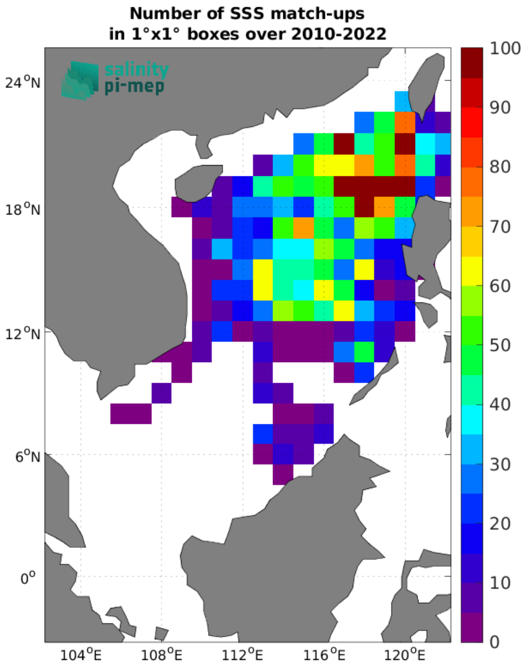
Figure 5: Number of SSS match-ups between Argo SSS and the SMOS SSS L4 v1 - Monthly (CMEMS-CNR) SSS product for the South China Sea Pi-MEP region over 1^\circ \times 1^\circ boxes and for the full satellite product period.
