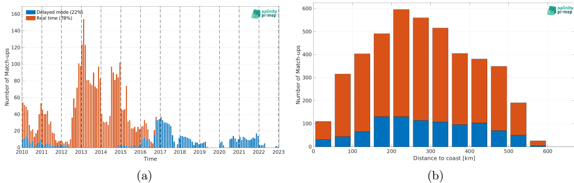
Figure 2: Number of match-ups between Argo and SMOS SSS L4 v1 - Monthly (CMEMS-CNR) SSS as a function of time (a) and as function of the distance to coast (b) over the South China Sea Pi-MEP region and for the full satellite product period.
