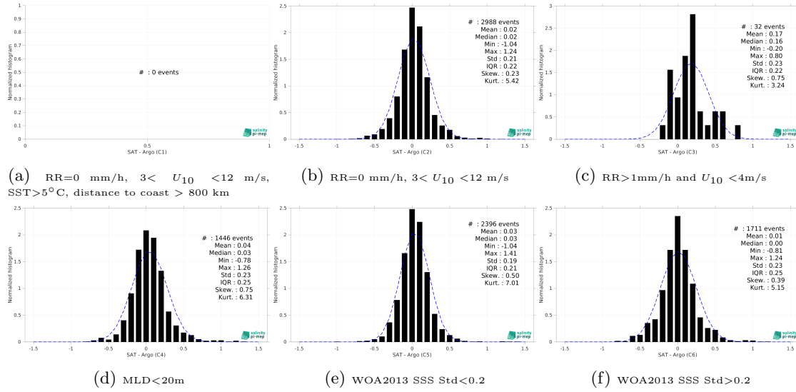
Figure 15: Normalized histogram of \Delta\text{SSS} (SMOS SSS L4 v1 - Monthly (CMEMS-CNR) - Argo) for 6 different subdatasets corresponding to: RR=0 mm/h, 3 < U_{10} < 12 m/s, SST>5°C, distance to coast > 800 km (a), RR=0 mm/h, 3 < U_{10} < 12 m/s (b), RR>1mm/h and U_{10} < 4 m/s (c), MLD<20m (d), WOA2013 SSS Std<0.2 (e), WOA2013 SSS Std>0.2 (f).
