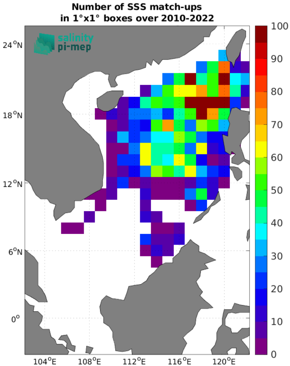
Figure 5: Number of SSS match-ups between Argo SSS and the SMOS SSS L4 v1 - Monthly (CMEMS-CNR) SSS product for the South China Sea Pi-MEP region over 1^{\circ} \times 1^{\circ} boxes and for the full satellite product period.
