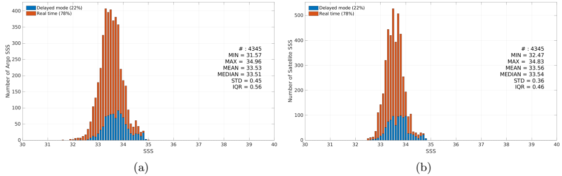
Figure 3: Histograms of SSS from Argo (a) and SMOS SSS L4 v1 - Monthly (CMEMS-CNR) (b) considering all match-up pairs per bins of 0.1 over the South China Sea Pi-MEP region and for the full satellite product period.
