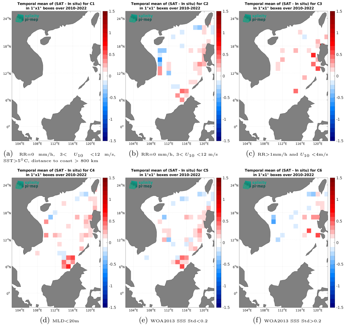
Figure 14: Temporal mean gridded over spatial boxes of size 1^\circ \times 1^\circ of \Delta SSS (SMOS SSS L4 v1 - Monthly (CMEMS-CNR) - Argo) for 6 different subdatasets corresponding to: RR=0 mm/h, 3 < U_{10} < 12 m/s, SST>5°C, distance to coast > 800 km (a), RR=0 mm/h, 3 < U_{10} < 12 m/s (b), RR>1mm/h and U_{10} < 4 m/s (c),MLD<20m (d),WOA2013 SSS Std<0.2 (e),WOA2013 SSS Std>0.2 (f).
