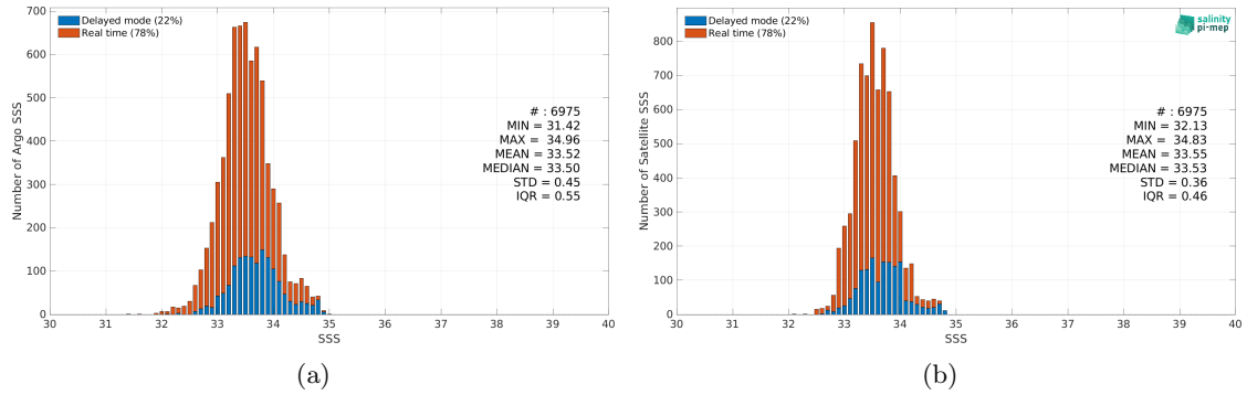
Figure 2: Histograms of SSS from Argo (a) and SMOS SSS L4 v1 - Monthly (CMEMS-CNR) (b) considering all match-up pairs per bins of 0.1 over the South China Sea Pi-MEP region and for the full satellite product period.
