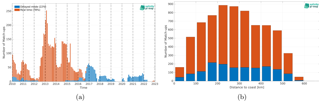
Figure 1: Number of match-ups between Argo and SMOS SSS L4 v1 - Monthly (CMEMS-CNR) SSS as a function of time (a) and as function of the distance to coast (b) over the South China Sea Pi-MEP region and for the full satellite product period.
