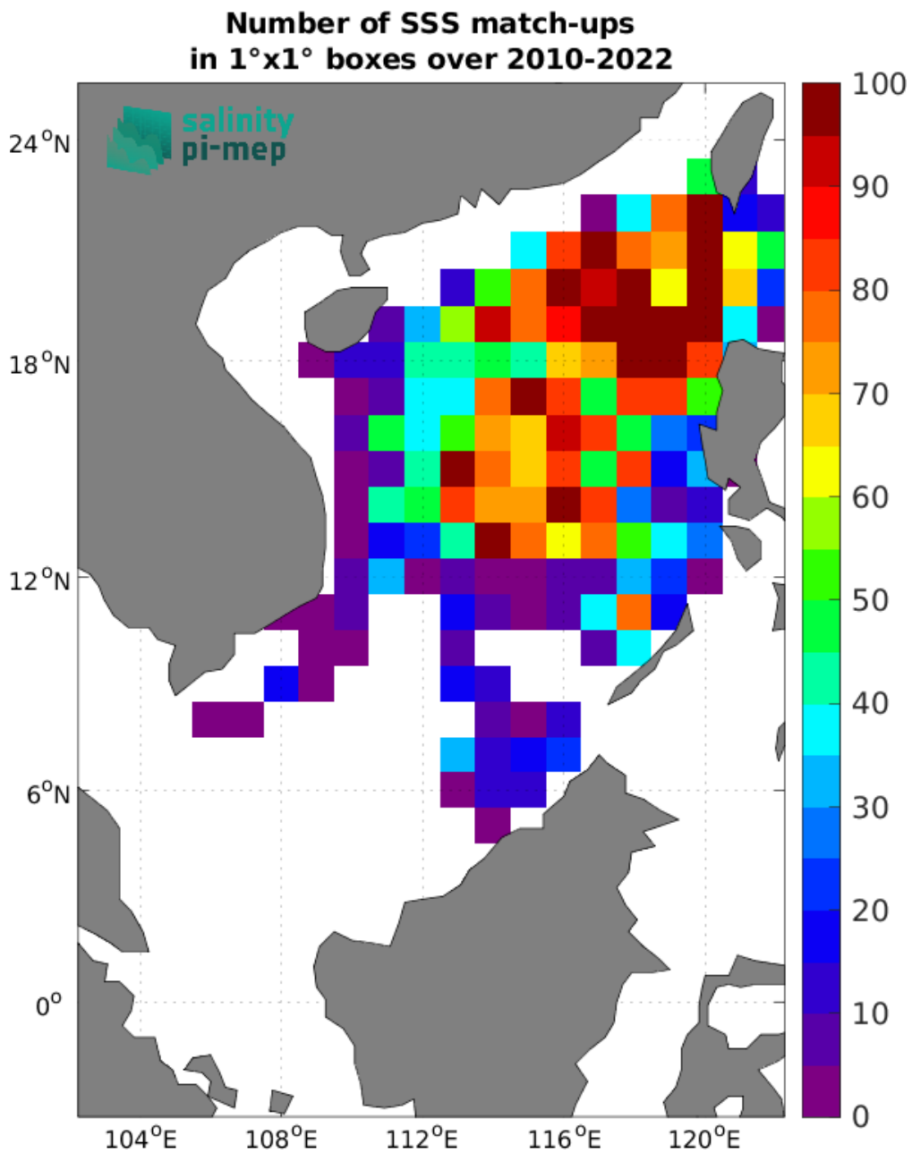
Figure 4: Number of SSS match-ups between Argo SSS and the SMOS SSS L4 v1 - Monthly (CMEMS-CNR) SSS product for the South China Sea Pi-MEP region over 1^\circ \times 1^\circ boxes and for the full satellite product period.
