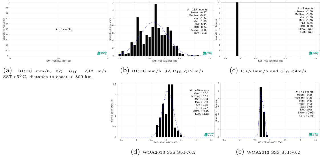
Figure 15: Normalized histogram of \Delta SSS (SMOS SSS L4 v1 - Daily (CMEMS-CNR) - TSG (SAMOS)) for 5 different subdatasets corresponding to: RR=0 mm/h, 3 < U_{10} < 12 m/s, SST > 5°C, distance to coast > 800 km (a), RR=0 mm/h, 3 < U_{10} < 12 m/s (b), RR > 1mm/h and U_{10} < 4 m/s (c), WOA2013 SSS Std < 0.2 (d), WOA2013 SSS Std > 0.2 (e).
