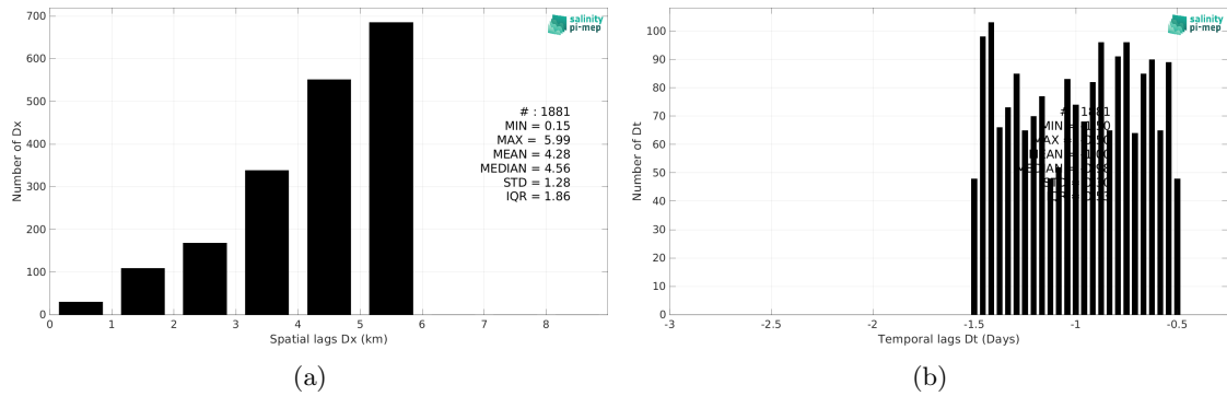
Figure 6: Histograms of the spatial (a) and temporal (b) lags between the location/time of the TSG (SAMOS) measurement and the date of the corresponding SMOS SSS L4 v1 - Daily (CMEMS-CNR) SSS pixel.
