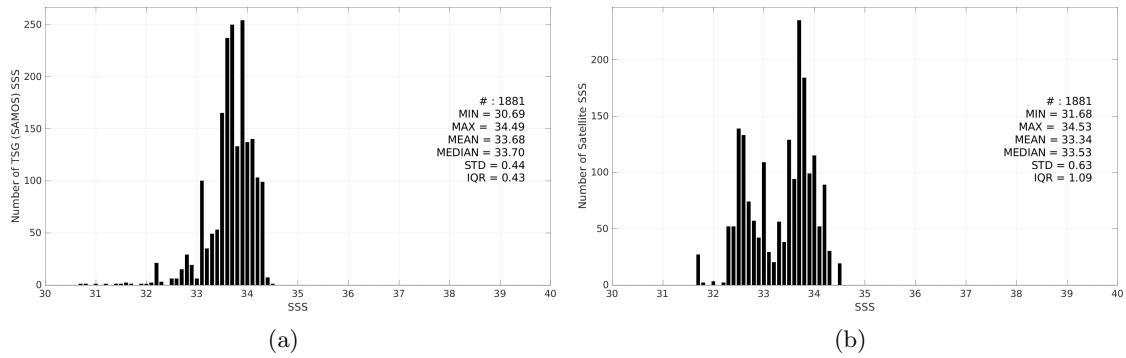
Figure 3: Histograms of SSS from TSG (SAMOS) (a) and SMOS SSS L4 v1 - Daily (CMEMS-CNR) (b) considering all match-up pairs per bins of 0.1 over the South China Sea Pi-MEP region and for the full satellite product period.
