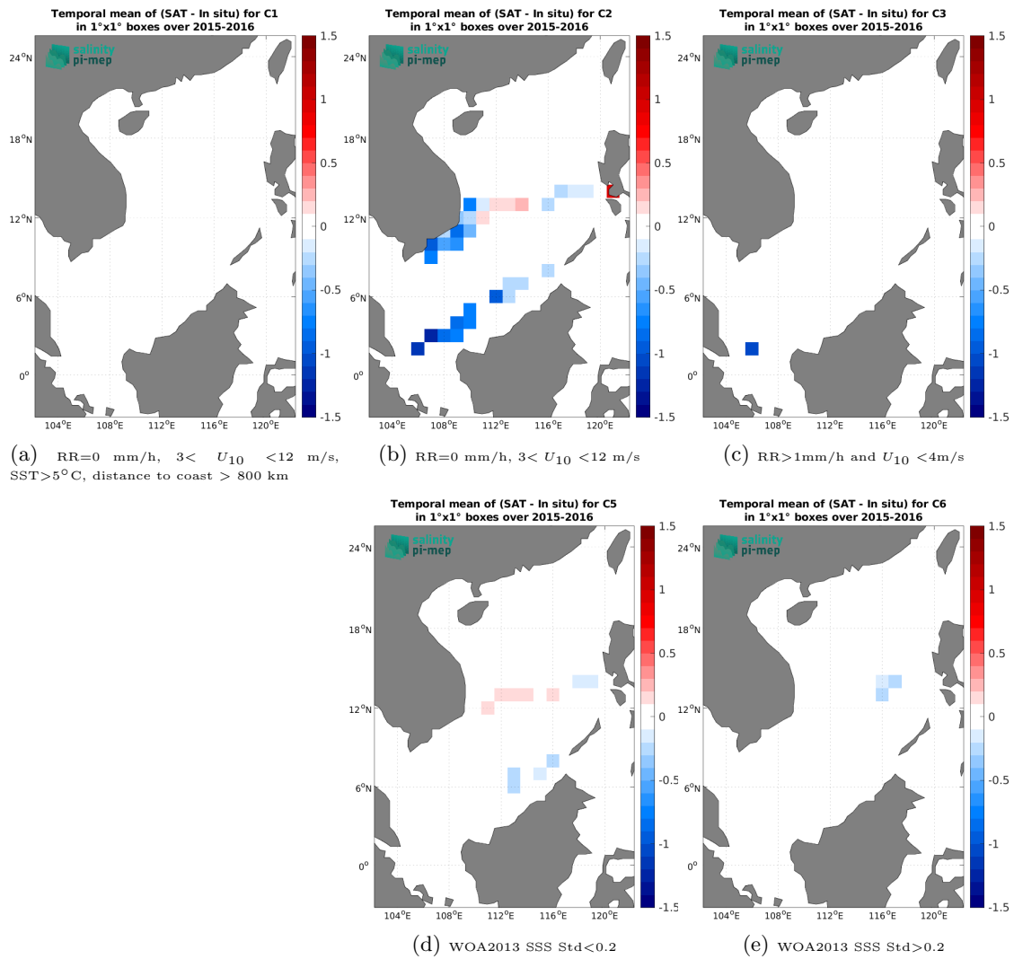
Figure 14: Temporal mean gridded over spatial boxes of size 1^\circ \times 1^\circ of \Delta\text{SSS} (SMOS SSS L4 v1 - Daily (CMEMS-CNR) - TSG (SAMOS)) for 5 different subdatasets corresponding to: RR=0 mm/h, 3 < U_{10} < 12 m/s, SST > 5^\circ\text{C} , distance to coast > 800 km (a), RR=0 mm/h, 3 < U_{10} < 12 m/s (b), RR > 1 mm/h and U_{10} < 4 m/s (c), WOA2013 SSS Std < 0.2 (d), WOA2013 SSS Std > 0.2 (e).
