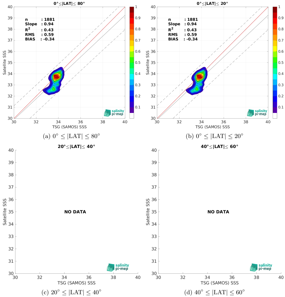
Figure 10: Contour maps of the concentration of SMOS SSS L4 v1 - Daily (CMEMS-CNR) SSS (y-axis) versus TSG (SAMOS) SSS (x-axis) at match-up pairs for different latitude bands. For each plot, the red line shows x=y . The black thin and dashed lines indicate a linear fit through the data cloud and the \pm 95\% confidence levels, respectively. The number match-up pairs n , the slope and R^2 coefficient of the linear fit, the root mean square (RMS) and the mean bias between satellite and in situ data are indicated for each latitude band in each plots.
