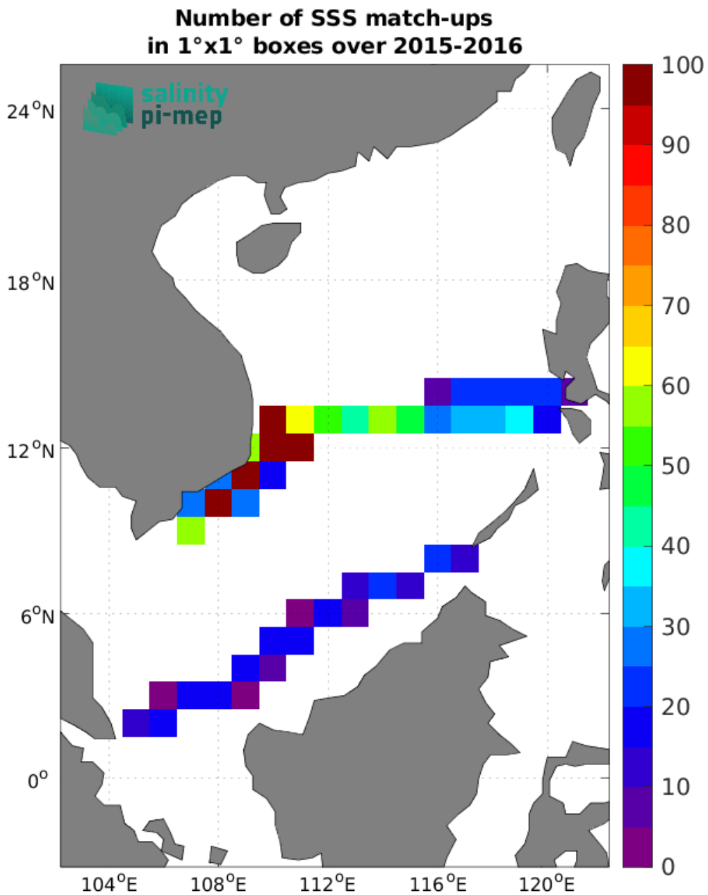
Figure 5: Number of SSS match-ups between TSG (SAMOS) SSS and the SMOS SSS L4 v1 - Daily (CMEMS-CNR) SSS product for the South China Sea Pi-MEP region over 1^\circ \times 1^\circ boxes and for the full satellite product period.
