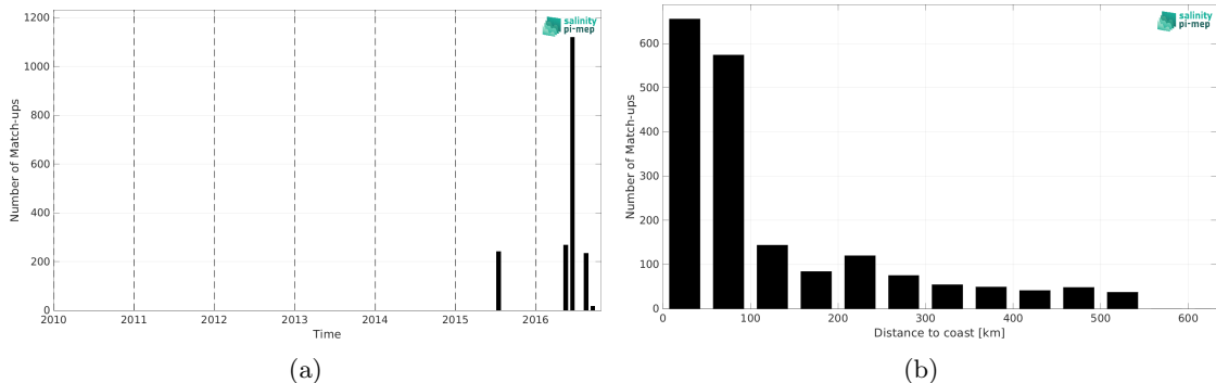
Figure 2: Number of match-ups between TSG (SAMOS) and SMOS SSS L4 v1 - Daily (CMEMS-CNR) SSS as a function of time (a) and as function of the distance to coast (b) over the South China Sea Pi-MEP region and for the full satellite product period.
