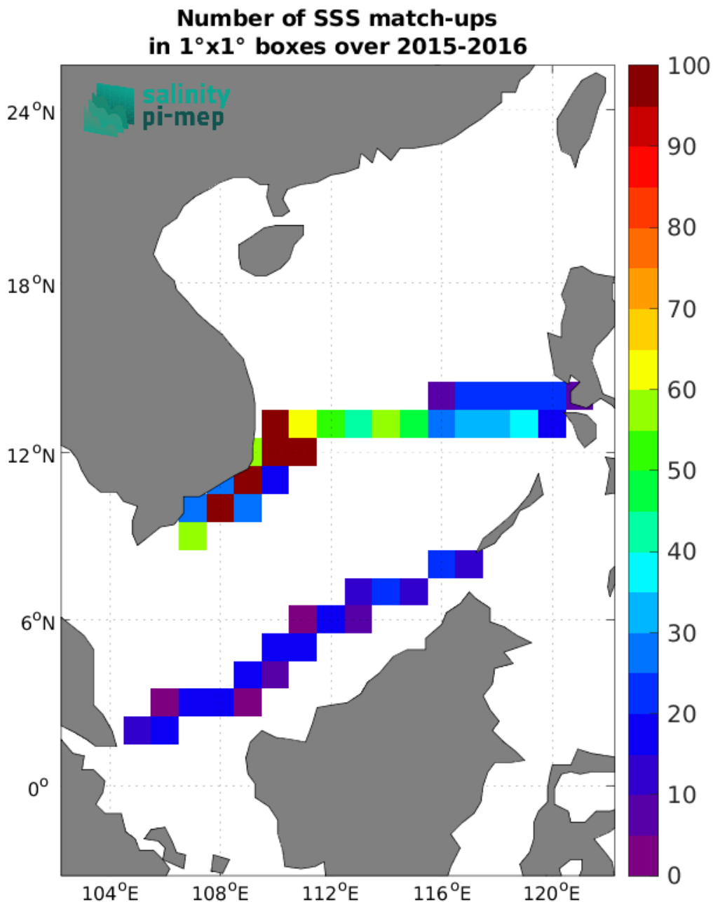
Figure 5: Number of SSS match-ups between TSG (SAMOS) SSS and the SMOS SSS L4 v1 - Daily (CMEMS-CNR) SSS product for the South China Sea Pi-MEP region over 1°x1° boxes and for the full satellite product period.
