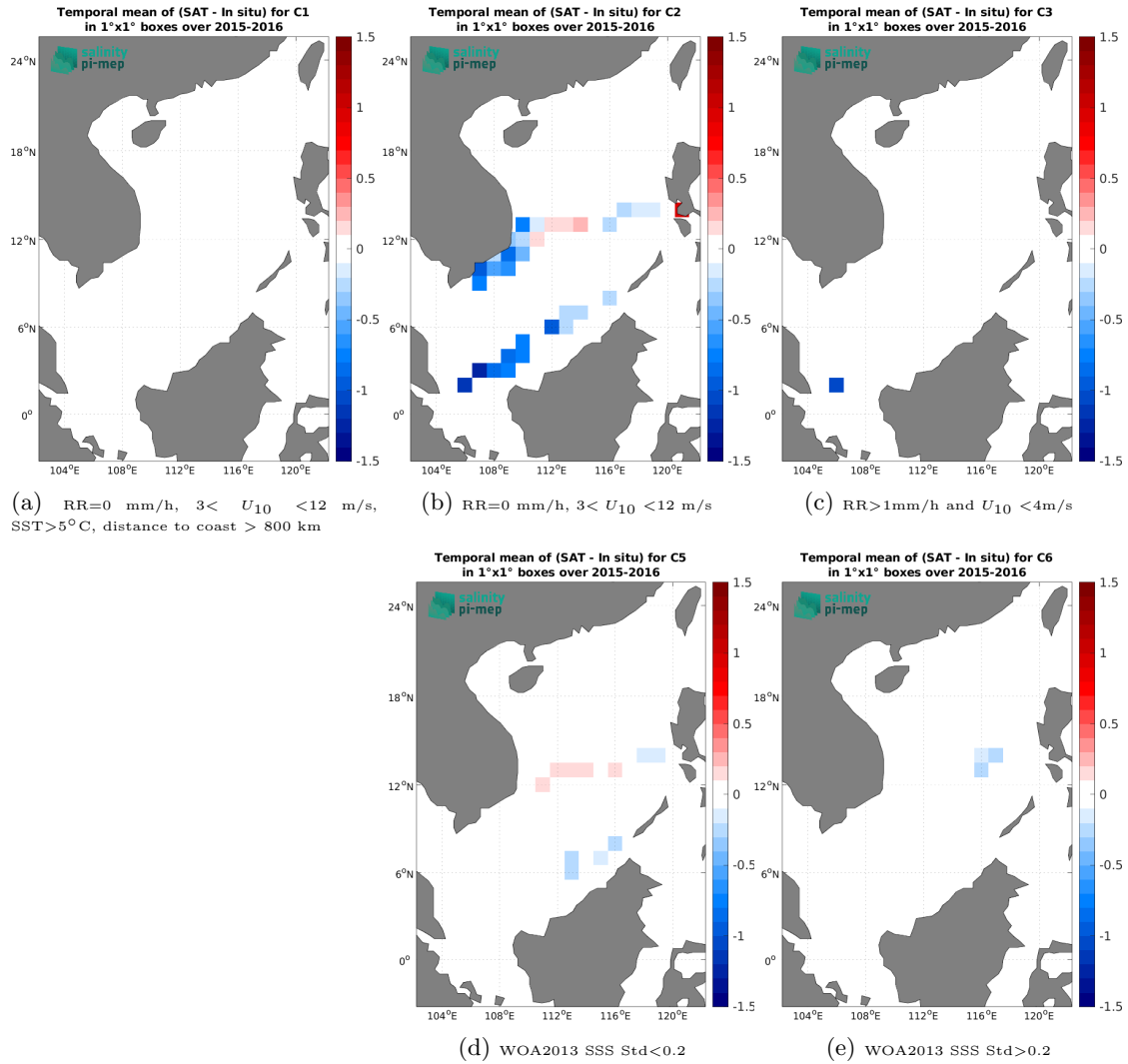
Figure 14: Temporal mean gridded over spatial boxes of size 1^{\circ} \times 1^{\circ} of \Delta SSS (SMOS SSS L4 v1 - Daily (CMEMS-CNR) - TSG (SAMOS)) for 5 different subdatasets corresponding to: RR=0 mm/h, 3 < U_{10} < 12 m/s, SST > 5^{\circ}C , distance to coast > 800 km (a), RR=0 mm/h, 3 < U_{10} < 12 m/s (b), RR > 1 mm/h and U_{10} < 4 m/s (c), WOA2013 SSS Std < 0.2 (d), WOA2013 SSS Std > 0.2 (e).
