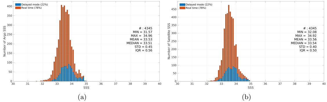
Figure 3: Histograms of SSS from Argo (a) and SMOS SSS L4 v1 - Daily (CMEMS-CNR) (b) considering all match-up pairs per bins of 0.1 over the South China Sea Pi-MEP region and for the full satellite product period.
