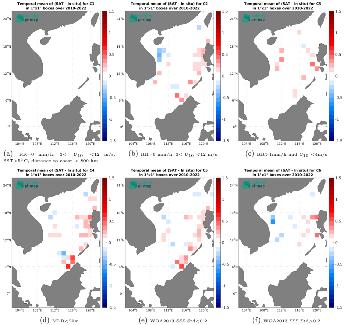
Figure 14: Temporal mean gridded over spatial boxes of size 1^\circ \times 1^\circ of \Delta\text{SSS} (SMOS SSS L4 v1 - Daily (CMEMS-CNR) - Argo) for 6 different subdatasets corresponding to: RR=0 mm/h, 3 < U_{10} < 12 m/s, SST > 5^\circ\text{C} , distance to coast > 800 km (a), RR=0 mm/h, 3 < U_{10} < 12 m/s (b), RR > 1 mm/h and U_{10} < 4 m/s (c), MLD < 20 m (d), WOA2013 SSS Std < 0.2 (e), WOA2013 SSS Std > 0.2 (f).
