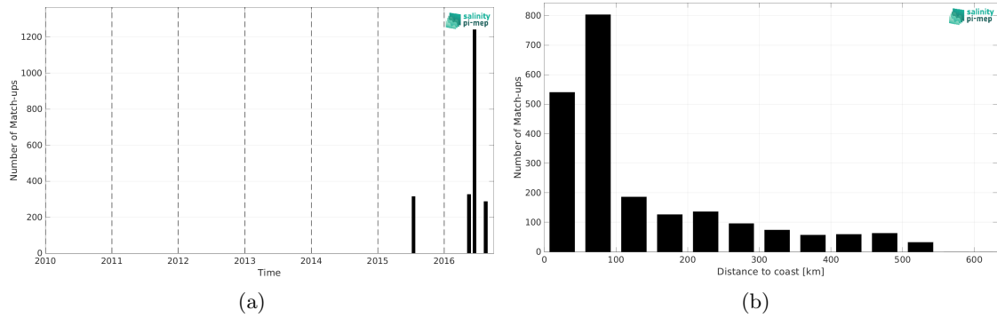
Figure 2: Number of match-ups between TSG (SAMOS) and SMOS SSS L4 OI v346 - Weekly (CMEMS-CATDS-LOPS) SSS as a function of time (a) and as function of the distance to coast (b) over the South China Sea Pi-MEP region and for the full satellite product period.
