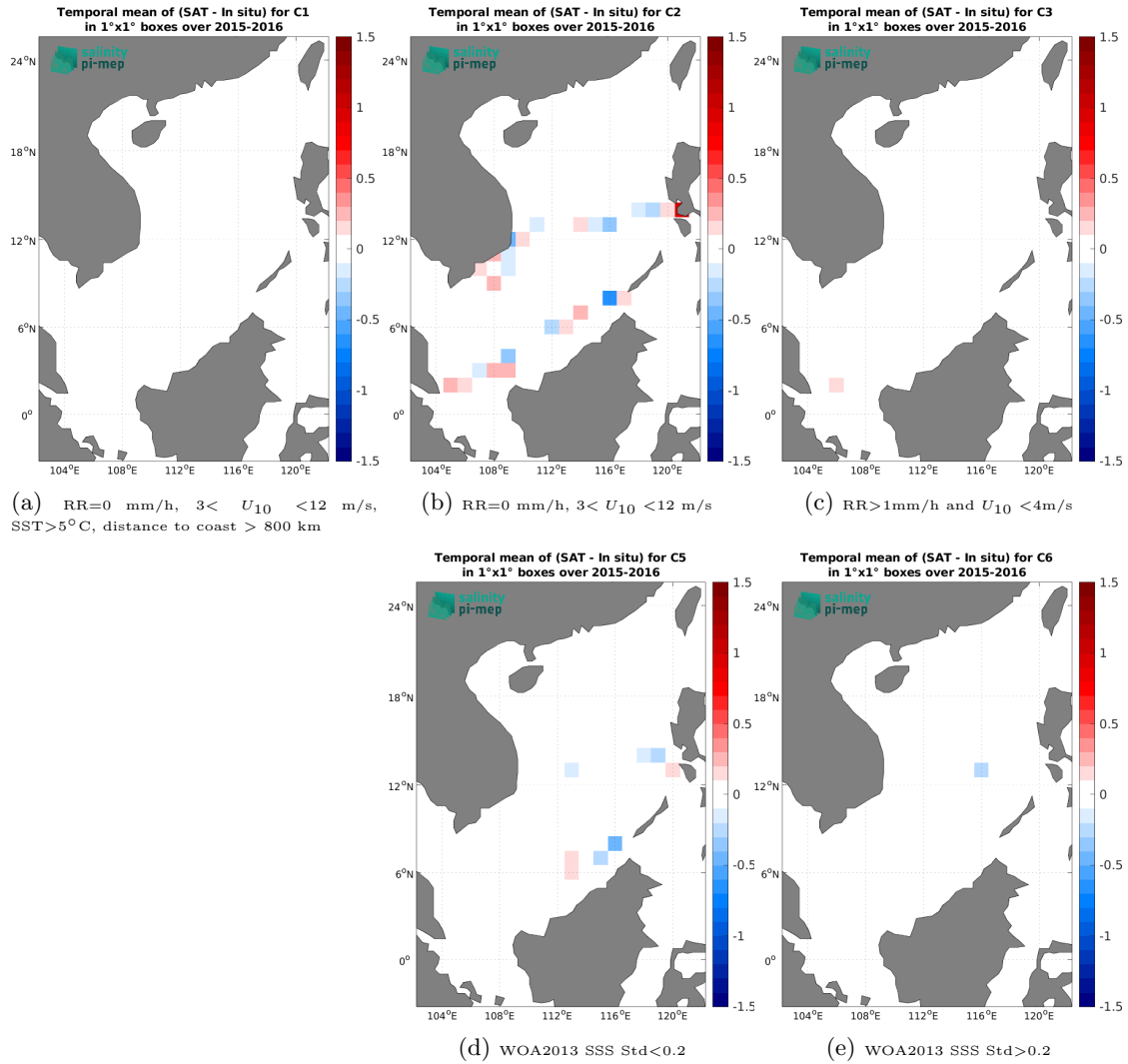
Figure 14: Temporal mean gridded over spatial boxes of size 1^\circ \times 1^\circ of \Delta SSS (SMOS SSS L4 OI v346 - Weekly (CMEMS-CATDS-LOPS) - TSG (SAMOS)) for 5 different subdatasets corresponding to: RR=0 mm/h, 3 < U_{10} < 12 m/s, SST>5°C, distance to coast > 800 km (a), RR=0 mm/h, 3 < U_{10} < 12 m/s (b), RR>1mm/h and U_{10} < 4 m/s (c), WOA2013 SSS Std<0.2 (d), WOA2013 SSS Std>0.2 (e).
