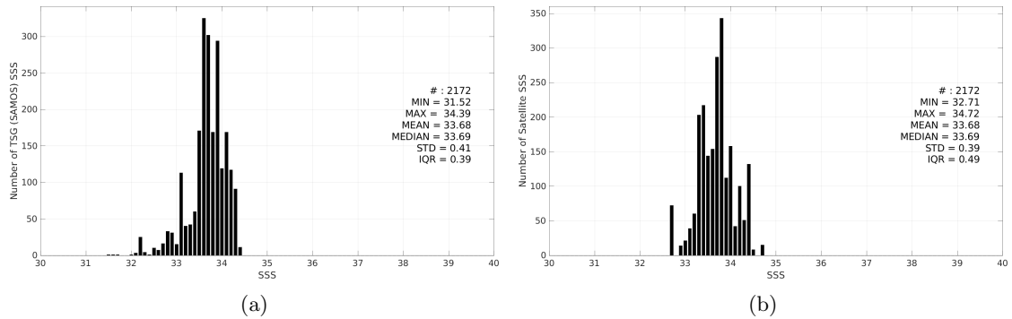
Figure 3: Histograms of SSS from TSG (SAMOS) (a) and SMOS SSS L4 OI v346 - Weekly (CMEMS-CATDS-LOPS) (b) considering all match-up pairs per bins of 0.1 over the South China Sea Pi-MEP region and for the full satellite product period.
