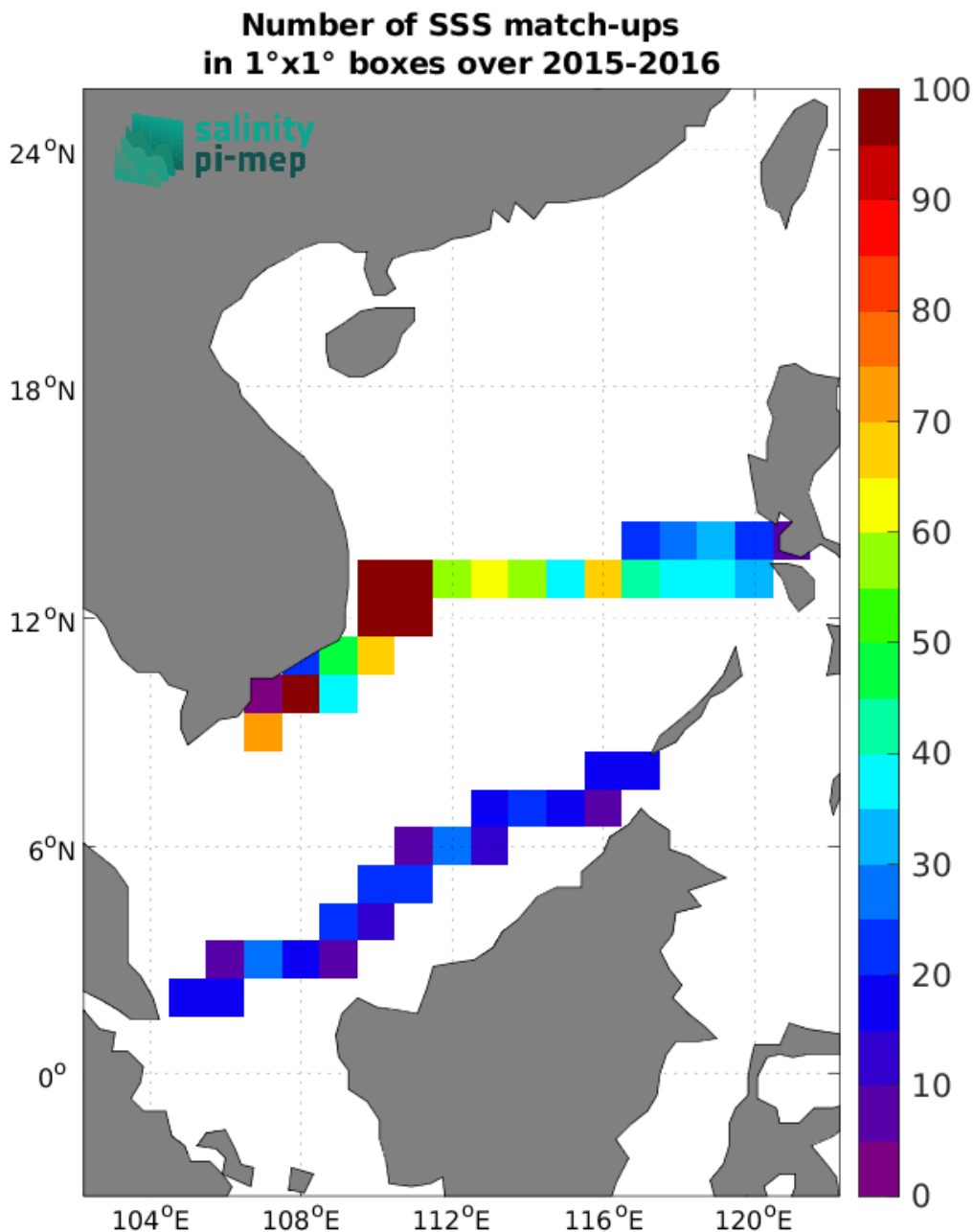
Figure 5: Number of SSS match-ups between TSG (SAMOS) SSS and the SMOS SSS L4 OI v346 - Weekly (CMEMS-CATDS-LOPS) SSS product for the South China Sea Pi-MEP region over 1°×1° boxes and for the full satellite product period.
