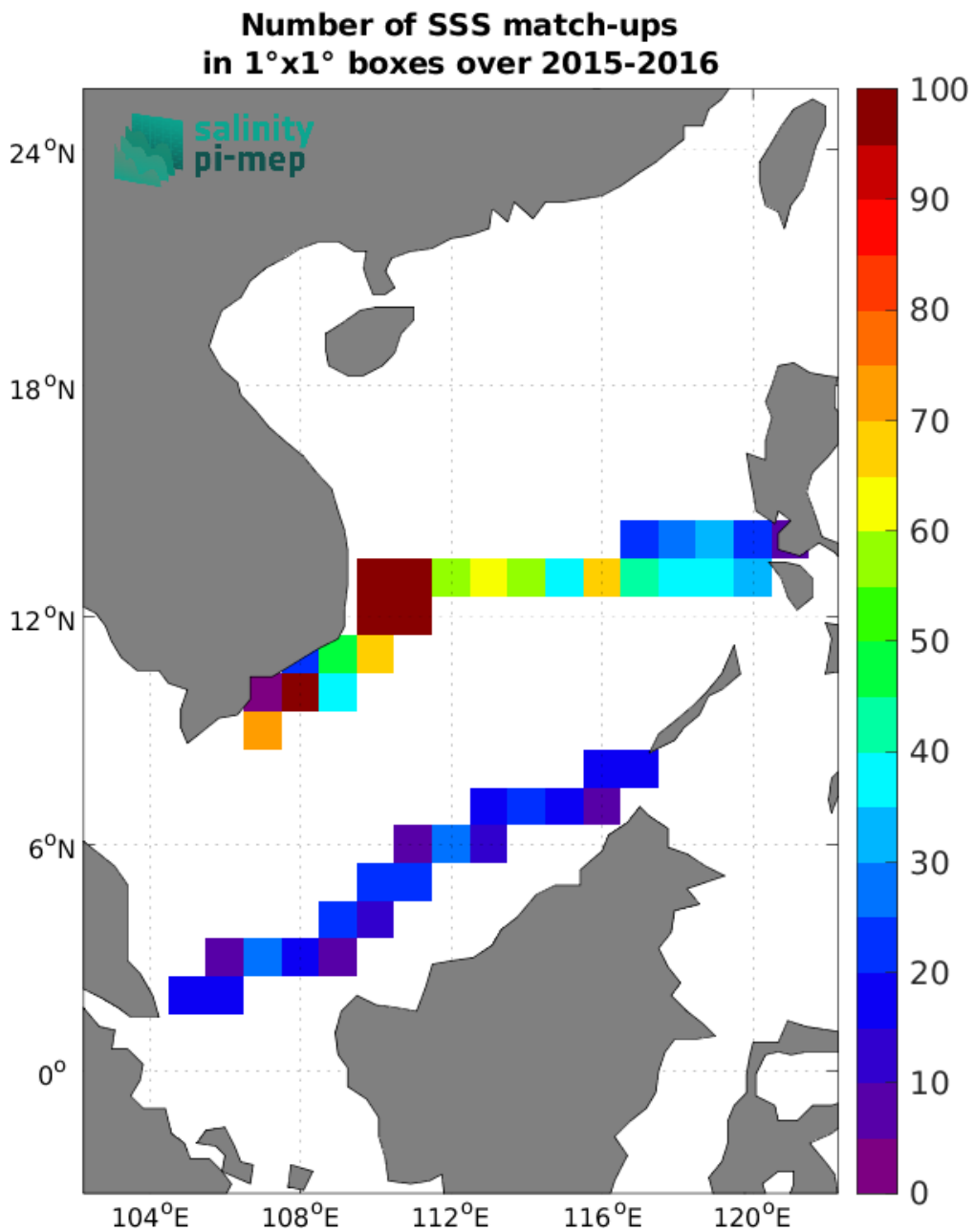
Figure 5: Number of SSS match-ups between TSG (SAMOS) SSS and the SMOS SSS L4 OI v346 - Weekly (CMEMS-CATDS-LOPS) SSS product for the South China Sea Pi-MEP region over 1^{\circ} \times 1^{\circ} boxes and for the full satellite product period.
