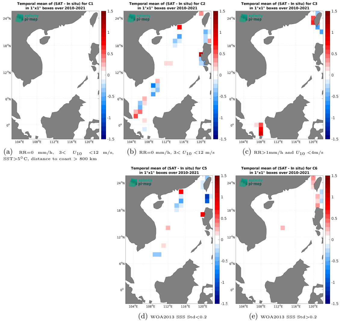
Figure 14: Temporal mean gridded over spatial boxes of size 1^\circ \times 1^\circ of \Delta\text{SSS} (SMOS SSS L4 OI v346 - Weekly (CMEMS-CATDS-LOPS) - TSG (LEGOS-DM)) for 5 different subdatasets corresponding to: RR=0 mm/h, 3 < U_{10} < 12 m/s, SST > 5^\circ\text{C} , distance to coast > 800 km (a), RR=0 mm/h, 3 < U_{10} < 12 m/s (b), RR > 1 mm/h and U_{10} < 4 m/s (c), WOA2013 SSS Std < 0.2 (d), WOA2013 SSS Std > 0.2 (e).
