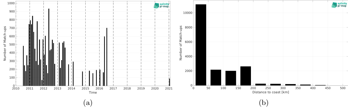
Figure 2: Number of match-ups between TSG (LEGOS-DM) and SMOS SSS L4 OI v346 - Weekly (CMEMS-CATDS-LOPS) SSS as a function of time (a) and as function of the distance to coast (b) over the South China Sea Pi-MEP region and for the full satellite product period.
