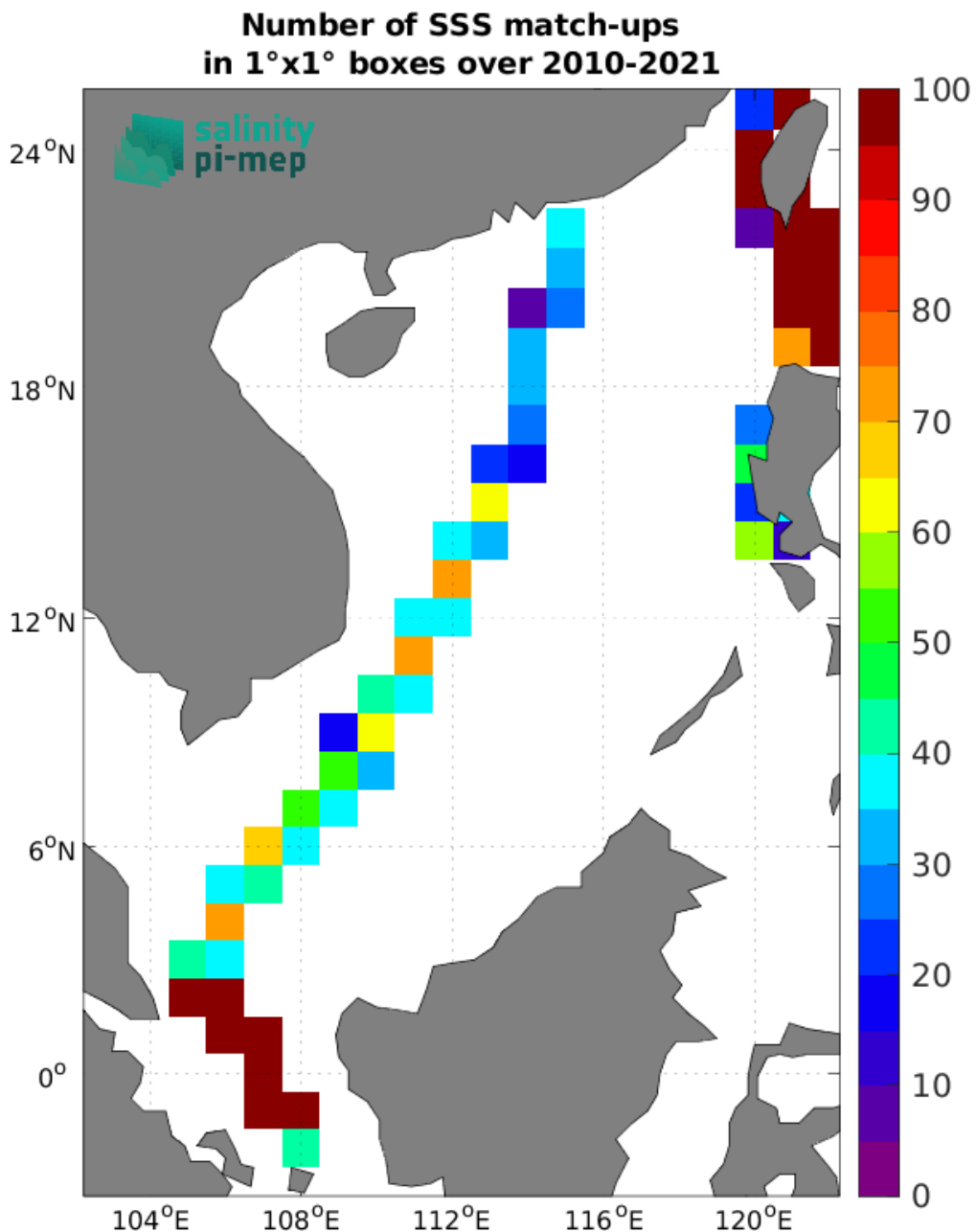
Figure 5: Number of SSS match-ups between TSG (LEGOS-DM) SSS and the SMOS SSS L4 OI v346 - Weekly (CMEMS-CATDS-LOPS) SSS product for the South China Sea Pi-MEP region over 1°×1° boxes and for the full satellite product period.
