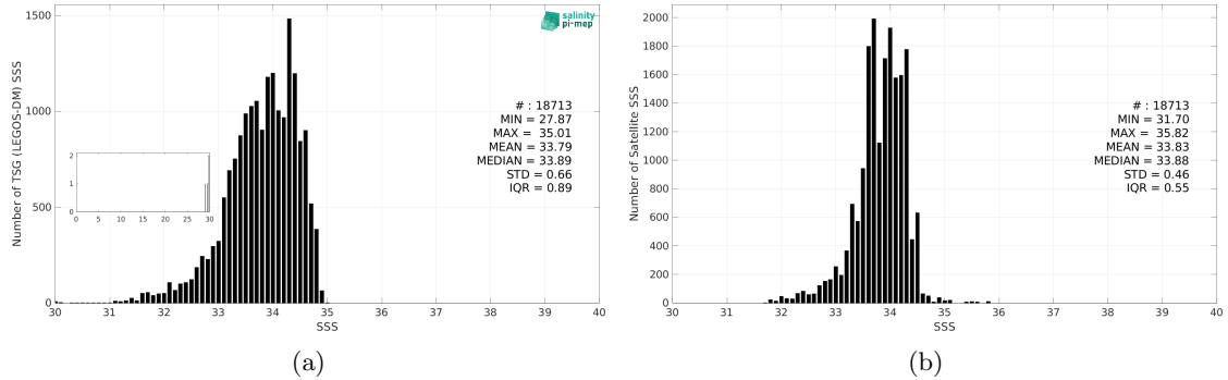
Figure 3: Histograms of SSS from TSG (LEGOS-DM) (a) and SMOS SSS L4 OI v346 - Weekly (CMEMS-CATDS-LOPS) (b) considering all match-up pairs per bins of 0.1 over the South China Sea Pi-MEP region and for the full satellite product period.
