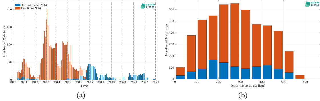
Figure 2: Number of match-ups between Argo and SMOS SSS L4 OI v346 - Weekly (CMEMS-CATDS-LOPS) SSS as a function of time (a) and as function of the distance to coast (b) over the South China Sea Pi-MEP region and for the full satellite product period.
