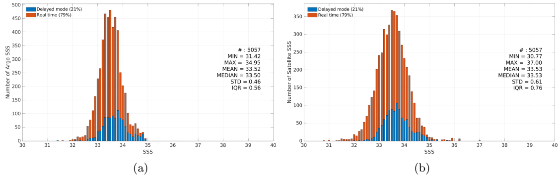
Figure 3: Histograms of SSS from Argo (a) and SMOS SSS L4 OI v346 - Weekly (CMEMS-CATDS-LOPS) (b) considering all match-up pairs per bins of 0.1 over the South China Sea Pi-MEP region and for the full satellite product period.
