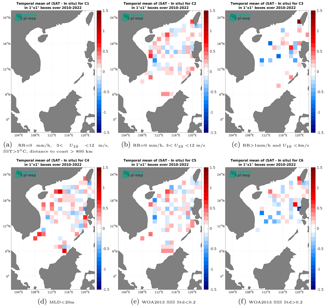
Figure 14: Temporal mean gridded over spatial boxes of size 1^\circ \times 1^\circ of \Delta SSS (SMOS SSS L4 OI v346 - Weekly (CMEMS-CATDS-LOPS) - Argo) for 6 different subdatasets corresponding to:RR=0 mm/h, 3 < U_{10} < 12 m/s, SST>5°C, distance to coast > 800 km (a), RR=0 mm/h, 3 < U_{10} < 12 m/s (b), RR>1mm/h and U_{10} < 4 m/s (c),MLD<20m (d),WOA2013 SSS Std<0.2 (e),WOA2013 SSS Std>0.2 (f).
