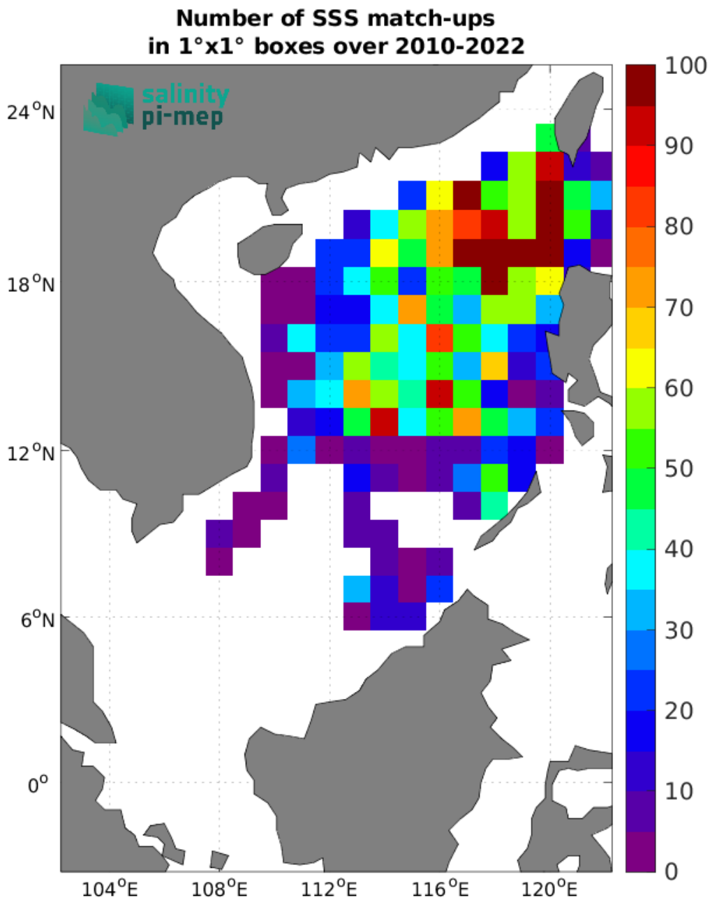
Figure 5: Number of SSS match-ups between Argo SSS and the SMOS SSS L4 OI v346 - Weekly (CMEMS-CATDS-LOPS) SSS product for the South China Sea Pi-MEP region over 1°×1° boxes and for the full satellite product period.
