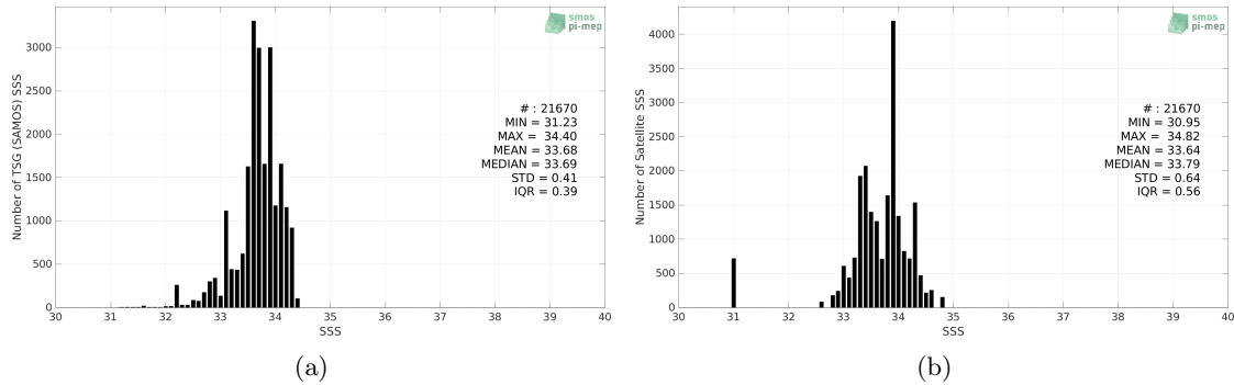
Figure 2: Histograms of SSS from TSG (SAMOS) (a) and SMOS SSS L4 OI v342 - Weekly (CMEMS-CATDS-LOPS) (b) considering all match-up pairs per bins of 0.1 over the South China Sea Pi-MEP region and for the full satellite product period.
