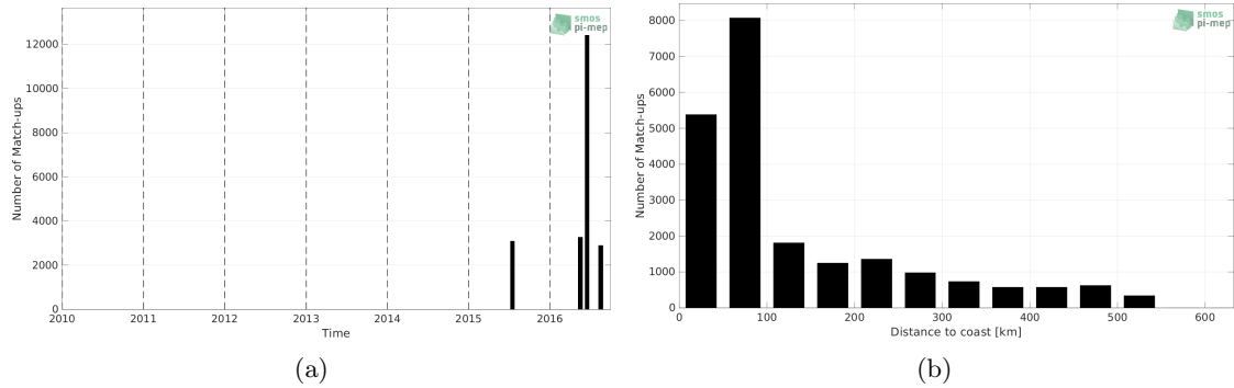
Figure 1: Number of match-ups between TSG (SAMOS) and SMOS SSS L4 OI v342 - Weekly (CMEMS-CATDS-LOPS) SSS as a function of time (a) and as function of the distance to coast (b) over the South China Sea Pi-MEP region and for the full satellite product period.
