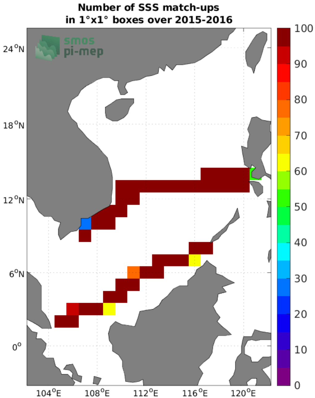
Figure 4: Number of SSS match-ups between TSG (SAMOS) SSS and the SMOS SSS L4 OI v342 - Weekly (CMEMS-CATDS-LOPS) SSS product for the South China Sea Pi-MEP region over 1^\circ \times 1^\circ boxes and for the full satellite product period.
