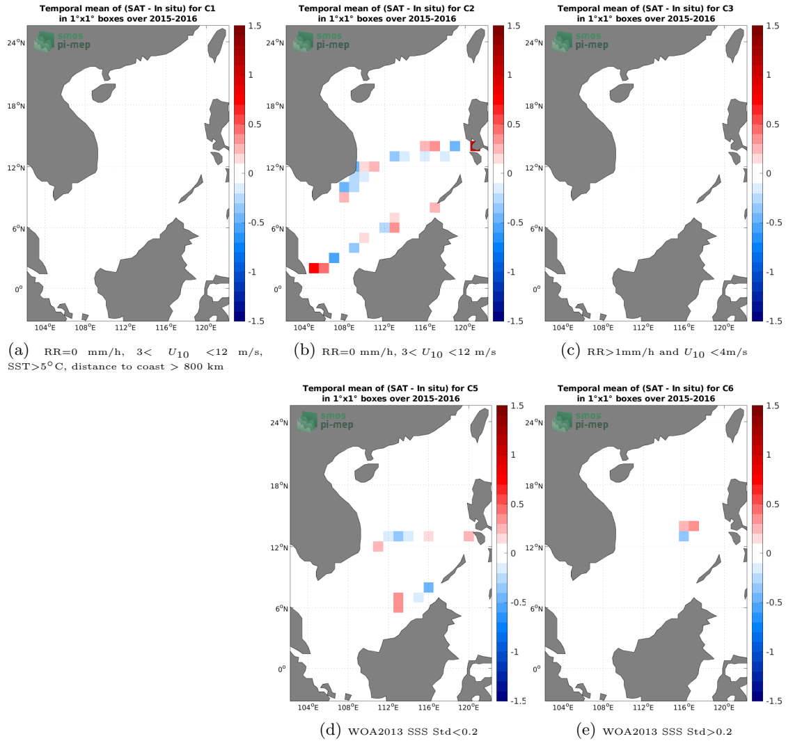
Figure 12: Temporal mean gridded over spatial boxes of size 1^\circ \times 1^\circ of \Delta SSS (SMOS SSS L4 OI v342 - Weekly (CMEMS-CATDS-LOPS) - TSG (SAMOS)) for 5 different subdatasets corresponding to:RR=0 mm/h, 3 < U_{10} < 12 m/s, SST>5°C, distance to coast > 800 km (a), RR=0 mm/h, 3 < U_{10} < 12 m/s (b), RR>1mm/h and U_{10} < 4 m/s (c), WOA2013 SSS Std<0.2 (d), WOA2013 SSS Std>0.2 (e).
