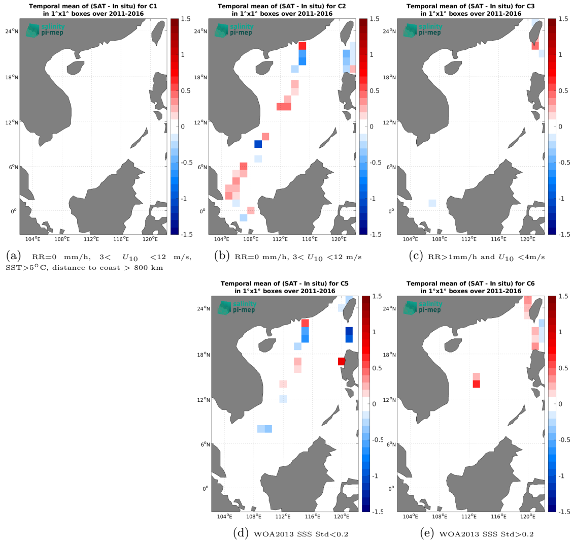
Figure 12: Temporal mean gridded over spatial boxes of size 1^\circ \times 1^\circ of \Delta\text{SSS} (SMOS SSS L4 OI v342 - Weekly (CMEMS-CATDS-LOPS) - TSG (LEGOS-DM)) for 5 different subdatasets corresponding to: RR=0 mm/h, 3 < U_{10} < 12 m/s, SST > 5^\circ\text{C} , distance to coast > 800 km (a), RR=0 mm/h, 3 < U_{10} < 12 m/s (b), RR > 1 mm/h and U_{10} < 4 m/s (c), WOA2013 SSS Std < 0.2 (d), WOA2013 SSS Std > 0.2 (e).
