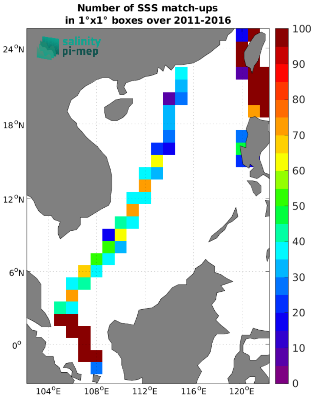
Figure 4: Number of SSS match-ups between TSG (LEGOS-DM) SSS and the SMOS SSS L4 OI v342 - Weekly (CMEMS-CATDS-LOPS) SSS product for the South China Sea Pi-MEP region over 1^{\circ} \times 1^{\circ} boxes and for the full satellite product period.
