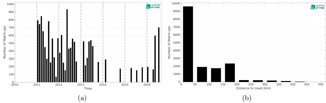
Figure 1: Number of match-ups between TSG (LEGOS-DM) and SMOS SSS L4 OI v342 - Weekly (CMEMS-CATDS-LOPS) SSS as a function of time (a) and as function of the distance to coast (b) over the South China Sea Pi-MEP region and for the full satellite product period.
