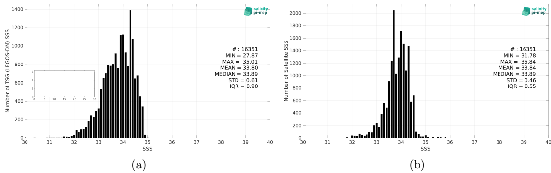
Figure 2: Histograms of SSS from TSG (LEGOS-DM) (a) and SMOS SSS L4 OI v342 - Weekly (CMEMS-CATDS-LOPS) (b) considering all match-up pairs per bins of 0.1 over the South China Sea Pi-MEP region and for the full satellite product period.
