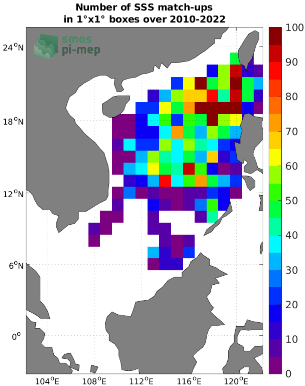
Figure 4: Number of SSS match-ups between Argo SSS and the SMOS SSS L4 OI v342 - Weekly (CMEMS-CATDS-LOPS) SSS product for the South China Sea Pi-MEP region over 1°x1° boxes and for the full satellite product period.
