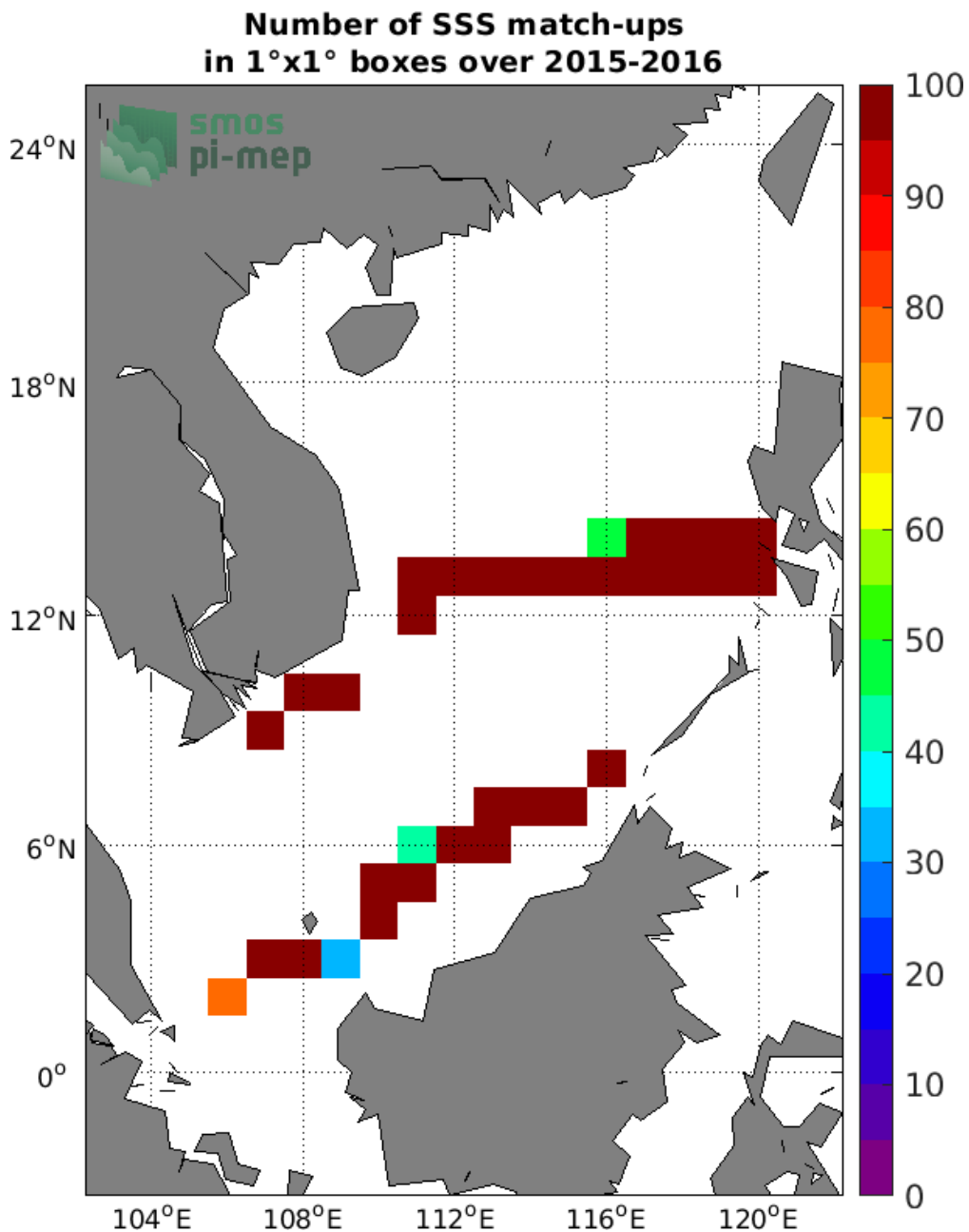
Figure 4: Number of SSS match-ups between TSG (SAMOS) SSS and the SMOS L4 v2 Weekly (CATDS-CECOS-IFREMER) SSS product for the South China Sea Pi-MEP region over 1°x1° boxes and for the full satellite product period.
