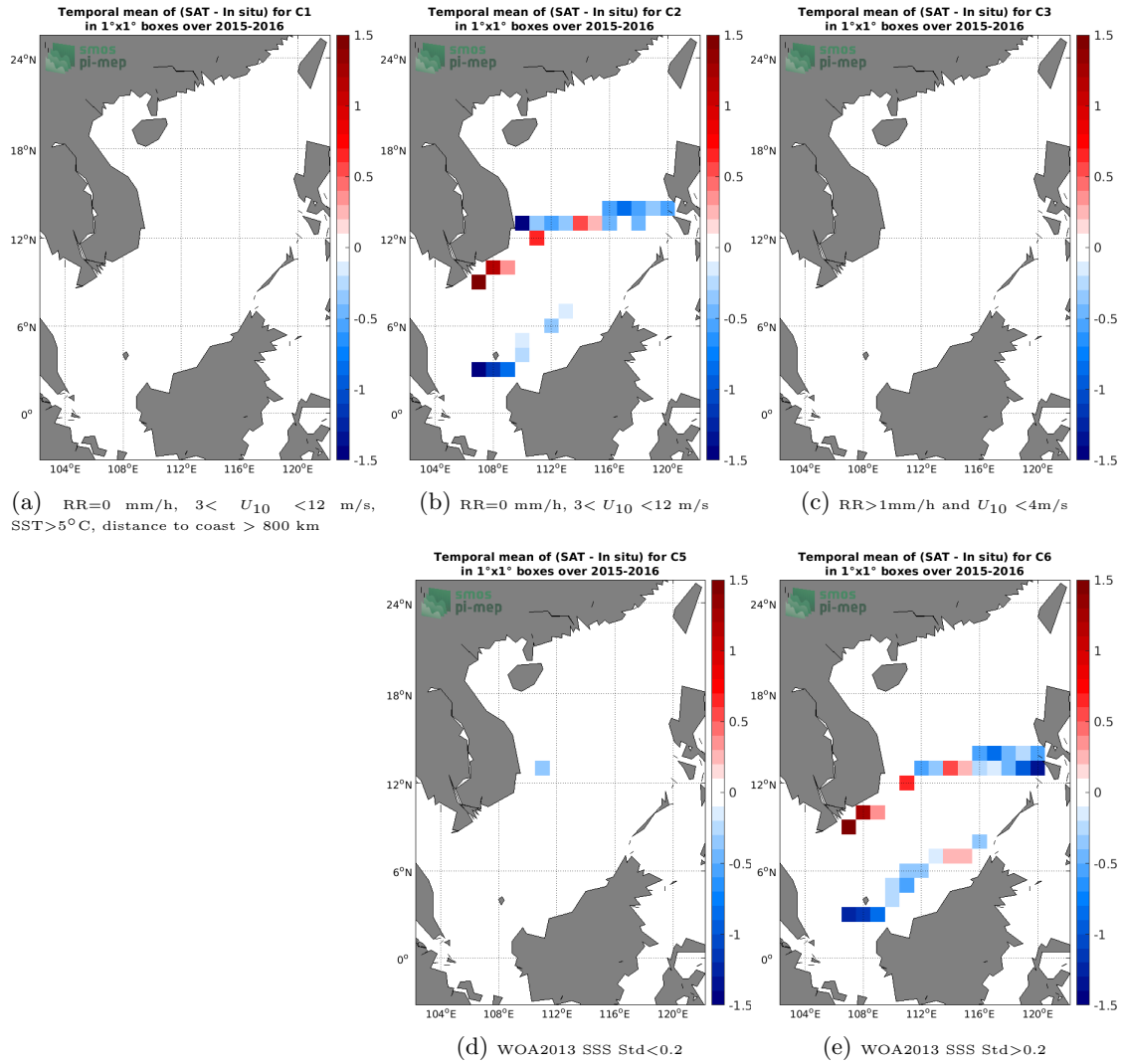
Figure 12: Temporal mean gridded over spatial boxes of size 1°x1° of \Delta SSS (SMOS L4 v2 Weekly (CATDS-CECOS-IFREMER) - TSG (SAMOS)) for 5 different subdatasets corresponding to: RR=0 mm/h, 3 < U_{10} < 12 m/s, SST > 5°C, distance to coast > 800 km (a), RR=0 mm/h, 3 < U_{10} < 12 m/s (b), RR > 1mm/h and U_{10} < 4 m/s (c), WOA2013 SSS Std < 0.2 (d), WOA2013 SSS Std > 0.2 (e).
