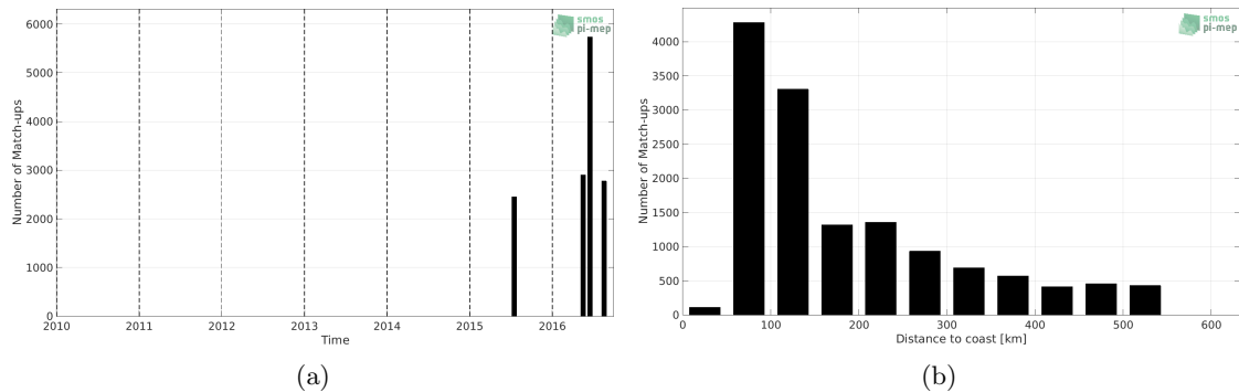
Figure 1: Number of match-ups between TSG (SAMOS) and SMOS L4 v2 Weekly (CATDS-CECOS-IFREMER) SSS as a function of time (a) and as function of the distance to coast (b) over the South China Sea Pi-MEP region and for the full satellite product period.
