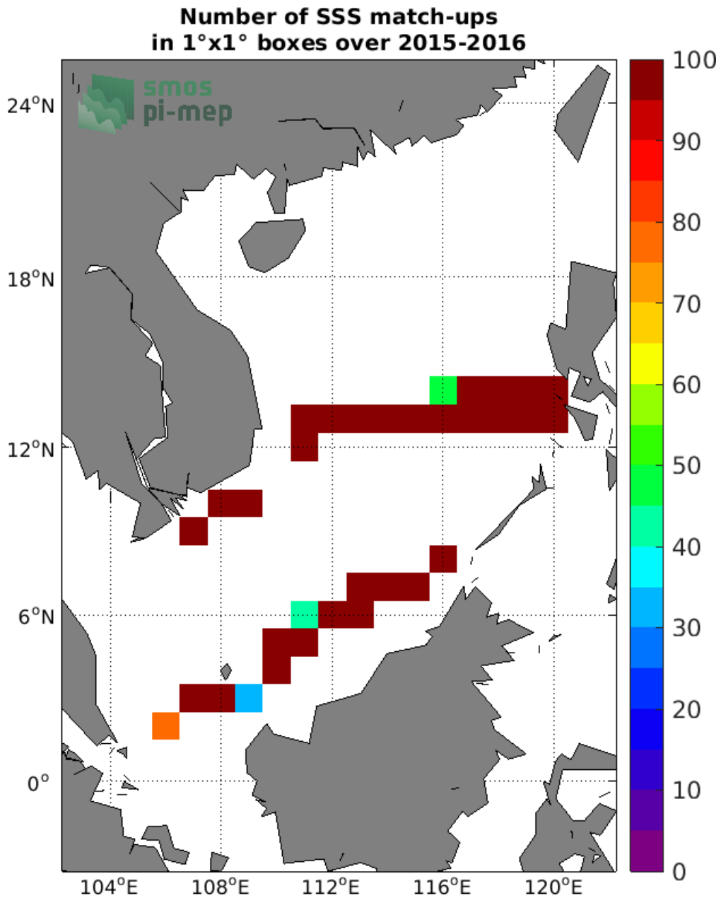
Figure 4: Number of SSS match-ups between TSG (SAMOS) SSS and the SMOS L4 v2 Weekly (CATDS-CECOS-IFREMER) SSS product for the South China Sea Pi-MEP region over 1°x1° boxes and for the full satellite product period.
