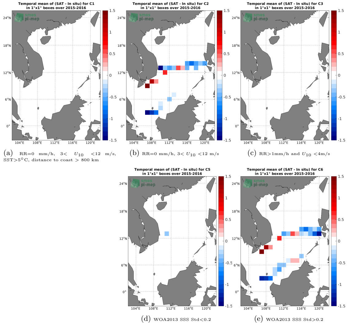
Figure 12: Temporal mean gridded over spatial boxes of size 1°x1° of \Delta SSS (SMOS L4 v2 Weekly (CATDS-CECOS-IFREMER) - TSG (SAMOS)) for 5 different subdatasets corresponding to:RR=0 mm/h, 3 < U_{10} < 12 m/s, SST>5°C, distance to coast > 800 km (a), RR=0 mm/h, 3 < U_{10} < 12 m/s (b), RR>1mm/h and U_{10} < 4 m/s (c), WOA2013 SSS Std<0.2 (d), WOA2013 SSS Std>0.2 (e).
