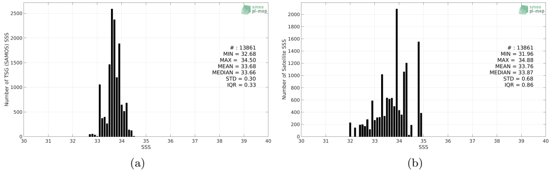
Figure 2: Histograms of SSS from TSG (SAMOS) (a) and SMOS L4 v2 Weekly (CATDS-CECOS-IFREMER) (b) considering all match-up pairs per bins of 0.1 over the South China Sea Pi-MEP region and for the full satellite product period.
