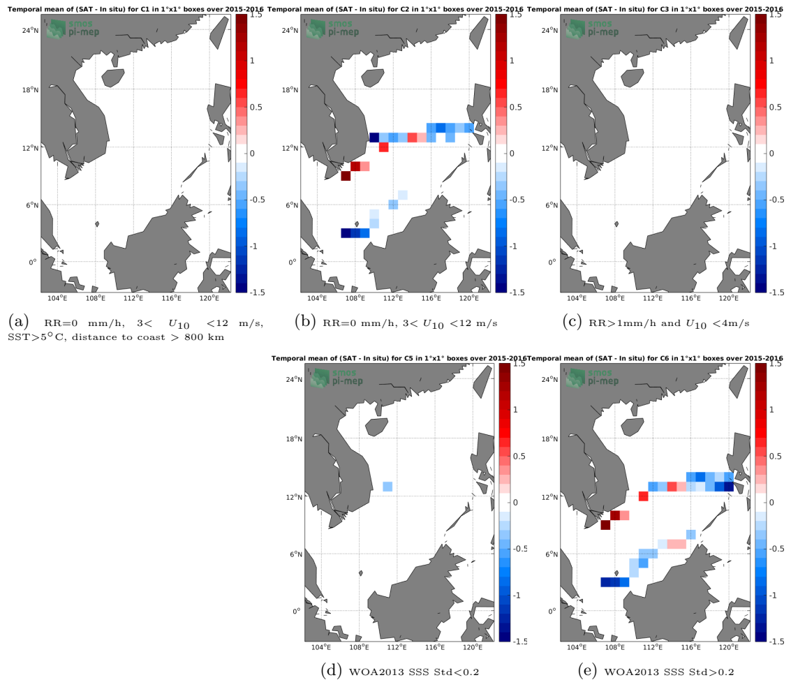
Figure 12: Temporal mean gridded over spatial boxes of size 1^\circ \times 1^\circ of \Delta SSS (SMOS-L4-CATDS-CECOS-IFREMER-V2-WEEKLY-0.5DEG - TSG-SAMOS) for 5 different subdatasets corresponding to:RR=0 mm/h, 3 < U_{10} < 12 m/s, SST > 5^\circ\text{C} , distance to coast > 800 km (a), RR=0 mm/h, 3 < U_{10} < 12 m/s (b), RR > 1 mm/h and U_{10} < 4 m/s (c), WOA2013 SSS Std < 0.2 (d), WOA2013 SSS Std > 0.2 (e).
