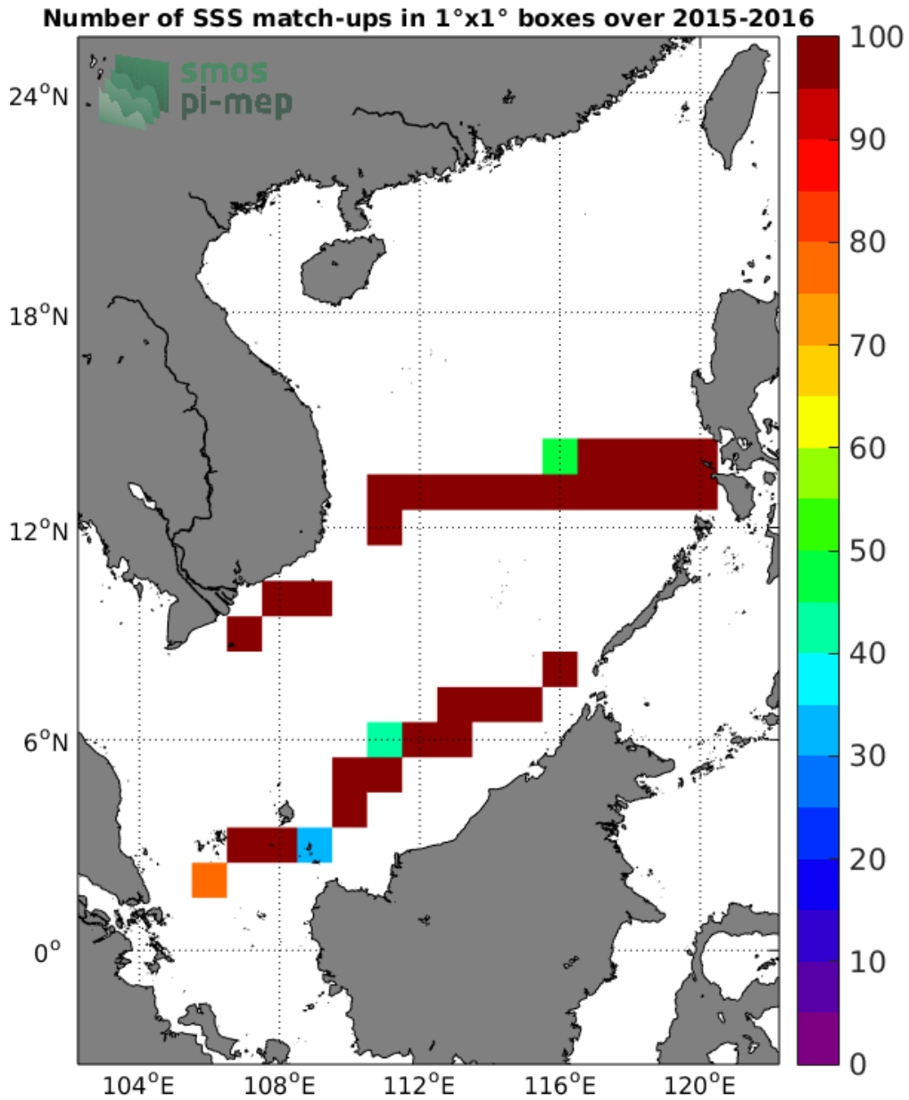
Figure 4: Number of SSS match-ups between TSG-SAMOS SSS and the SMOS-L4-CATDS-CECOS-IFREMER-V2-WEEKLY-0.5DEG SSS product for the South China Sea Pi-MEP region over 1°x1° boxes and for the full satellite product period.
