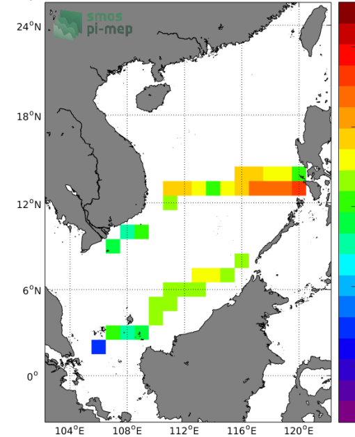
(c) MEAN(TSG-SAMOS SSS)
