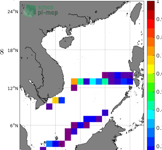
Temporal STD of (Sat-TSG-SAMOS) in 1°x1° boxes over 2015-2016
