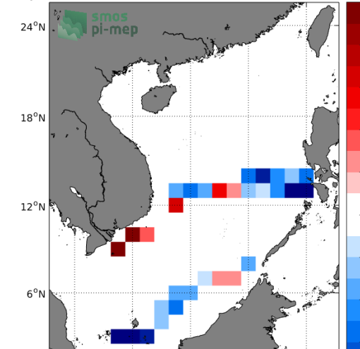
Temporal mean of (Sat-TSG-SAMOS) in 1°x1° boxes over 2015-2016
