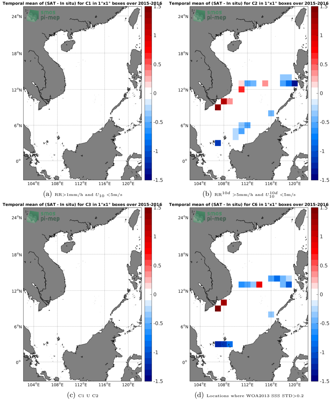
Figure 12: Temporal mean gridded over spatial boxes of size 1°x1° of \Delta\text{SSS} (SMOS-L4-CATDS-CECOS-IFREMER-V2-WEEKLY-0.5DEG - TSG-SAMOS) for 4 different subdatasets corresponding to: RR > 1\text{mm/h} and U_{10} < 5\text{m/s} (a), RR^{10d} > 5\text{mm/h} and U_{10}^{10d} < 5\text{m/s} (b), C1 U C2 (c), Locations where WOA2013 SSS STD > 0.2 (d).
