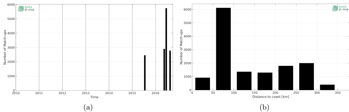
Figure 1: Number of match-ups between TSG-SAMOS and SMOS-L4-CATDS-CECOS-IFREMER-V2-WEEKLY-0.5DEG SSS as a function of time (a) and as function of the distance to coast (b) over the South China Sea Pi-MEP region and for the full satellite product period.
