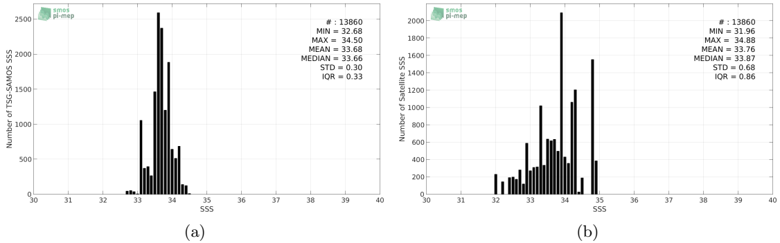
Figure 2: Histograms of SSS from TSG-SAMOS (a) and SMOS-L4-CATDS-CECOS-IFREMER-V2-WEEKLY-0.5DEG (b) considering all match-up pairs per bins of 0.1 over the South China Sea Pi-MEP region and for the full satellite product period.
