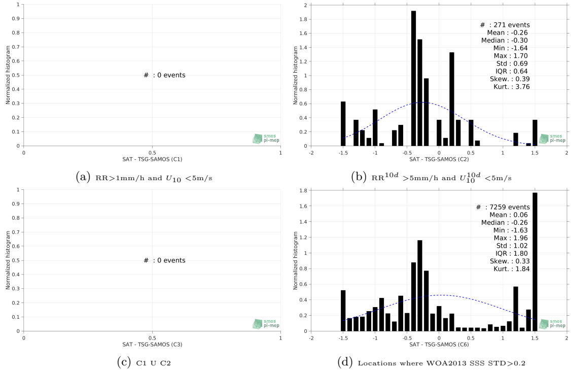
Figure 13: Normalized histogram of \Delta\text{SSS} (SMOS-L4-CATDS-CECOS-IFREMER-V2-WEEKLY-0.5DEG - TSG-SAMOS) for 6 different subdatasets corresponding to: RR > 1\text{mm/h} and U_{10} < 5\text{m/s} (a), RR^{10d} > 5\text{mm/h} and U_{10}^{10d} < 5\text{m/s} (b), C1 \cup C2 (c), Locations where WOA2013 SSS STD > 0.2 (d).
