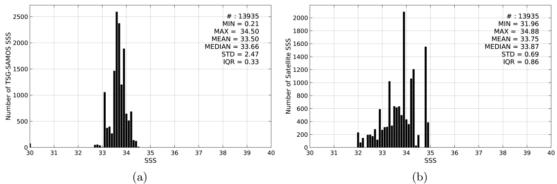
Figure 2: Histograms of SSS from TSG-SAMOS (a) and SMOS-L4-CATDS-CECOS-IFREMER-V2-WEEKLY-0.5DEG (b) considering all match-up pairs per bins of 0.1 over the South China Sea Pi-MEP region and for the full satellite product period.
