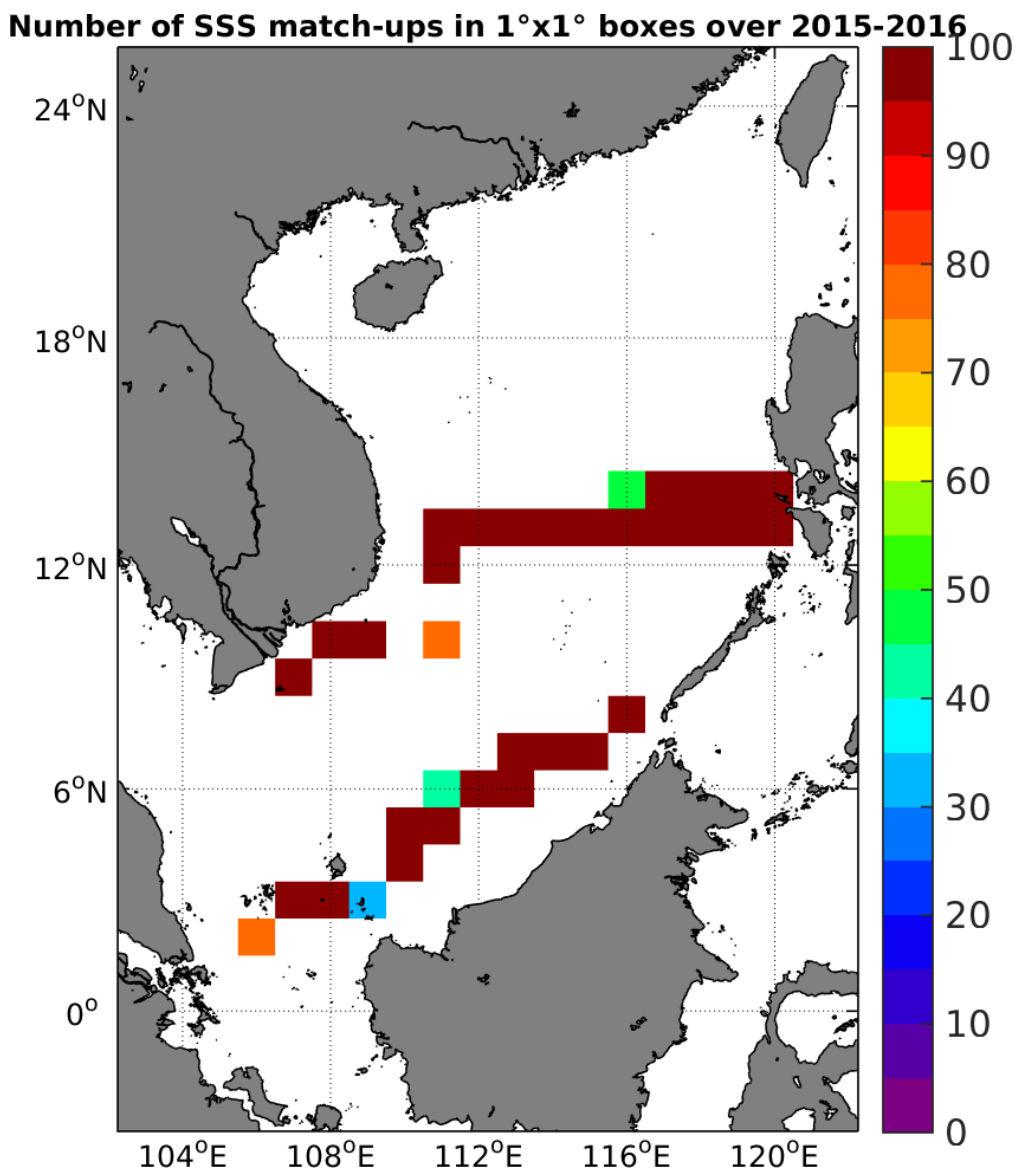
Figure 4: Number of SSS match-ups between TSG-SAMOS SSS and the SMOS-L4-CATDS-CECOS-IFREMER-V2-WEEKLY-0.5DEG SSS product for the South China Sea Pi-MEP region over 1°x1° boxes and for the full satellite product period.
