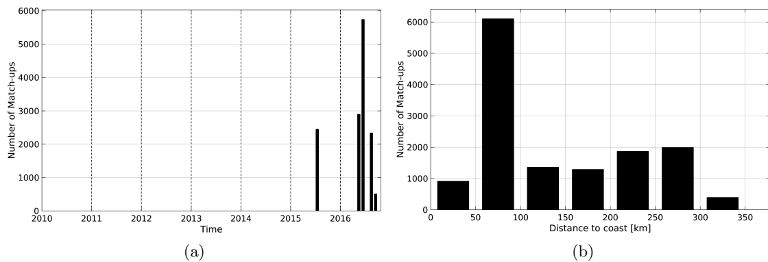
Figure 1: Number of match-ups between TSG-SAMOS and SMOS-L4-CATDS-CECOS-IFREMER-V2-WEEKLY-0.5DEG SSS as a function of time (a) and as function of the distance to coast (b) over the South China Sea Pi-MEP region and for the full satellite product period.
