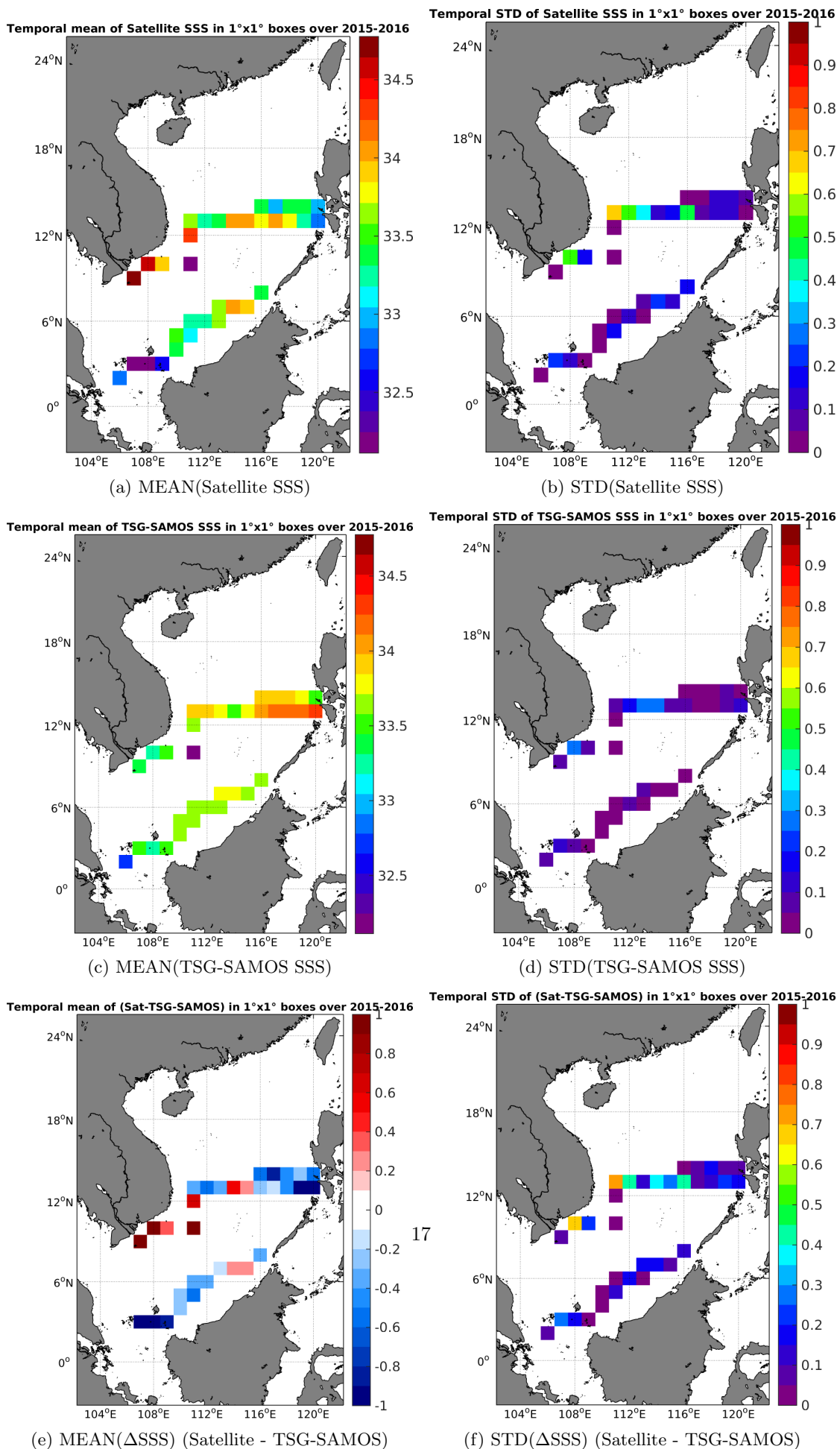
Figure 6: Temporal mean (left) and STD (right) of SSS from SMOS-L4-CATDS-CECOS-
