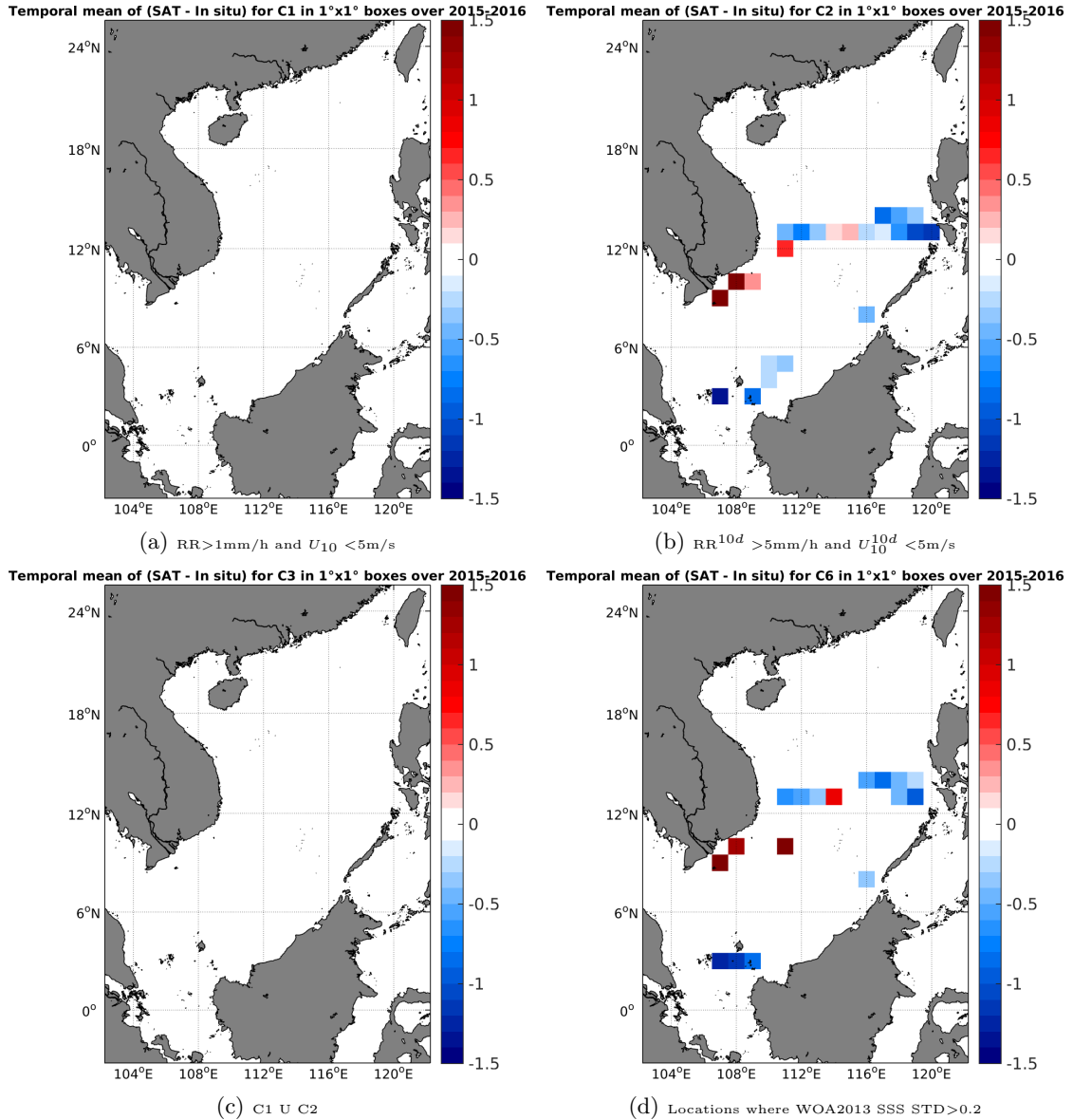
Figure 12: Temporal mean gridded over spatial boxes of size 1°x1° of ΔSSS (SMOS-L4-CATDS-CECOS-IFREMER-V2-WEEKLY-0.5DEG - TSG-SAMOS) for 4 different subdatasets corresponding to:RR>1mm/h and U_{10} < 5\text{m/s} (a), RR^{10d} > 5\text{mm/h} and U_{10}^{10d} < 5\text{m/s} (b), C1 U C2 (c),Locations where WOA2013 SSS STD>0.2 (d).
